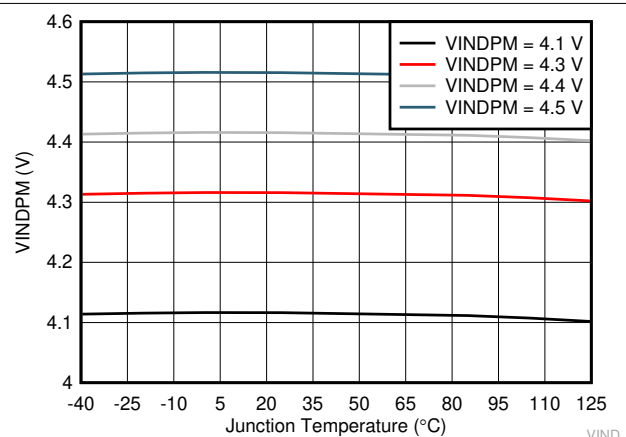
8-6. VINDPM vs Junction Temperature
