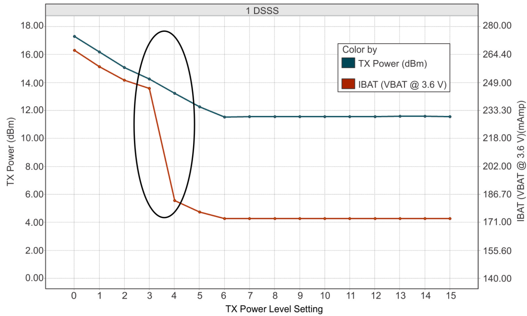
FIG 8-1. TX Power and IBAT vs TX Power Level Settings (1 DSSS)
