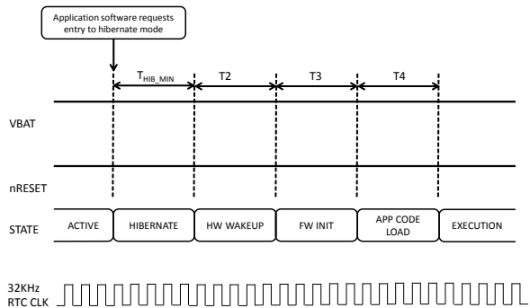
Figure 8-7. Wake Up From Hibernate Timing Diagram
