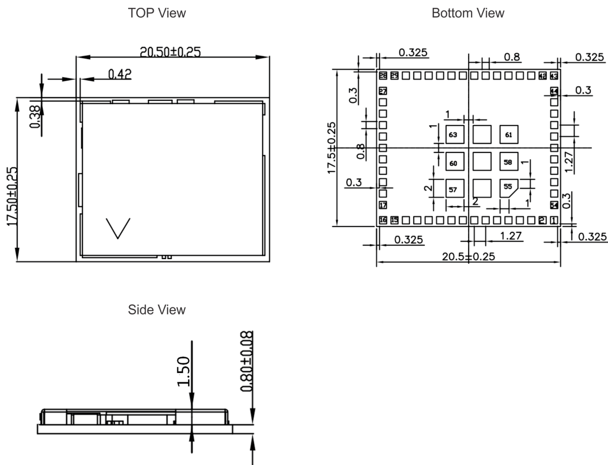
✕ 13-1. Mechanical Drawing
