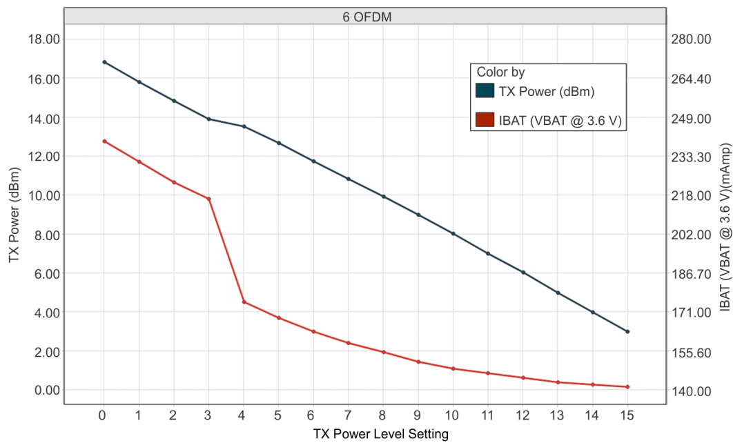
FIG 8-2. TX Power and IBAT vs TX Power Level Settings (6 OFDM)
