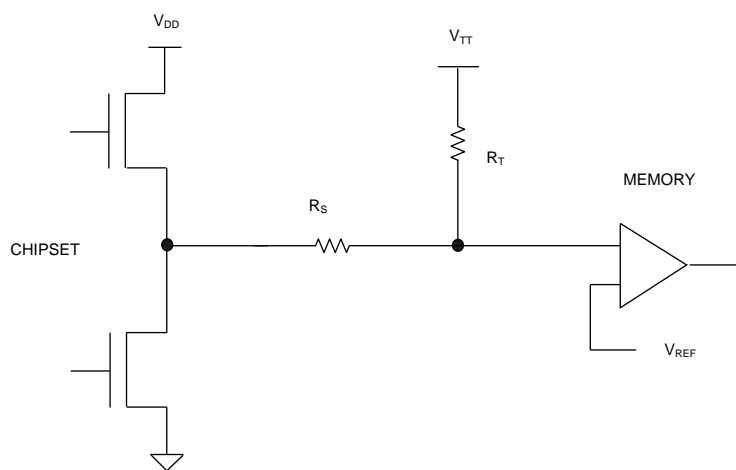
Figure 17. SSTL-Termination Scheme
