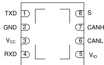
图 5-4. DRB Package for (V), (GV), (HV) and (HGV) Devices 8 PIN (VSON) Top View
