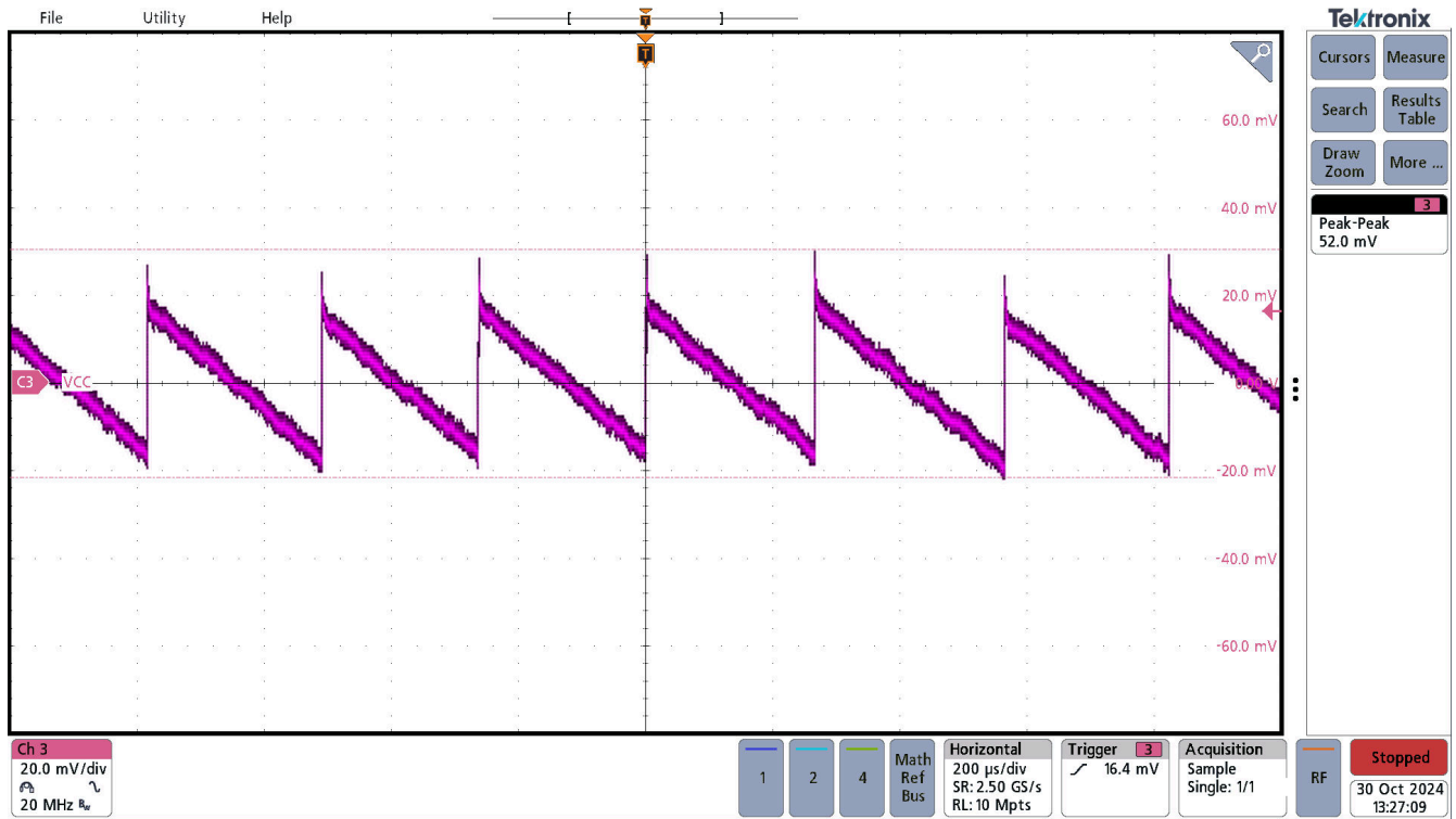
Figure 3-13. UCC33421-Q1 VCC AC Ripple, VINP=5.0V, VCC=5.0V, I out =0mA
