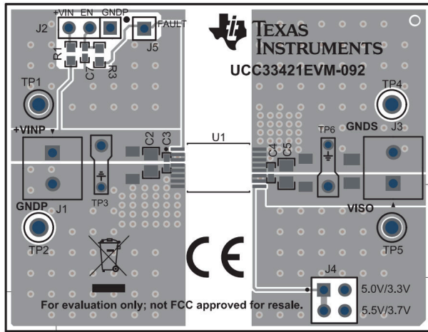
Figure 4-4. PCB Top Layer, Assembly
