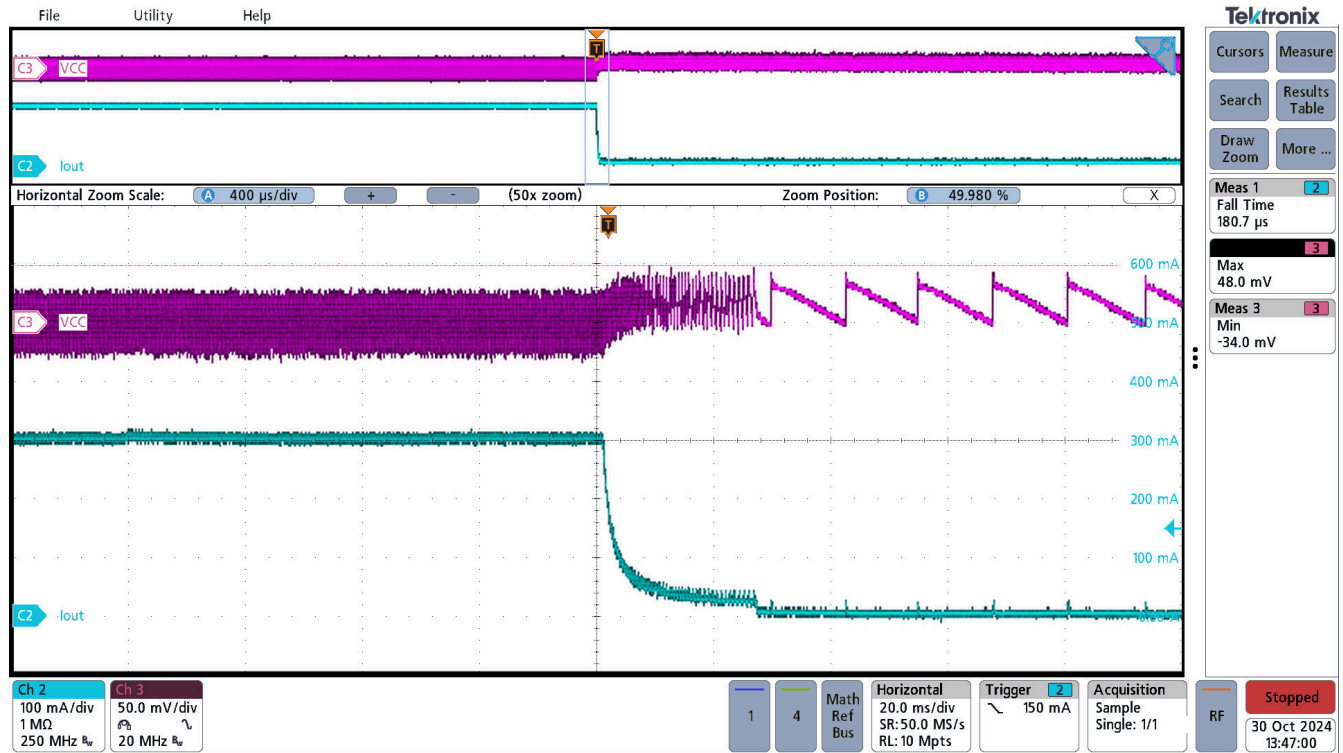
Figure 3-19. UCC33421-Q1 Load transient, VINP=5.0V, VCC=5.0V, Full load ( I_{out}=300\text{mA} ) to No load ( I_{out}=0\text{mA} )
