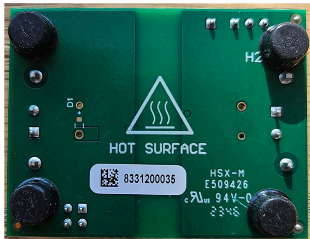
UCC33421EVM-092 (Bottom View)
