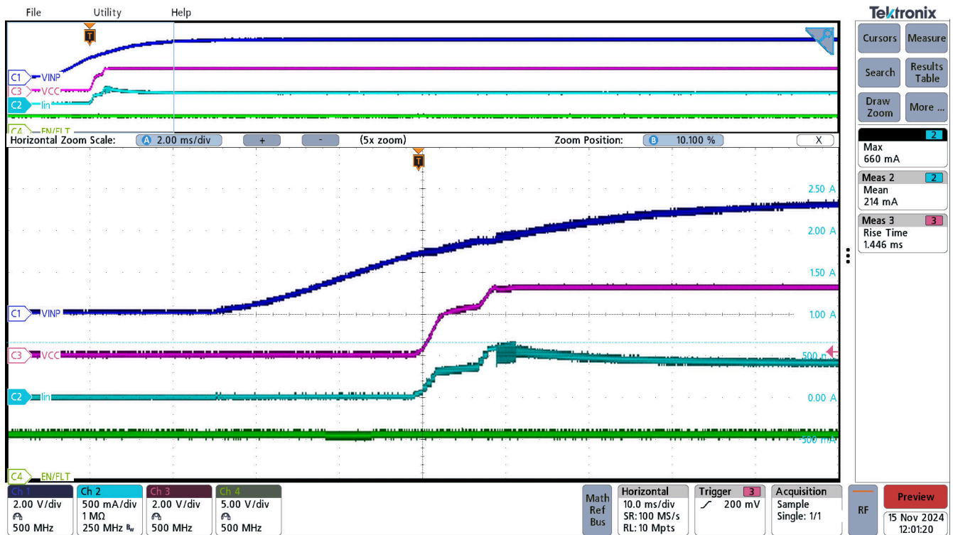
Figure 3-8. UCC33411-Q1 Start-up, sequence EN=5.0V → VINP=5.0V, VCC=3.3V, Rload=10Ω
