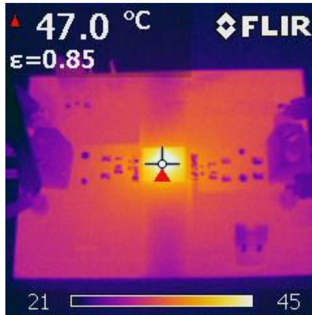
Figure 3-25. UCC33421-Q1 VINP=5.0V, VCC=5.0V, I out =150 mA, P out =0.75W, TA=25°C
