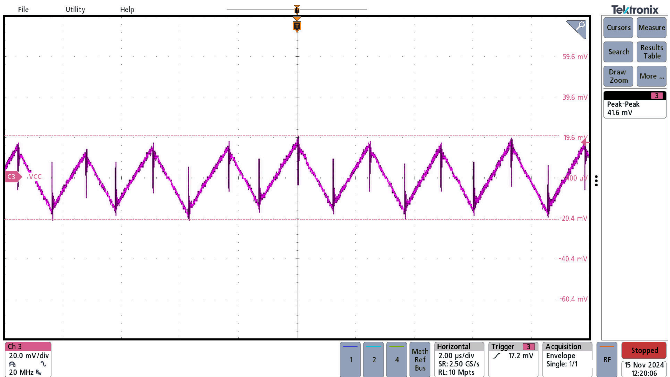
Figure 3-16. UCC33411-Q1 VCC AC Ripple, VINP=5.0V, VCC=3.3V, I out =300mA
