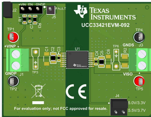
Figure 4-2. Fully Assembled 3D Top View
