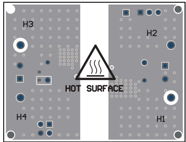
Figure 4-7. PCB Bottom Layer, Assembly (Mirrored View)
