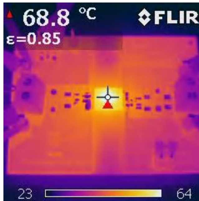
Figure 3-24. UCC33411-Q1 VINP=5.0V, VCC=3.3V, I out =300mA, P out =1W, TA=25°C
