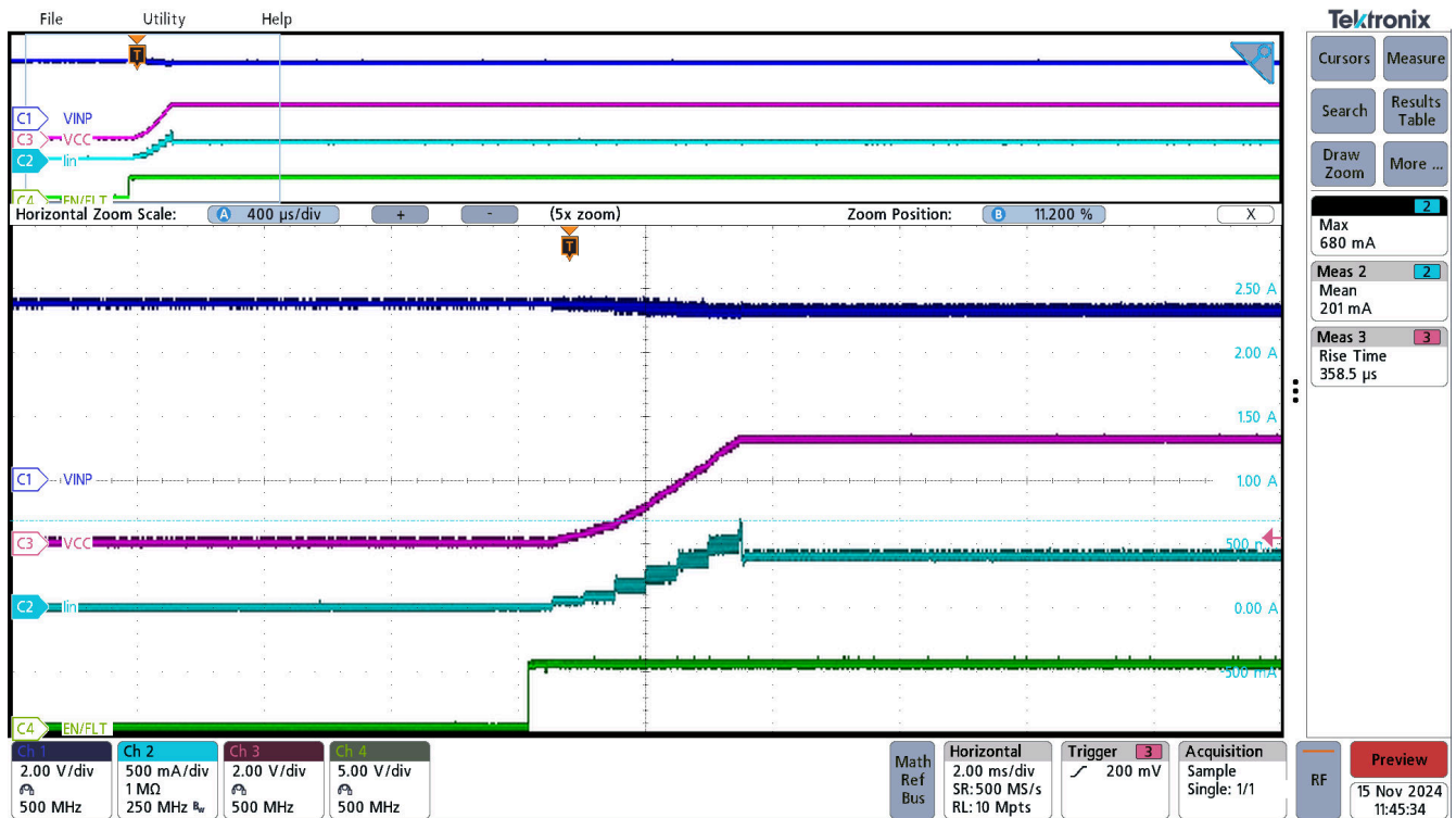
Figure 3-12. UCC33411-Q1 Inrush current, sequence VINP=5.0V → EN=5.0V, VCC=3.3V, Rload=10Ω
