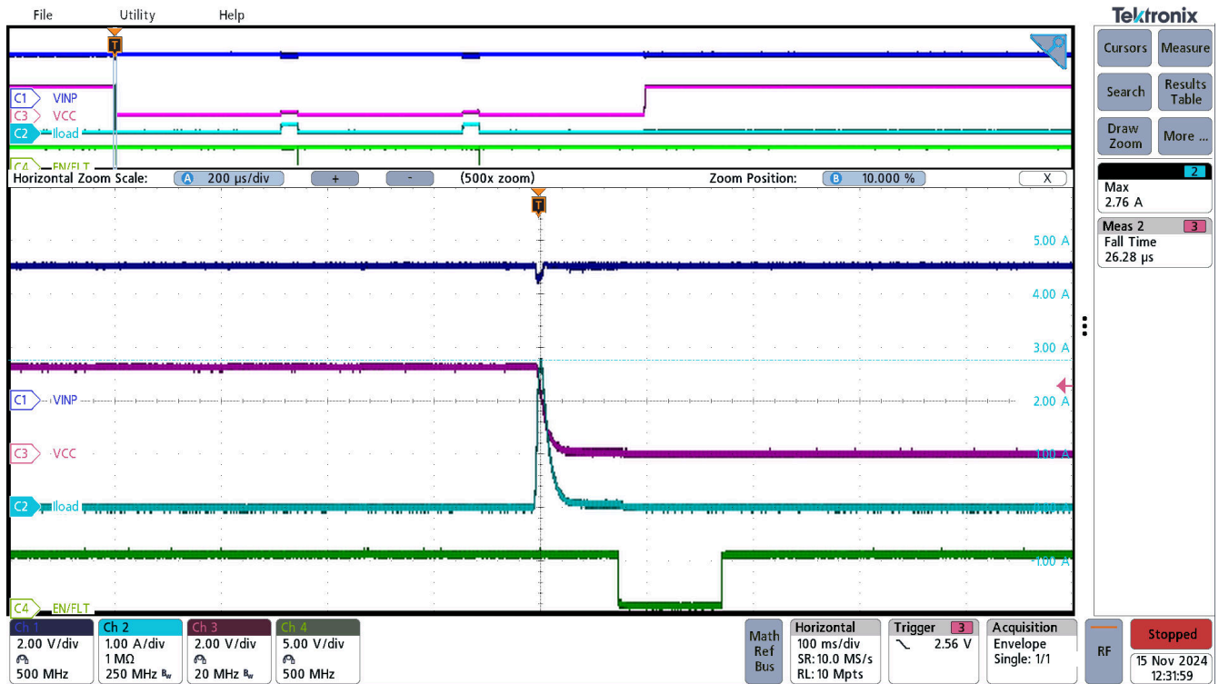
Figure 3-22. UCC33411-Q1 Short circuit, VINP=5.0V, VCC=3.3V
