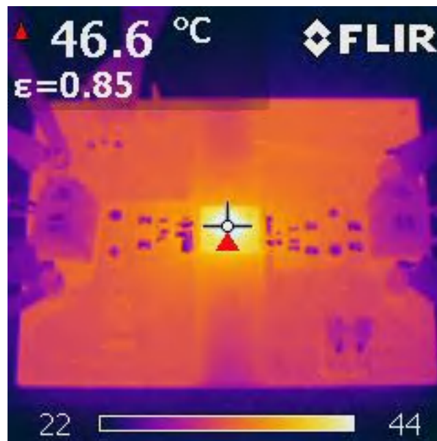
Figure 3-26. UCC33411-Q1 VINP=5.0V, VCC=3.3V, I out =150 mA, P out =0.5W, TA=25°C
