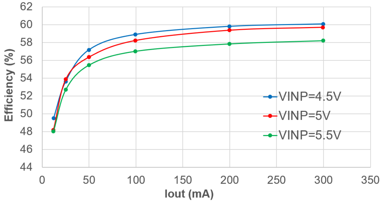
Figure 3-1. UCC33421-Q1 Efficiency VCC=5.0V
