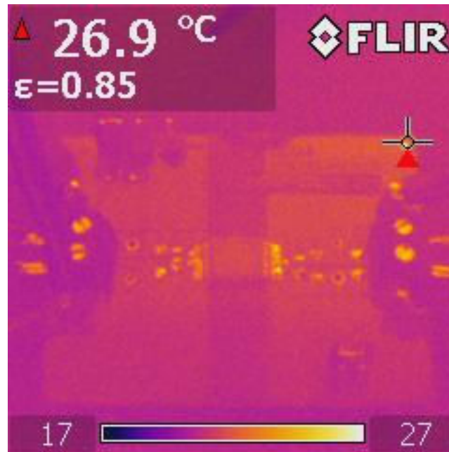
Figure 3-27. UCC33421-Q1 VINP=5.0V, VCC=5.0V, I out =0mA, P out =0W, TA=25°C
