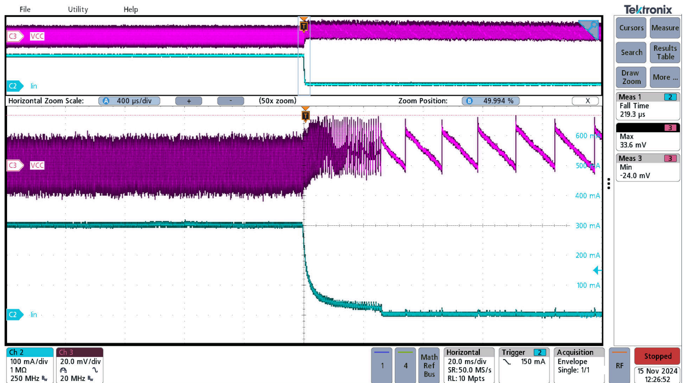
Figure 3-20. UCC33411-Q1 Load transient, VINP=5.0V, VCC=3.3V, Full load ( I_{out}=300\text{mA} ) to No load ( I_{out}=0\text{mA} )
