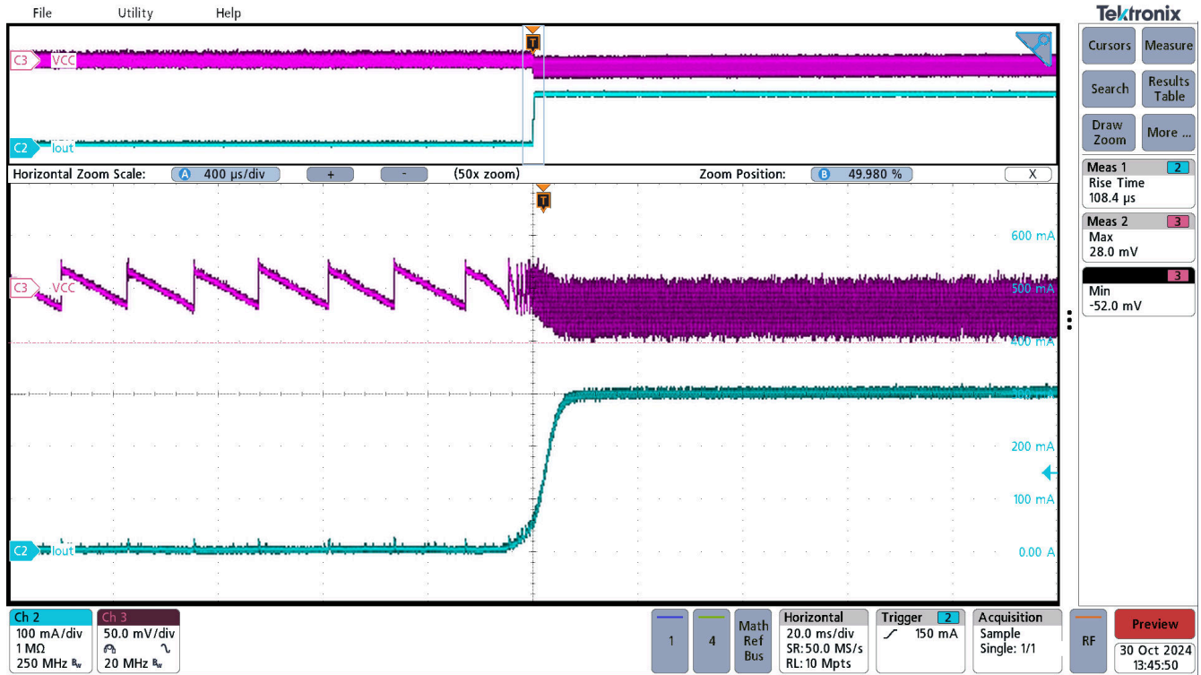
Figure 3-17. UCC33421-Q1 Load transient, VINP=5.0V, VCC=5.0V, No load (I out =0mA) to Full load (I out =300mA)
