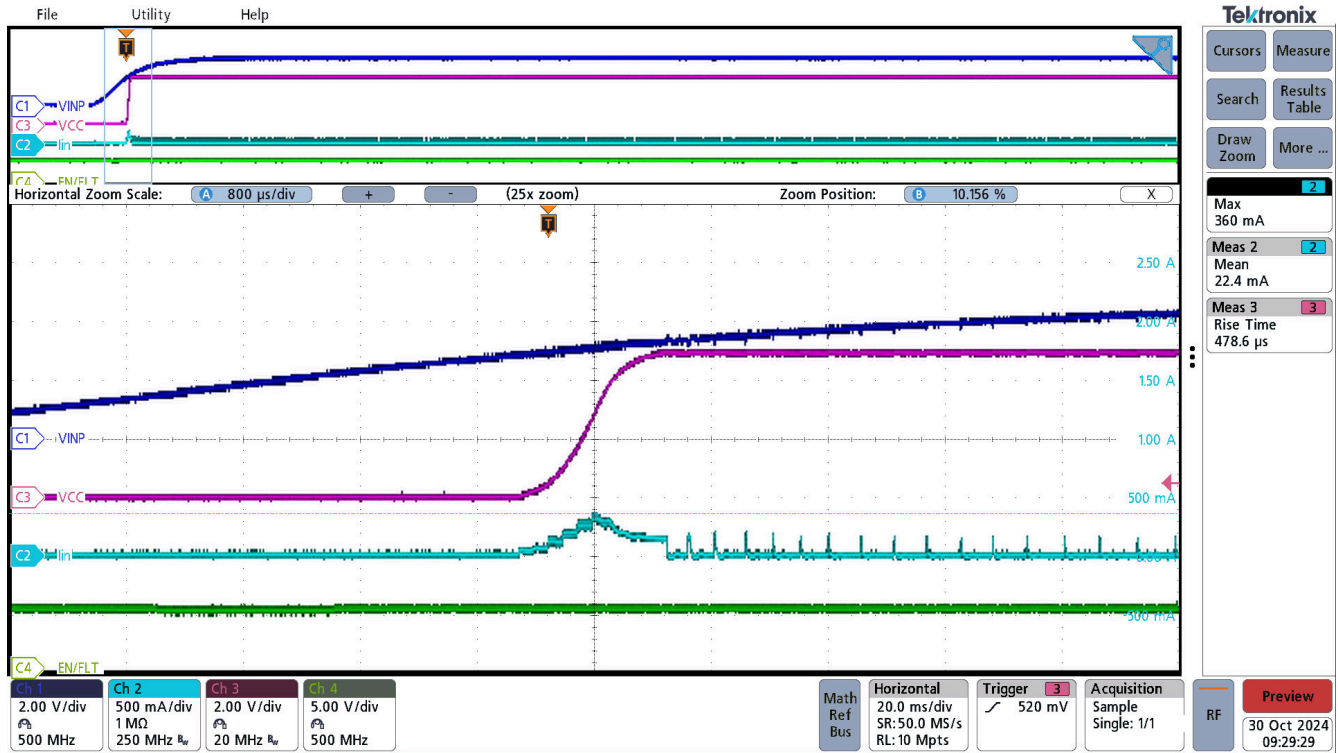
Figure 3-5. UCC33421-Q1 Start-up, sequence EN=5.0V → VINP=5.0V, VCC=5.0V, I out =0mA
