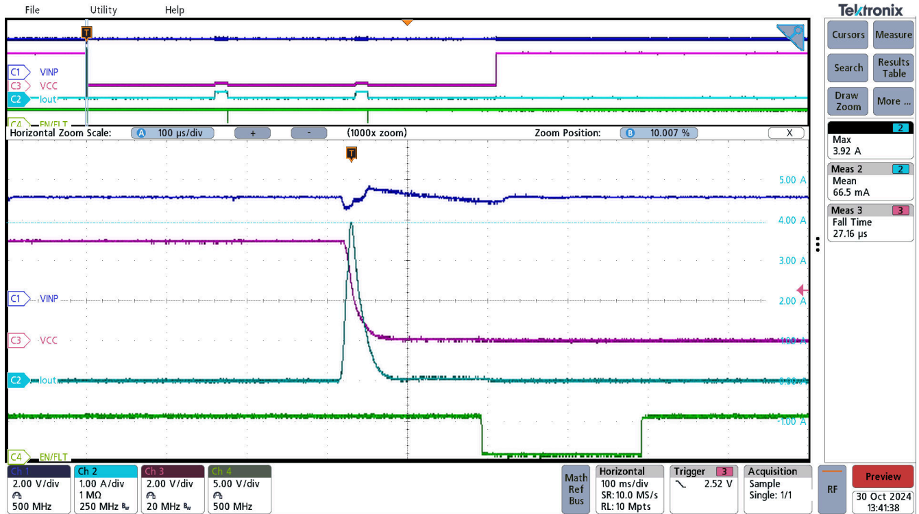
Figure 3-21. UCC33421-Q1 Short circuit, VINP=5.0V, VCC=5.0V
