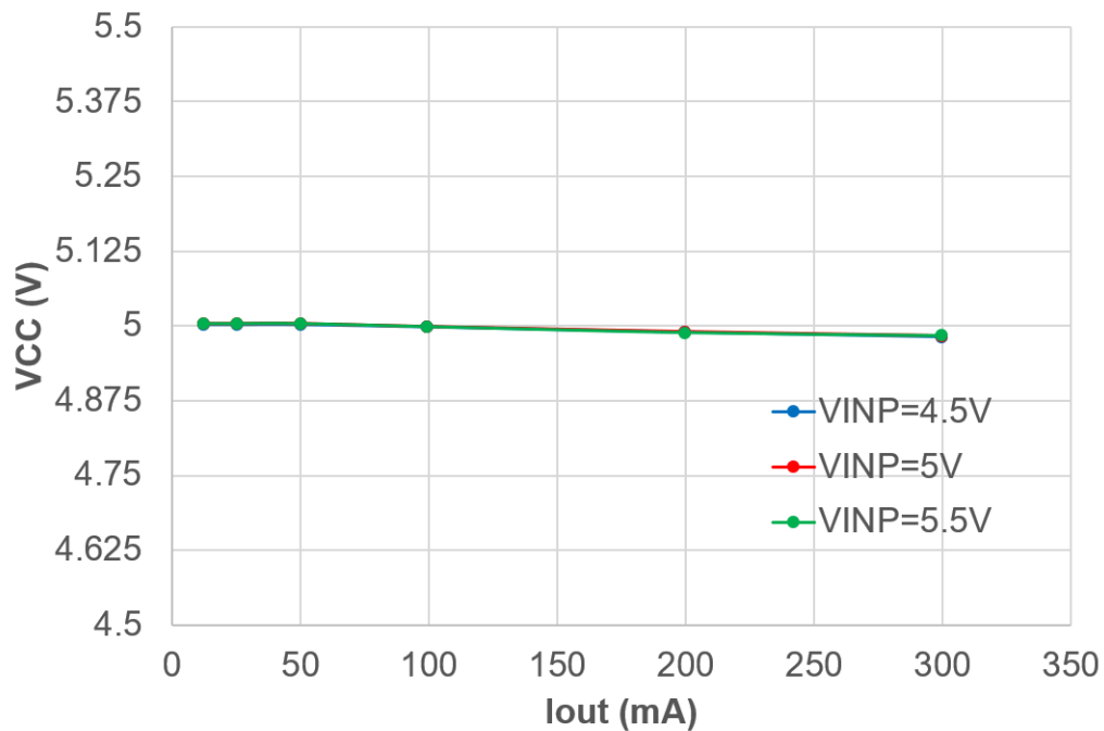
Figure 3-3. UCC33421-Q1 Regulation vs Load Current VCC=5.0V
