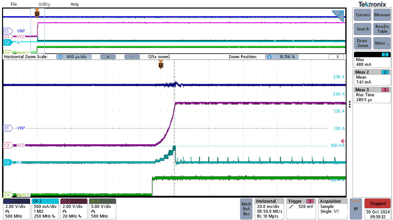
Figure 3-9. UCC33421-Q1 Inrush current , sequence VINP=5.0V → EN=5.0V, VCC=5.0V, I out =0mA
