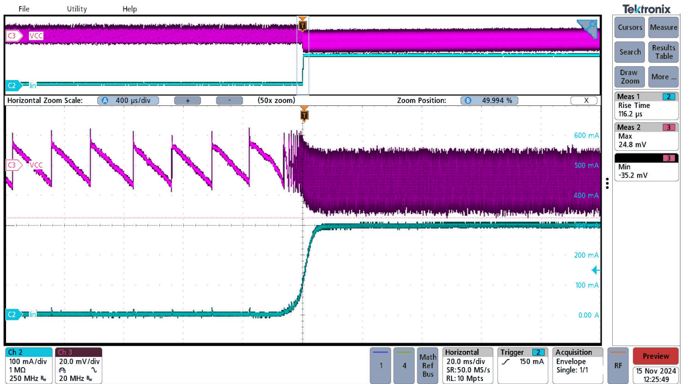
Figure 3-18. UCC33411-Q1 Load transient, VINP=5.0V, VCC=3.3V, No load (I out =0mA) to Full load (I out =300mA)
