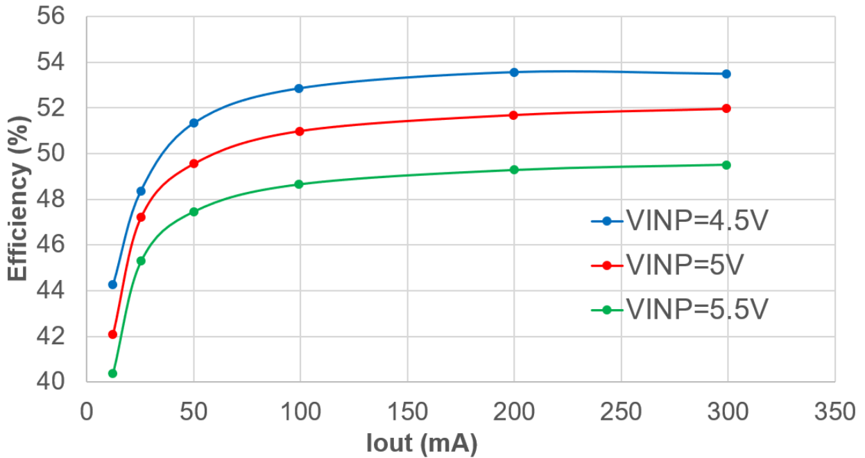
Figure 3-2. UCC33411-Q1 Efficiency VCC=3.3V
