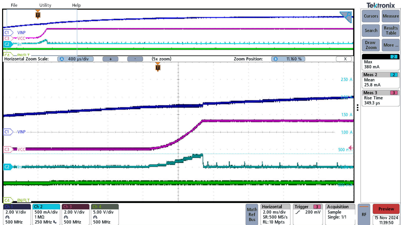
Figure 3-6. UCC33411-Q1 Start-up, sequence EN=5.0V → VINP=5.0V, VCC=3.3V, I out =0mA
