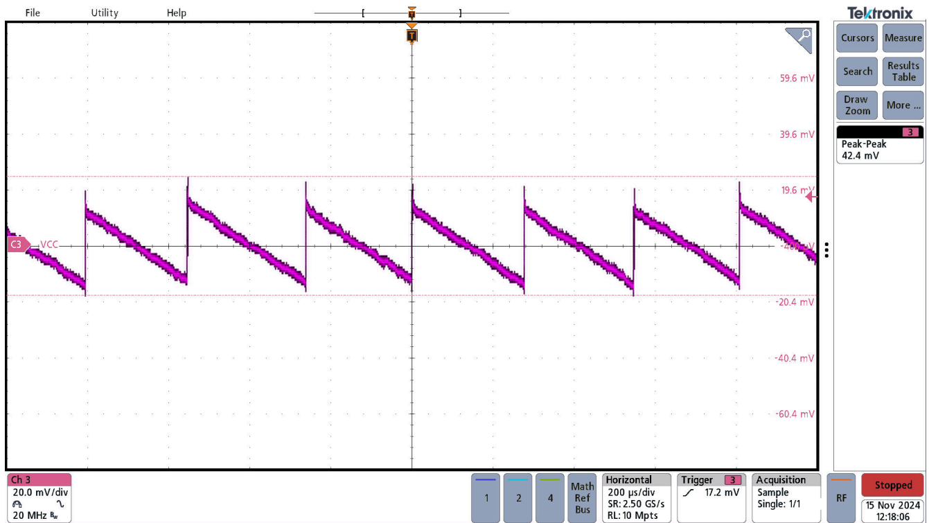
Figure 3-14. UCC33411-Q1 VCC AC Ripple, VINP=5.0V, VCC=3.3V, I out =0mA
