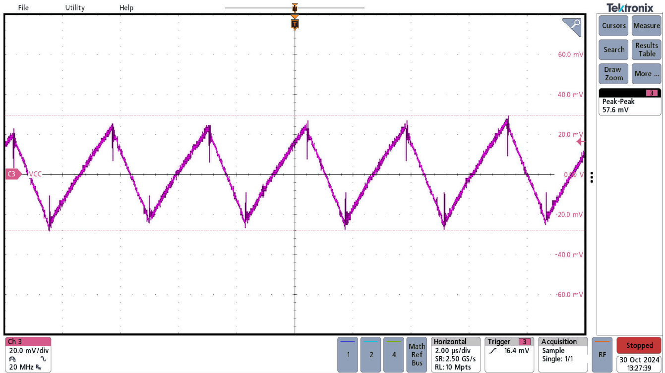
Figure 3-15. UCC33421-Q1 VCC AC Ripple, VINP=5.0V, VCC=5.0V, I out =300mA
