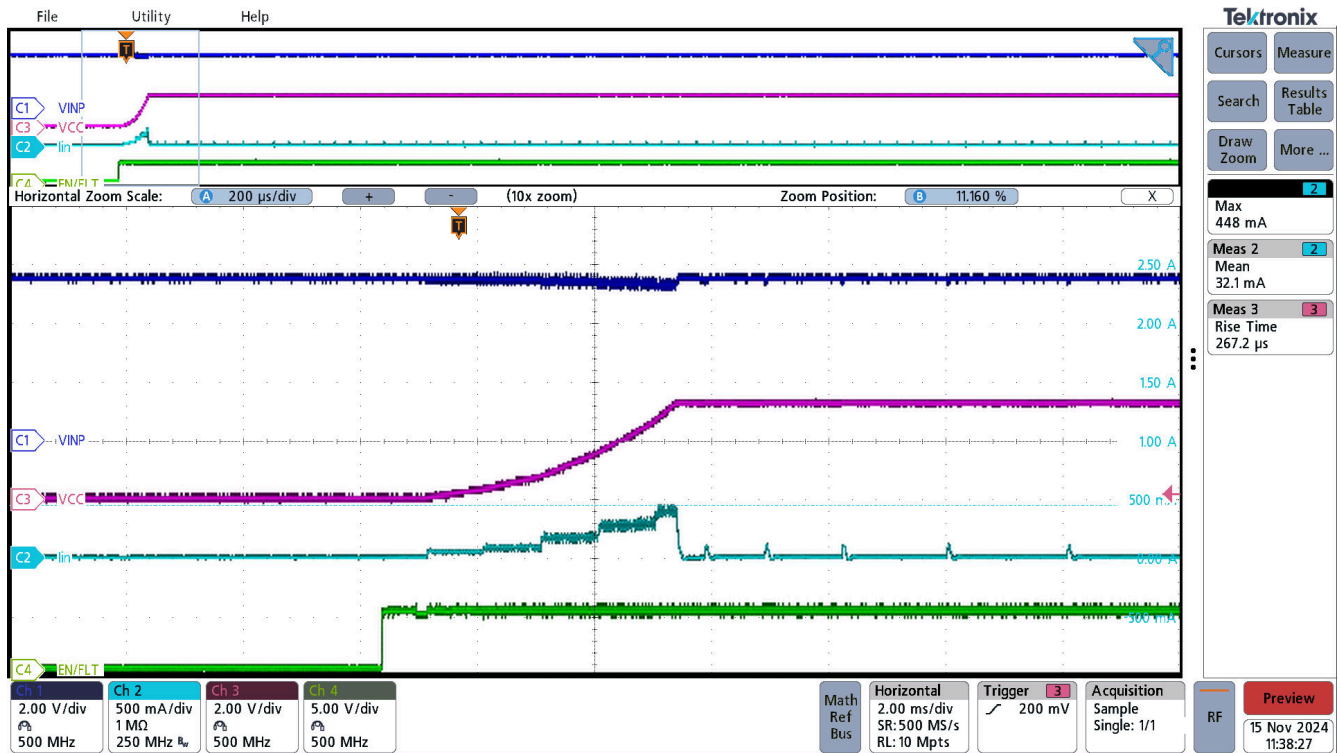
Figure 3-10. UCC33411-Q1 Inrush current , sequence VINP=5.0V → EN=5.0V, VCC=3.3V, I out =0mA
