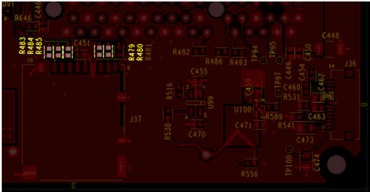
Figure 5-5. MMC1 Layout
