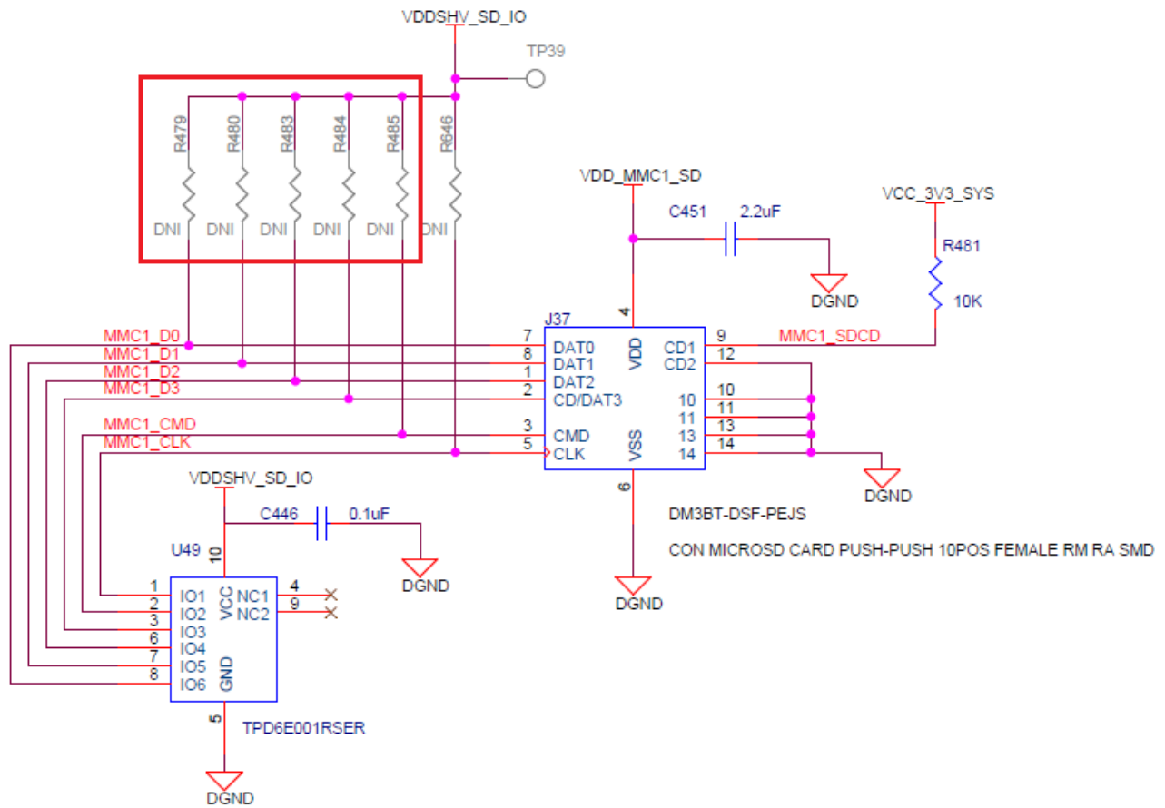
Figure 5-4. MMC1 Schematics
