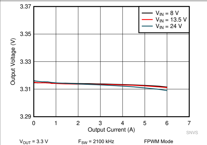
10-16. LM61460-Q1 Load and Line Regulation
