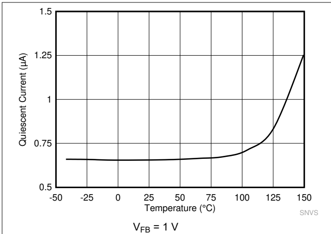
8-1. Non-Switching Input Supply Current
