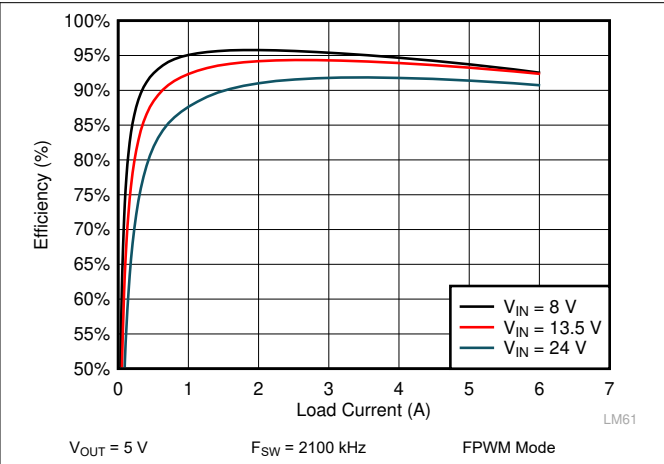
10-12. LM61460-Q1 Efficiency
