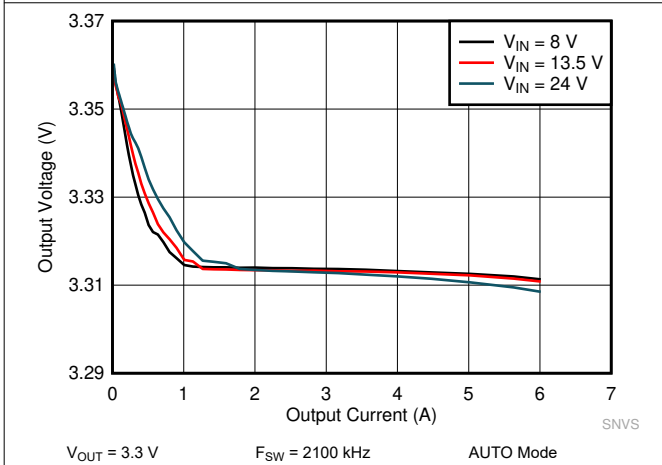
10-15. LM61460-Q1 Load and Line Regulation
