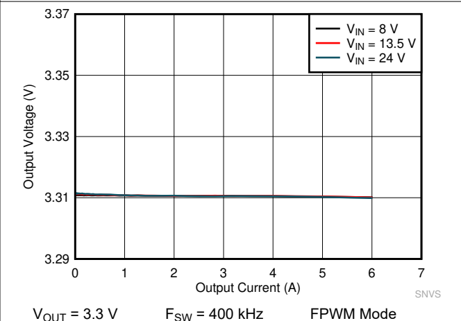
10-14. LM61460-Q1 Load and Line Regulation
