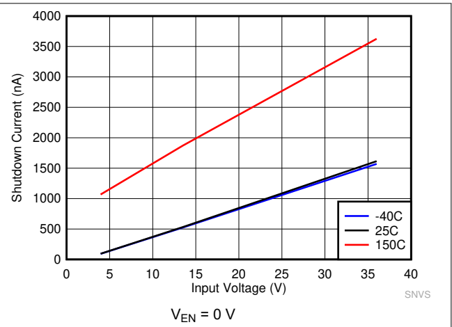
8-2. Shutdown Supply Current
