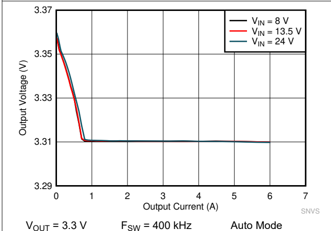
10-13. LM61460-Q1 Load and Line Regulation
