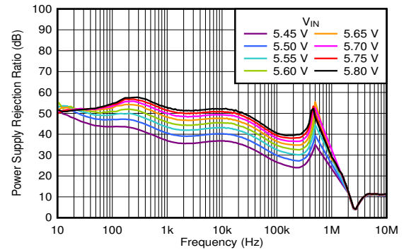
6-50. PSRR vs Frequency and V_{IN} ( V_{OUT} = 5\text{ V} )
