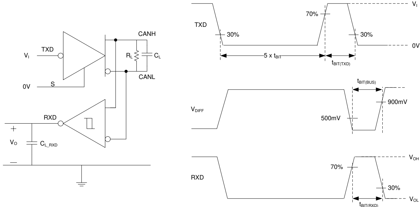
FIG 7-5. CAN FD Timing Parameter Measurement
