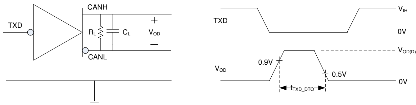
FIG 7-5. CAN FD Timing Parameter Measurement
