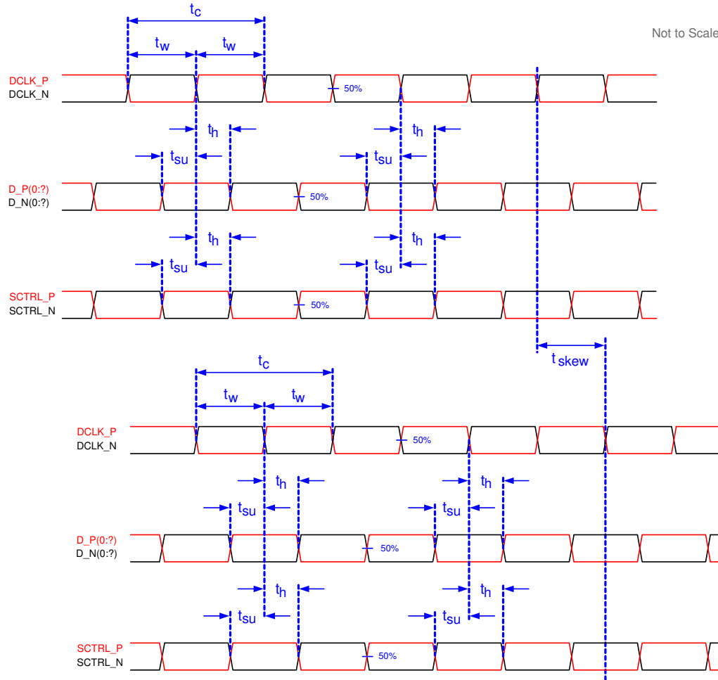
Figure 5-6. Timing Requirements
