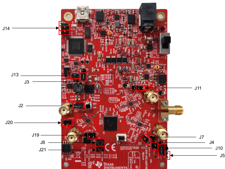
Figure 3-2. Jumper Locations
