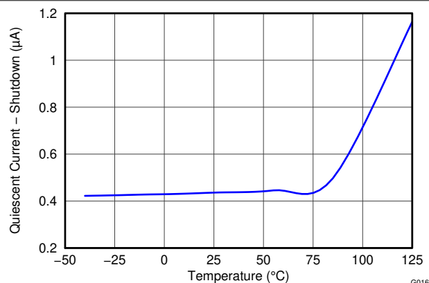
Figure 5-16. Shutdown I_Q vs Temperature
