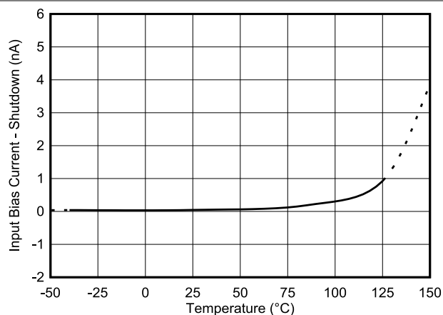
Figure 5-14. Input Bias Current vs Temperature, Shutdown
