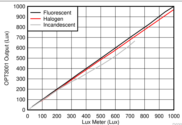
Figure 8-6. Compensated Output of the OPT3001-Q1 Grade 3 Device Under a Dark Window Illuminated by Fluorescent, Halogen, and Incandescent Light Sources
