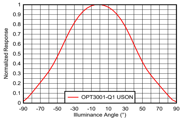
Figure 5-15. Normalized Response vs Illuminance Angle
