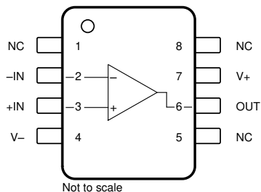
Figure 4-1. TLV888: D Package, 8-Pin SOIC (Top View)
