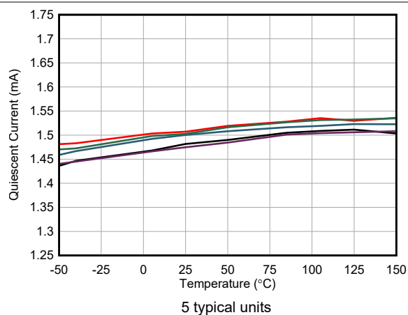
Figure 5-26. Quiescent Current vs Temperature
