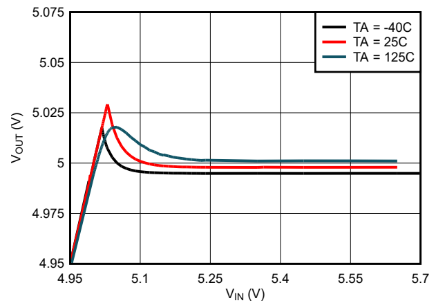
Figure 6-12. V_{OUT} Vs V_{IN} across Temperature
