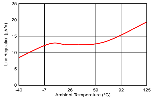
Figure 6-10. Line Regulation vs Temperature V_{OUT} = 2.5\text{V}
