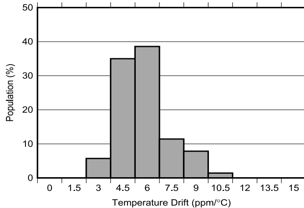
Figure 6-3. Temperature Drift Histogram 0°C to +70°C
