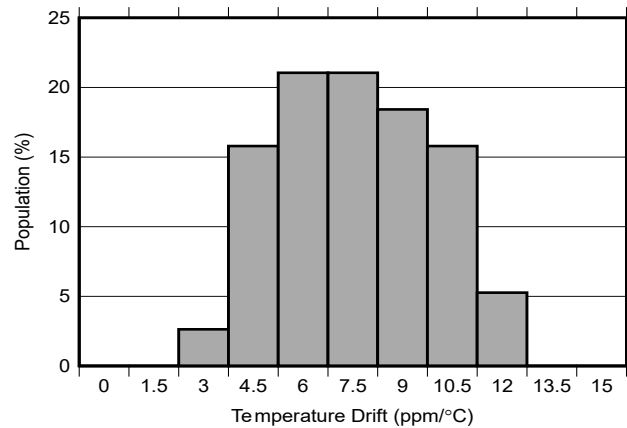
Figure 6-2. Temperature Drift Histogram -40°C to +85°C
