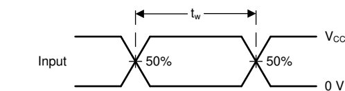
Figure 6-2. Voltage Waveforms, Pulse Duration
