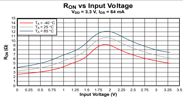
Figure 5-2. R_{ON} vs Input Voltage, V_{DD} = 3.3\text{V} , I_{DS} = 64\text{mA}
