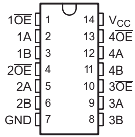
Figure 4-1. DYY, DGV or PW Package, 14-Pin SOT, TVSOP or TSSOP (Top View)
