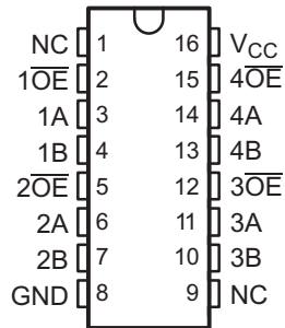
Figure 4-3. DBQ Package, 16-Pin SSOP (Top View)
