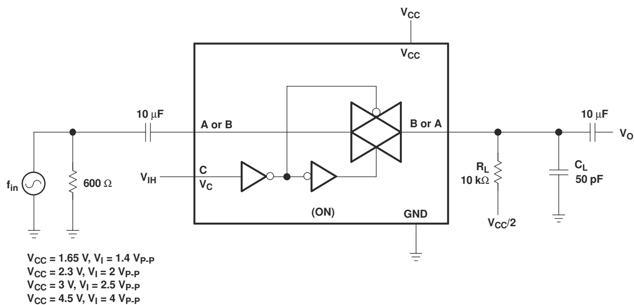
Figure 6-8. Sine-Wave Distortion
