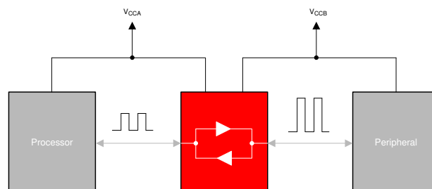
Typical Application Block Diagram for TXB0604
