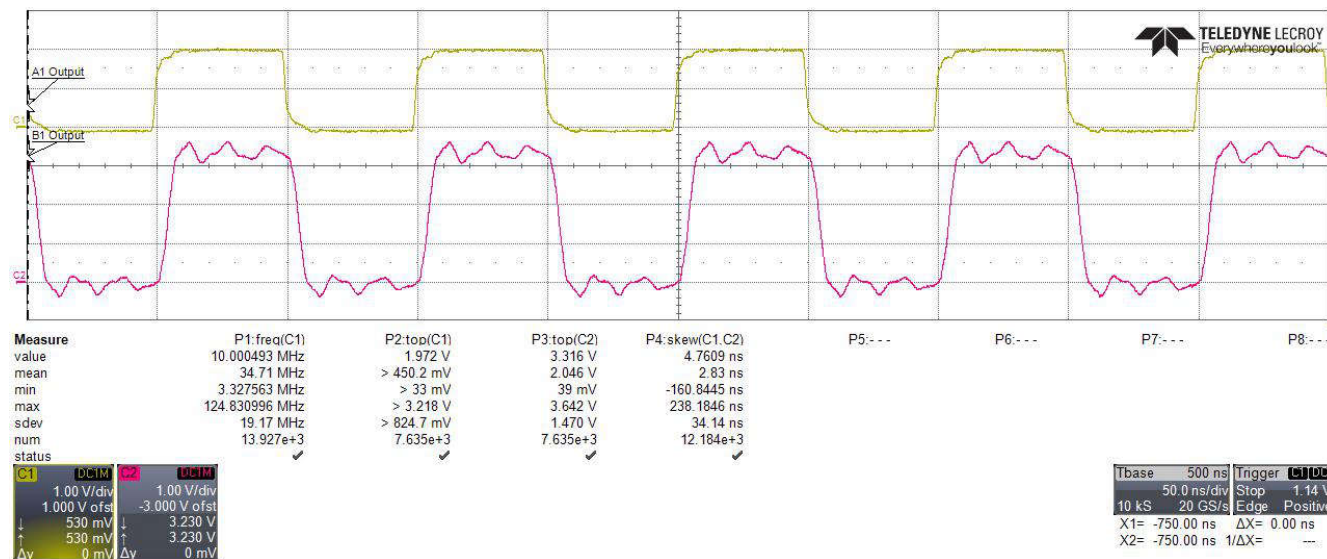
Figure 8-1. Level-Translation of a 10MHz Signal ( V_{CCA} = 1.8V , V_{CCB} = 3.6V , C_L = 20\text{inch} + 50\text{pF} )
