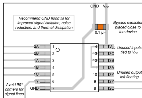
Figure 8-3. Example layout for the SN74HCS4075-Q1
