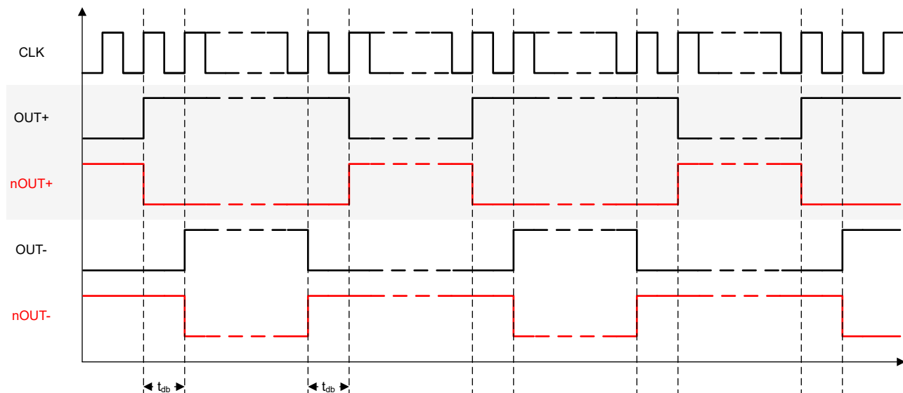
Figure 8-39. PWM Generator Timing Example
