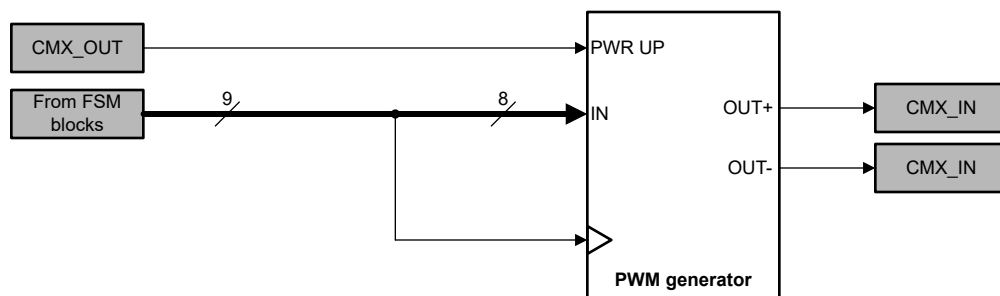
Figure 8-38. PWM Generator Block Diagram
