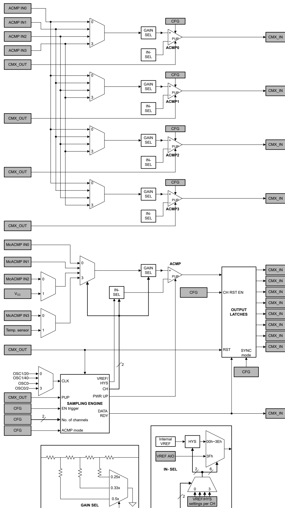
Figure 8-43. Analog Comparators Block Diagram
