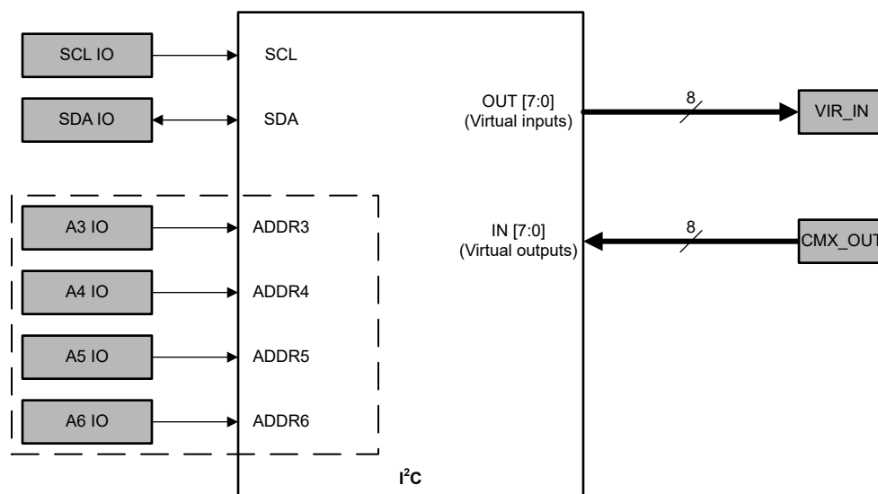
Figure 8-50. I 2 C Serial Communications GPIO Allocation
