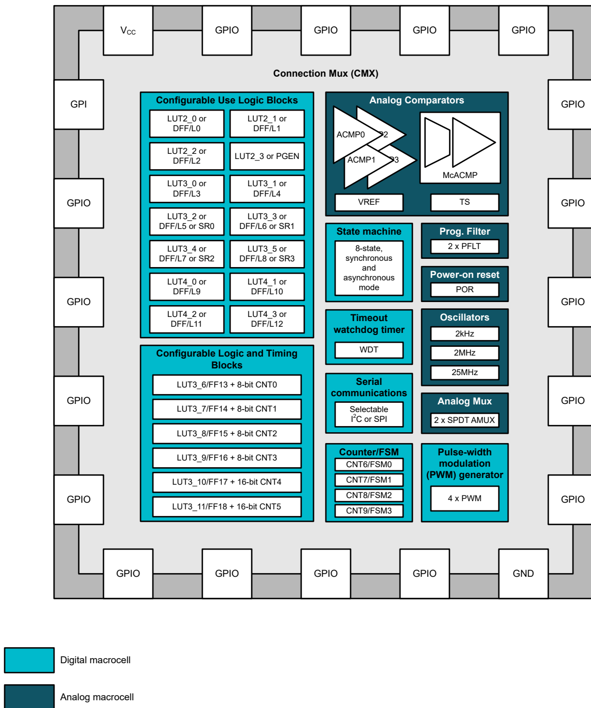
Figure 8-1. TPLD2001 Functional Block Diagram
