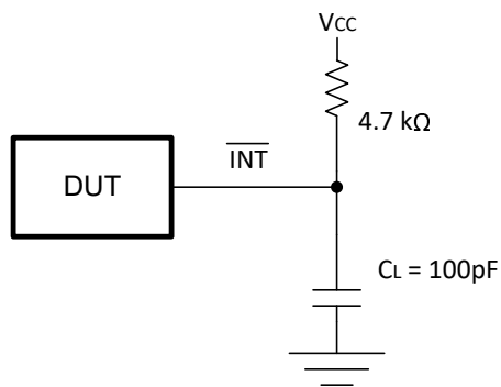
INTERRUPT LOAD CONFIGURATION
