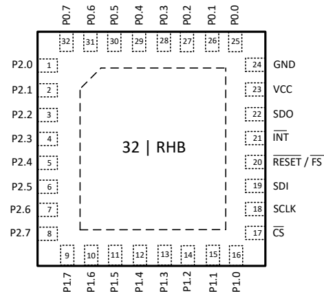
Figure 4-2. TXE8124-Q1 RHB (VQFN) Package, 32-Pin (Top View)
