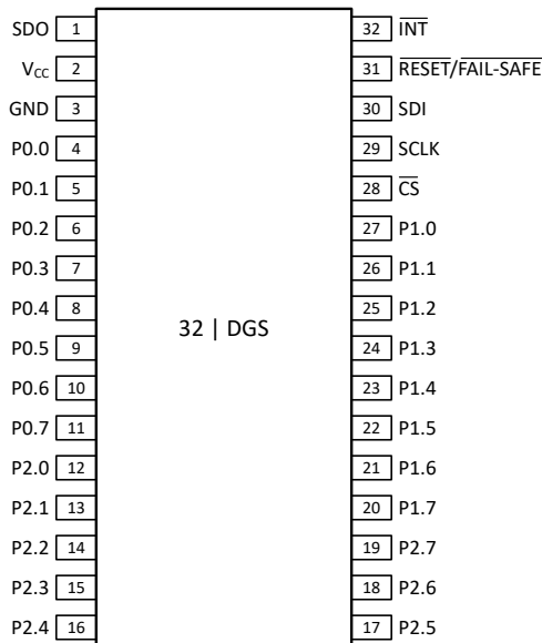
Figure 4-1. TXE8124-Q1 DGS (VSSOP) Package, 32-Pin (Top View)
