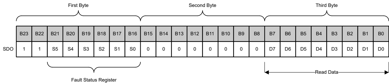
Figure 7-6. SPI SDO Data Format
