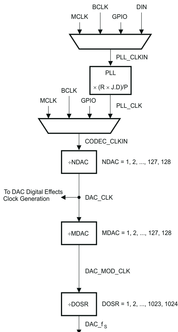
Figure 4-8. Clock Distribution Tree
