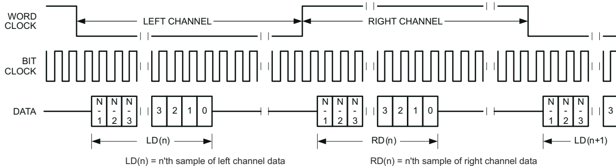
Figure 4-15. Timing Diagram for I²S Mode
