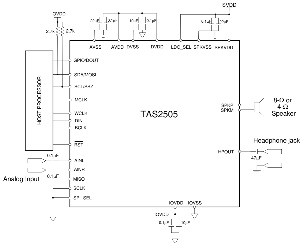
Figure 3-3. Application Schematics for LDO
