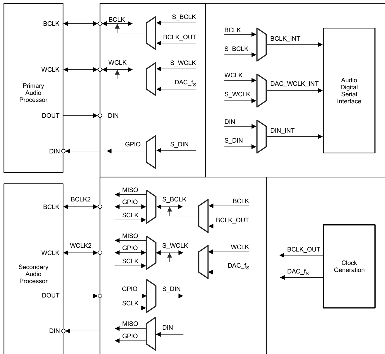
Figure 4-21. Audio Serial Interface Multiplexing
