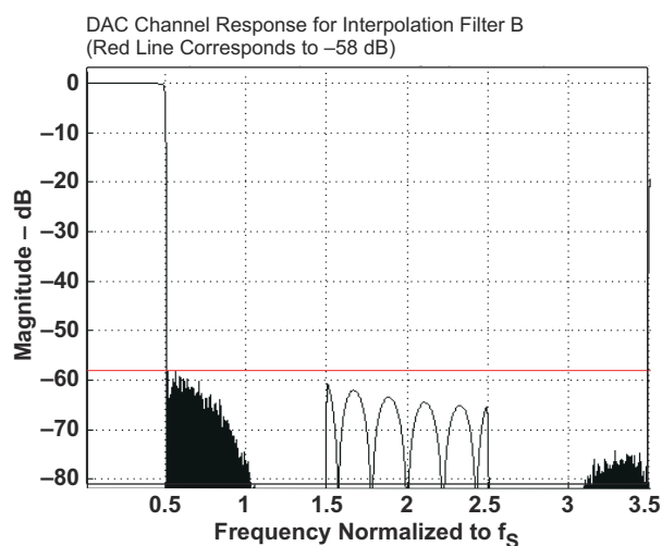
Figure 4-4. Frequency Response of Channel Interpolation Filter B
