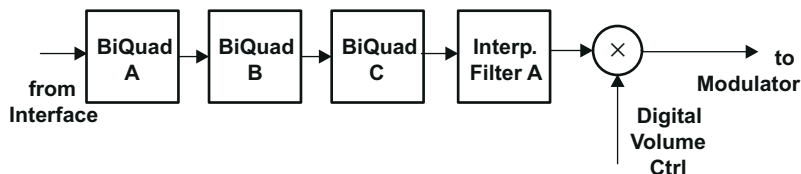
Figure 4-1. Signal Chain for PRB_P2
