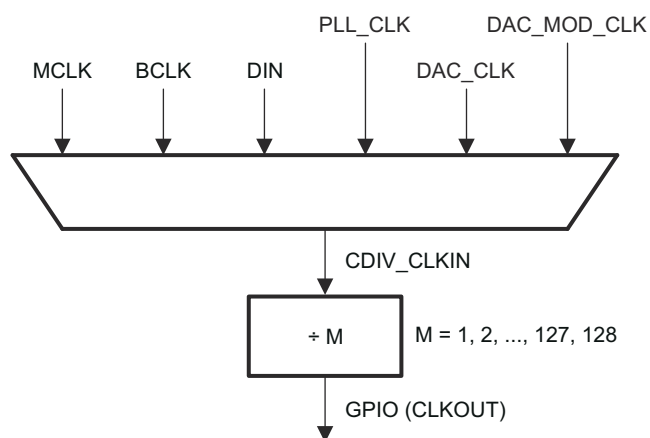
Figure 4-10. General-Purpose Clock Output Options
