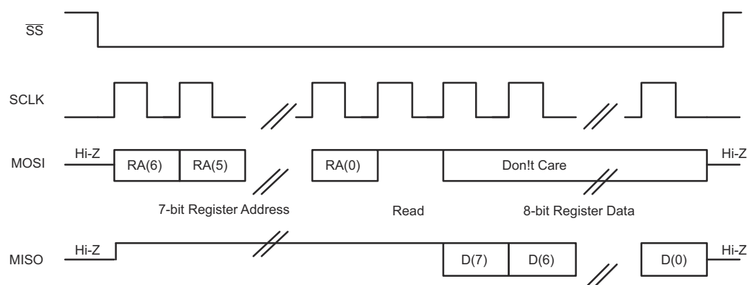
Figure 4-25. SPI Timing Diagram for Register Read
