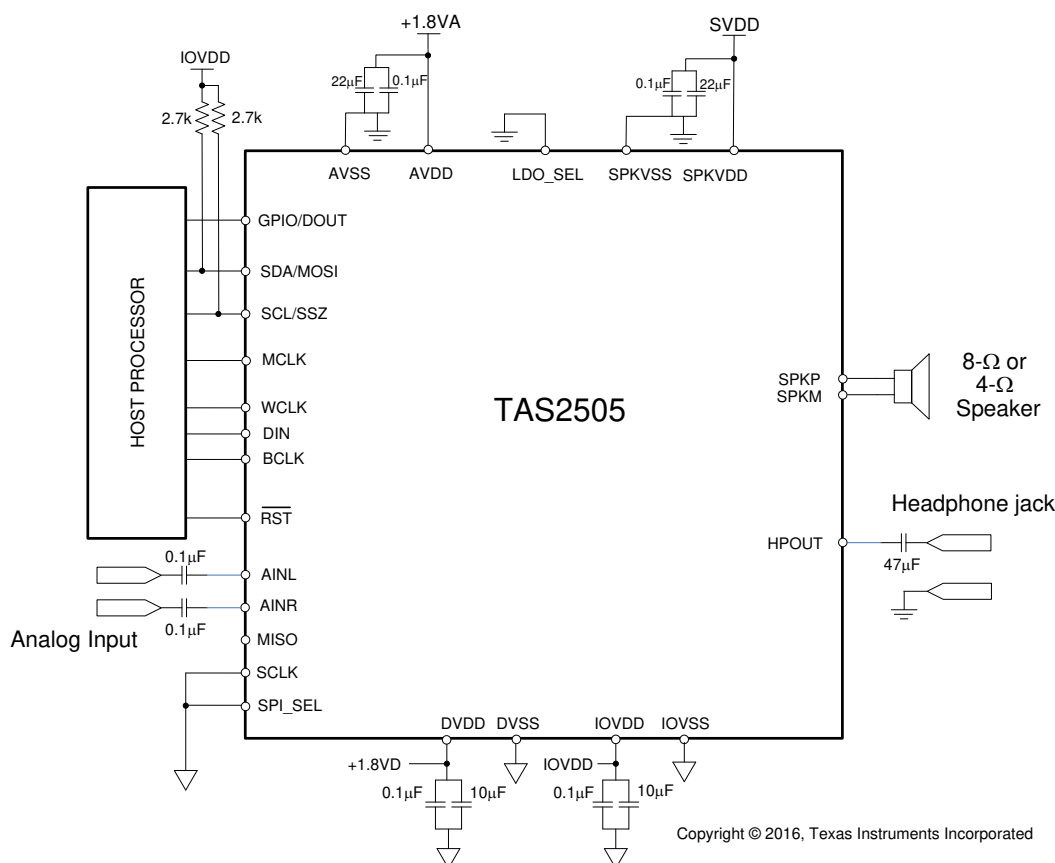
Figure 3-2. Typical Circuit Configuration
