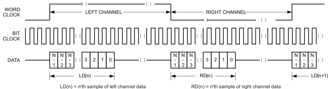
Figure 4-12. Timing Diagram for Left-Justified Mode
