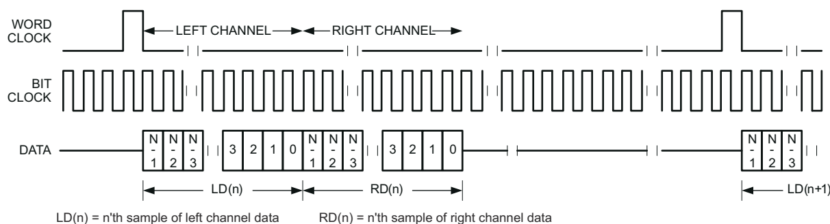
Figure 4-19. Timing Diagram for DSP Mode With Offset = 1
