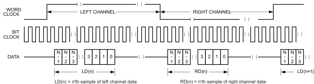
Figure 4-13. Timing Diagram for Left-Justified Mode With Offset = 1
