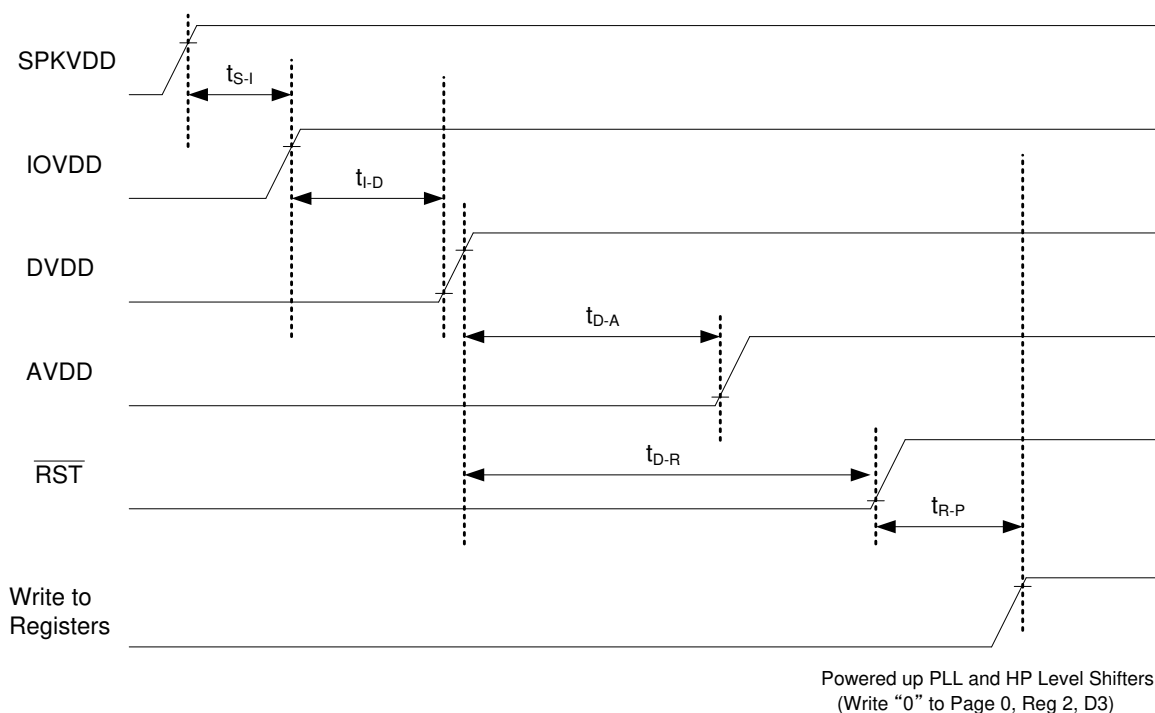
Figure 5-1. Analog Supply provided after Digital Supply
