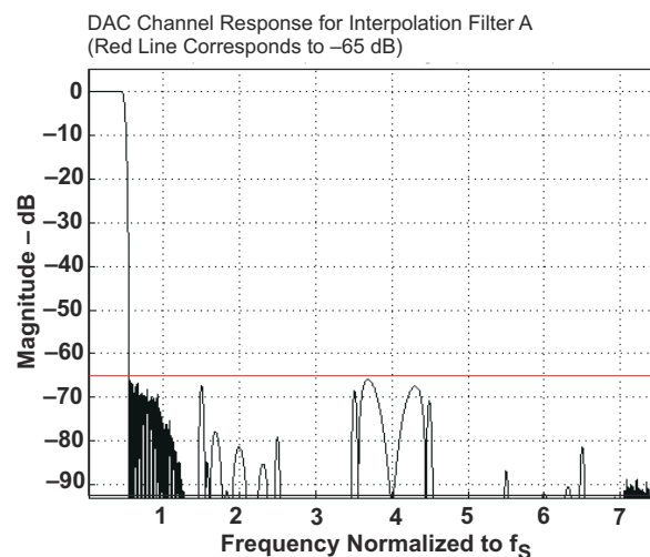
Figure 4-3. Frequency Response of DAC Interpolation Filter A
