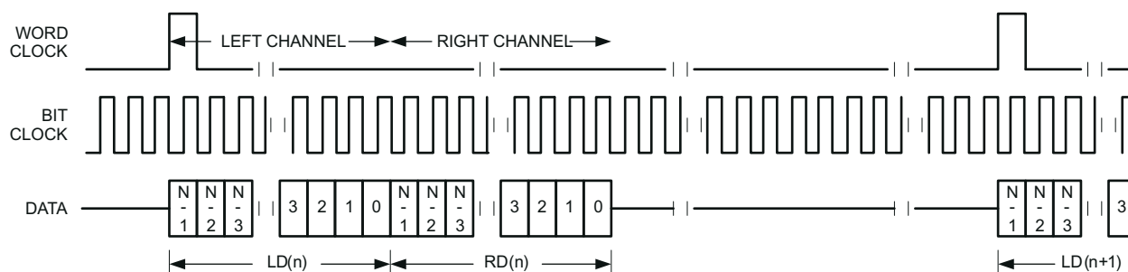
Figure 4-20. Timing Diagram for DSP Mode With Offset = 0 and Bit Clock Inverted
