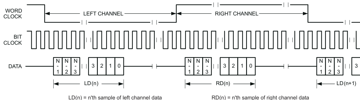
Figure 4-17. Timing Diagram for I²S Mode With Offset = 0 and Bit Clock Inverted
