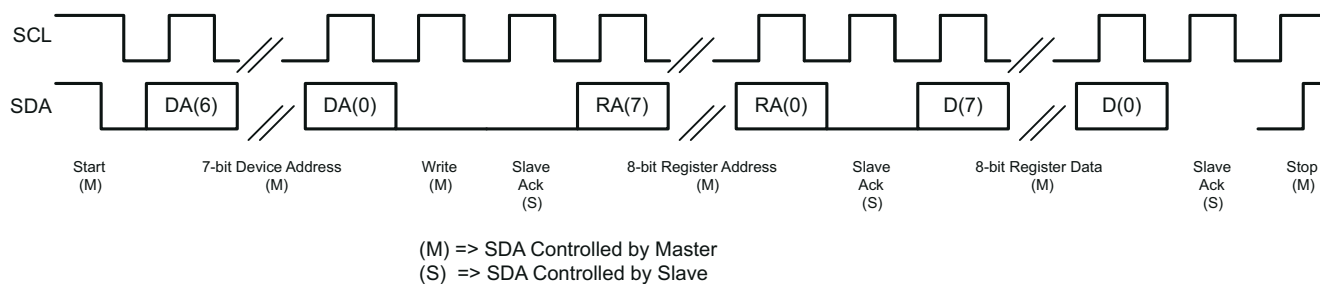
Figure 4-22. I²C Write
