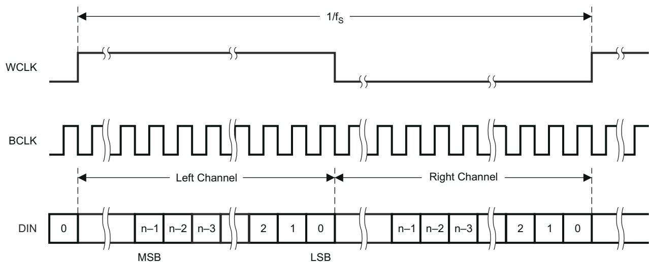
Figure 4-11. Timing Diagram for Right-Justified Mode
