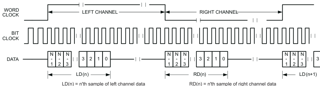
Figure 4-14. Timing Diagram for Left-Justified Mode With Offset = 0 and Inverted Bit Clock
