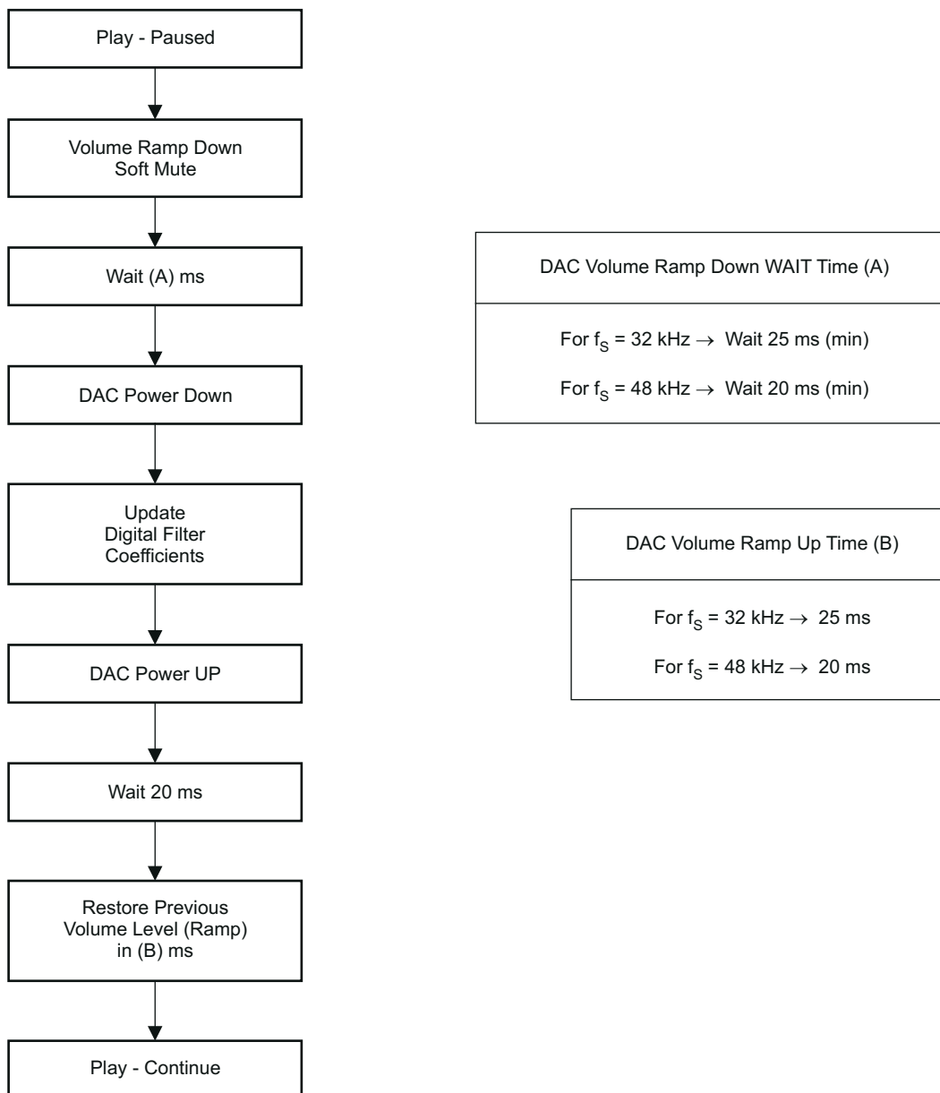
Figure 4-5. Example Flow For Updating DAC Digital Filter Coefficients During Play
