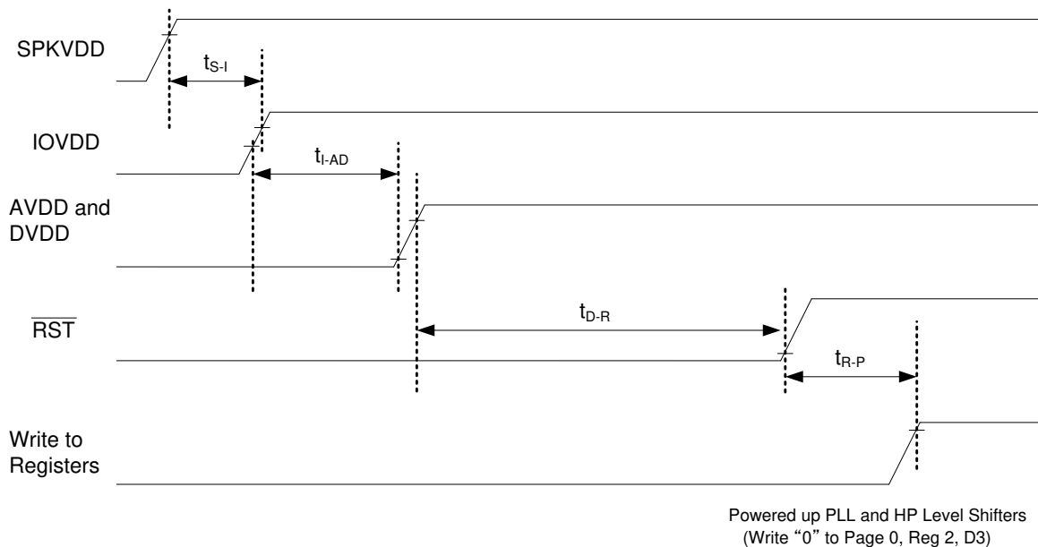
Figure 5-2. Digital and Analog 1.8 V Supplies provided Together
