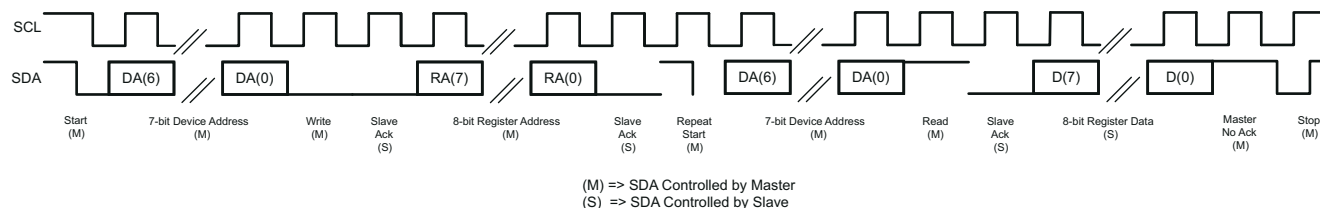
Figure 4-23. I²C Read
