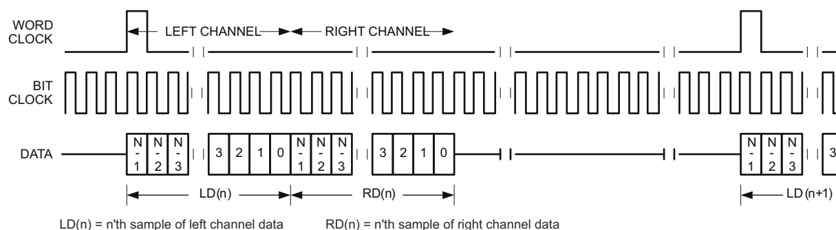
Figure 4-18. Timing Diagram for DSP Mode
