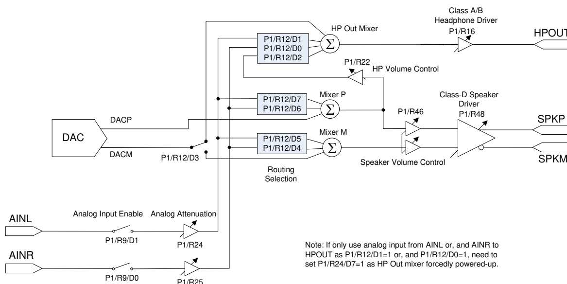
Figure 4-6. Analog Block Diagram
