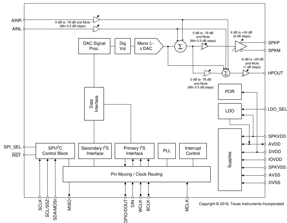
Figure 3-1. Simplified Block Diagram
