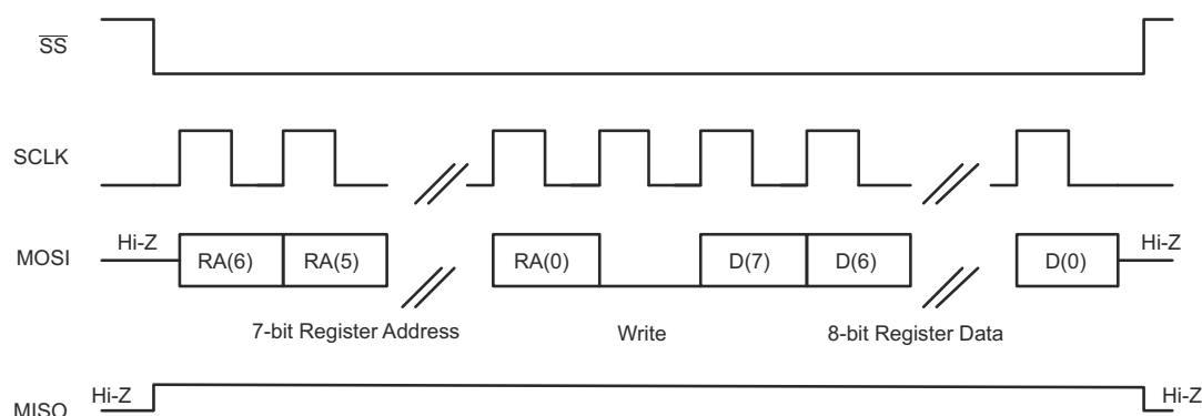
Figure 4-24. SPI Timing Diagram for Register Write
