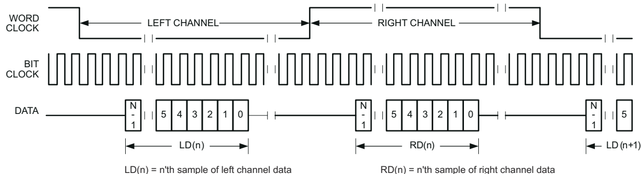
Figure 4-16. Timing Diagram for I²S Mode With Offset = 2
