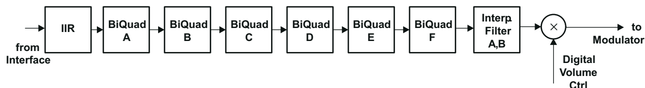
Figure 4-2. Signal Chain for PRB_P1 and PRB_P3
