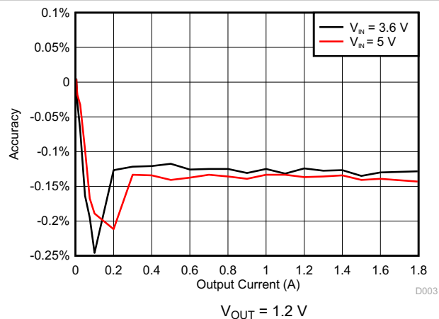
Figure 5-3. DCDC3 Accuracy
