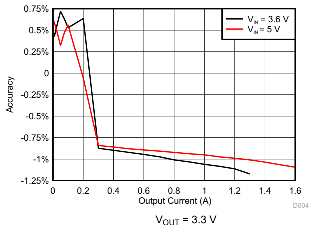
Figure 5-4. DCDC4 Accuracy
