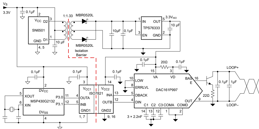
Figure 8-1. Isolated 4mA to 20mA Current Loop
