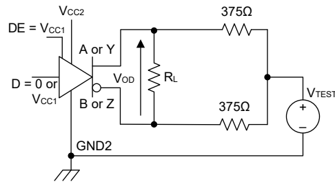
Figure 7-1. Driver Voltages
