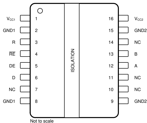
Figure 5-2. DW Package 16-Pin SOIC Half-Duplex Device Top View
