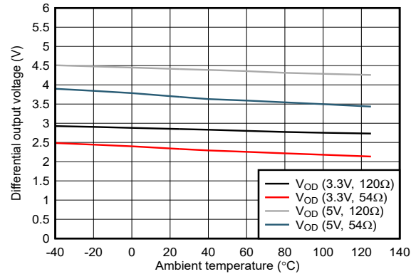
Figure 6-14. Driver Differential Output Voltage Vs Temperature
