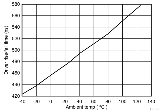
Figure 6-16. ISO141x Driver Rise/fall Time (ns) Vs Temperature (c)
