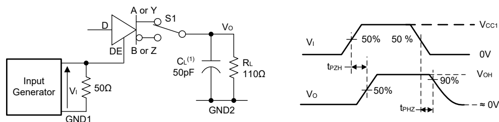
Figure 7-5. Common Mode Transient Immunity (CMTI)—Half Duplex
