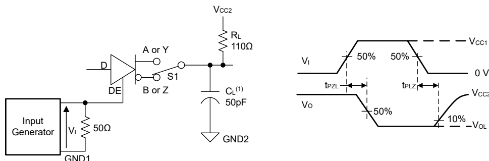
Figure 7-7. Driver Enable and Disable Times
