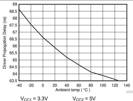
Figure 6-20. ISO143x Driver Propagation Delay (ns) Vs Temperature (C)
