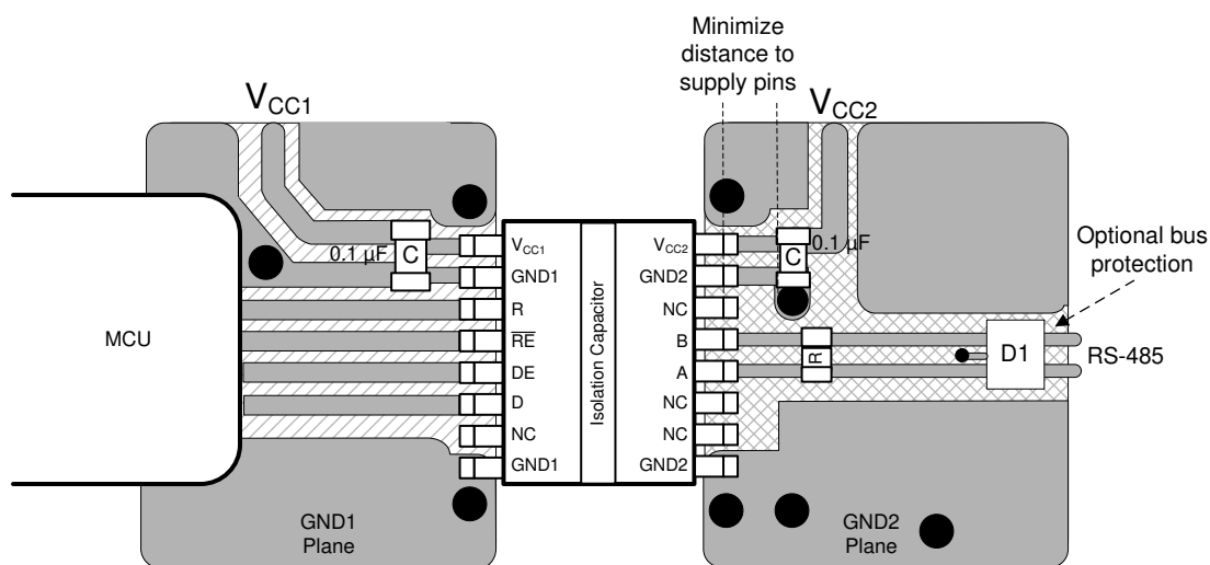
Figure 9-9. Layout Example
