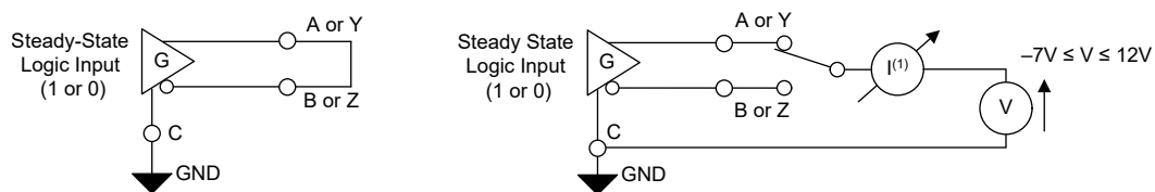
Figure 7-11. Short-Circuit Current Limiting
