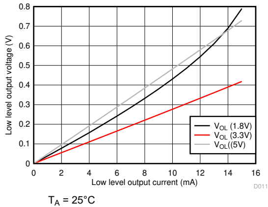
Figure 6-23. Receiver Buffer Low Level Output Voltage Vs Low Level Output Current
