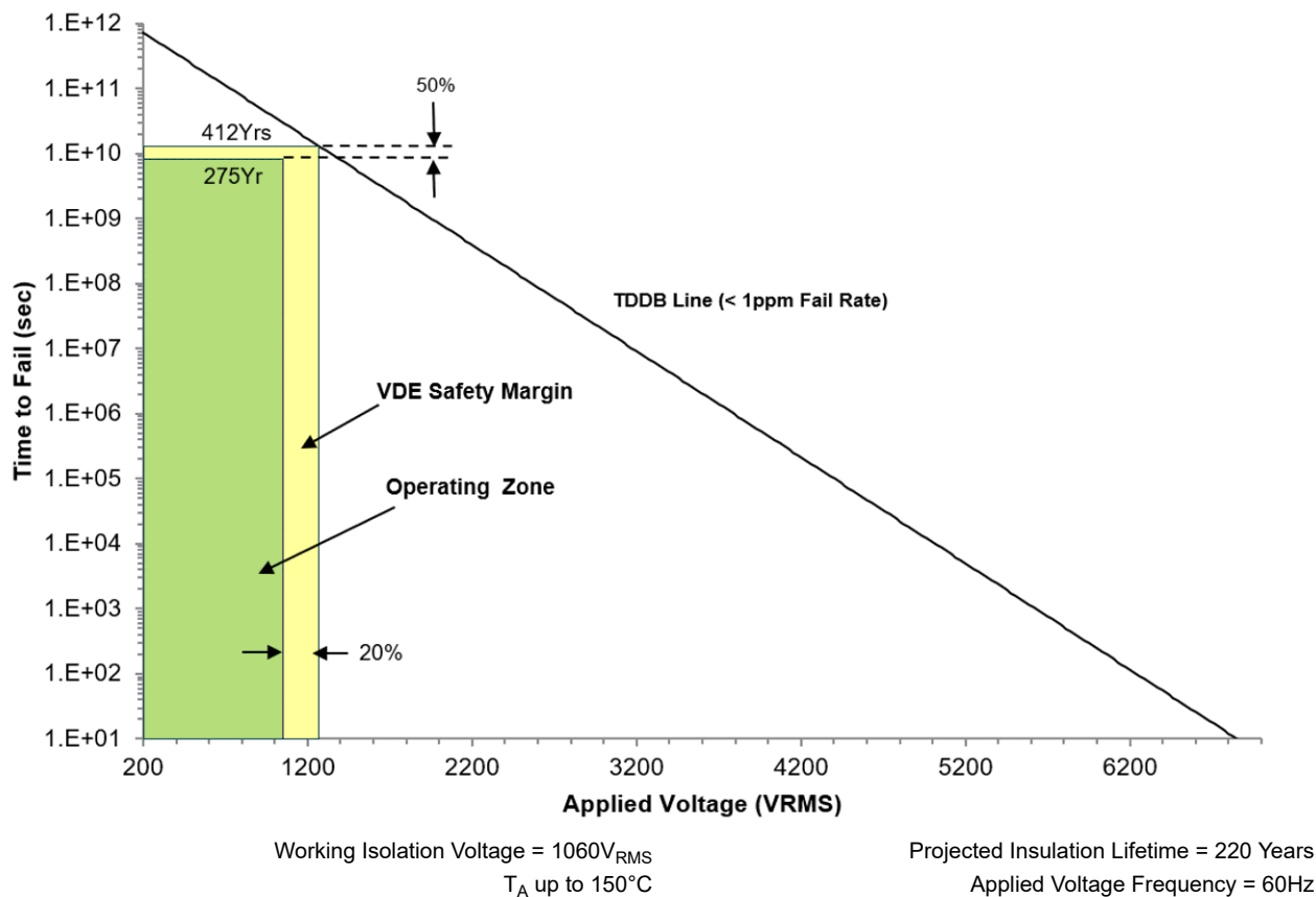
Figure 9-7. Insulation Lifetime Projection Data
