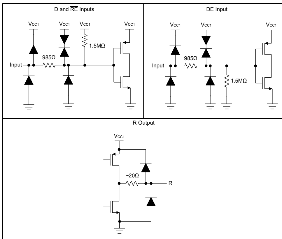
Figure 8-4. Device I/O Schematics
