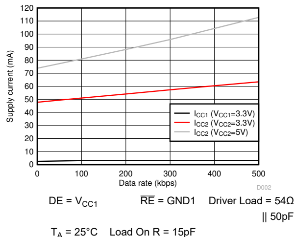
Figure 6-4. ISO141x Supply Current Vs Data Rate- With 54\Omega || 50pF Load
