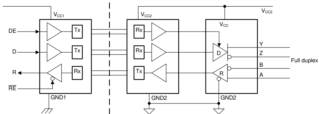
Figure 8-1. Full-Duplex Block Diagram
