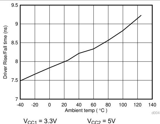
Figure 6-17. ISO143x Driver Rise/Fall Time (ns) Vs Temperature (C)
