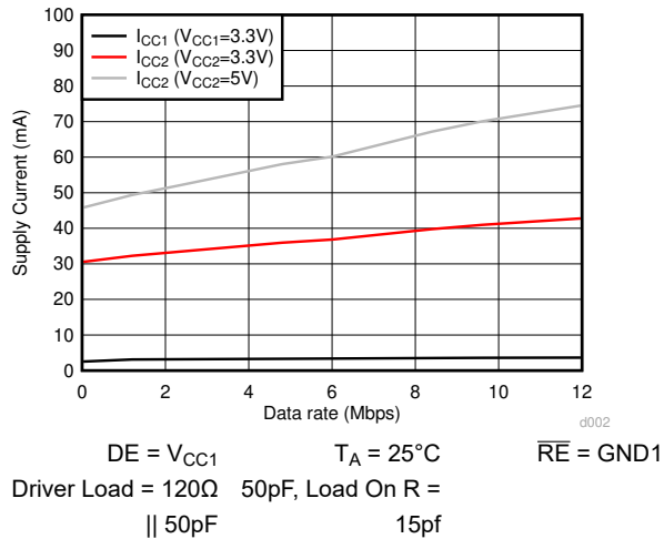
Figure 6-7. ISO143x Supply Current Vs. Data Rate - 120Ω||50pF Load
