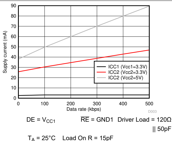
Figure 6-5. ISO141x Supply Current Vs Data Rate- With 120\Omega || 50pF Load
