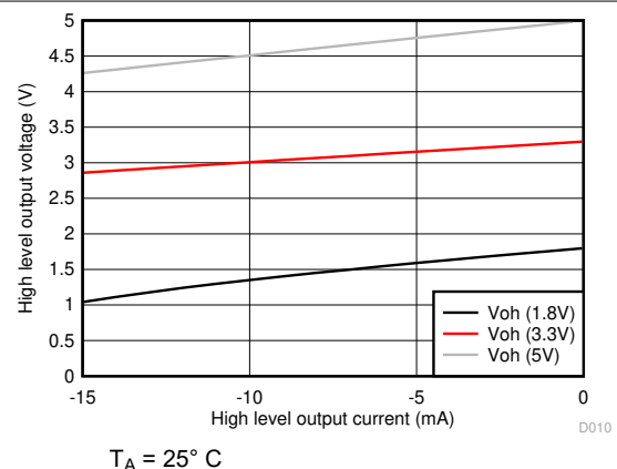
Figure 6-22. Receiver Buffer High Level Output Voltage Vs High Level Output Current
