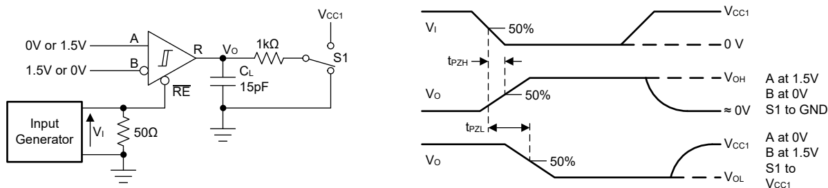
Figure 7-10. Receiver Enable and Disable Times
