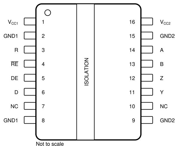
Figure 5-1. DW Package 16-Pin SOIC Full-Duplex Device Top View
