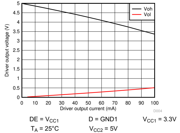
Figure 6-12. Driver Output Voltage Vs Driver Output Current
