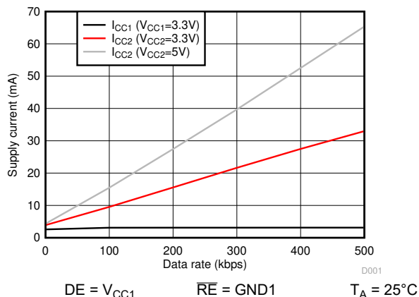
Figure 6-3. ISO141x Supply Current Vs Data Rate- No Load
