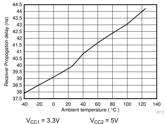
Figure 6-26. ISO145x Receiver Propagation Delay (ns) Vs. Temperature (C)
