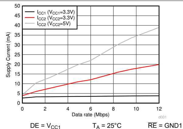
Figure 6-6. ISO143x Supply Current Vs. Data Rate - No Load
