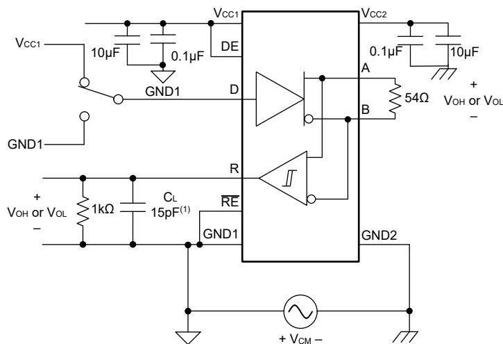
Figure 7-4. Common Mode Transient Immunity (CMTI)—Full Duplex
