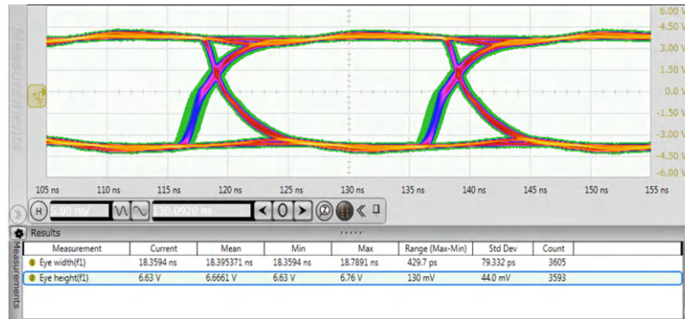
Figure 9-5. Eye Diagram at 50Mbps Clock, V_{CC2} = 5V , 25°C
