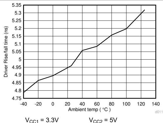
Figure 6-18. ISO145x Driver Rise/Fall Time (ns) Vs Temperature (C)
