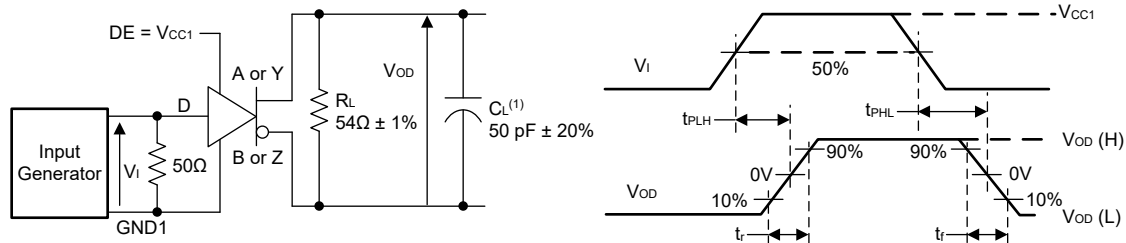
Figure 7-2. Driver Voltages
