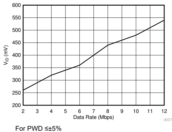
Figure 6-27. ISO143x Receiver V_{ID} vs Signaling Rate
