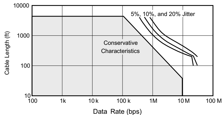
Figure 9-4. Cable Length vs Data Rate Characteristics
