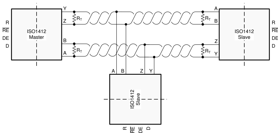
Figure 9-1. Typical RS-485 Network With Full-Duplex Isolated Transceivers
