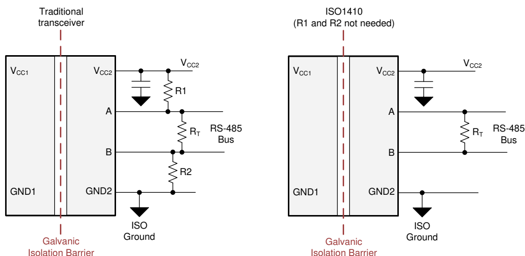
Figure 8-3. Failsafe Transceiver
