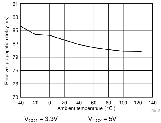
Figure 6-24. ISO141x Receiver Propagation Delay (ns) Vs Temperature (c)
