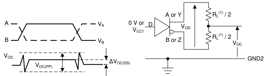
Figure 7-1. Driver Voltages
