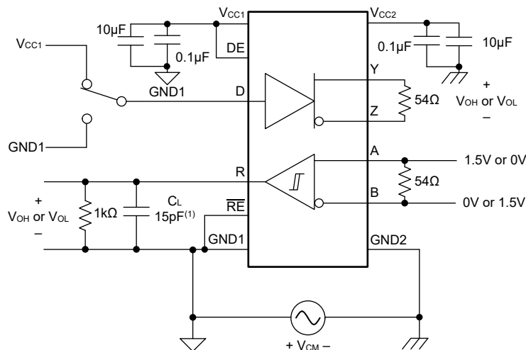
Figure 7-4. Common Mode Transient Immunity (CMTI)—Full Duplex
