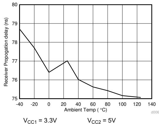
Figure 6-25. ISO143x Receiver Propagation Delay (ns) Vs. Temperature (C)
