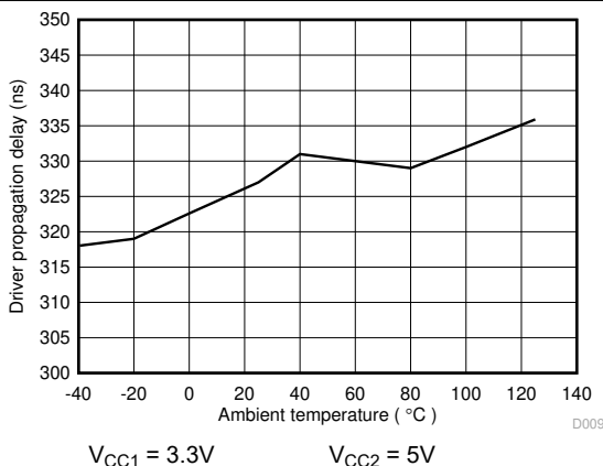
Figure 6-19. ISO141x Driver Propagation Delay (ns) Vs Temperature (c)
