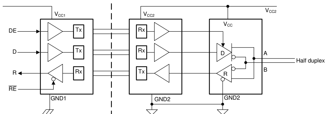
Figure 8-2. Half-Duplex Block Diagram
