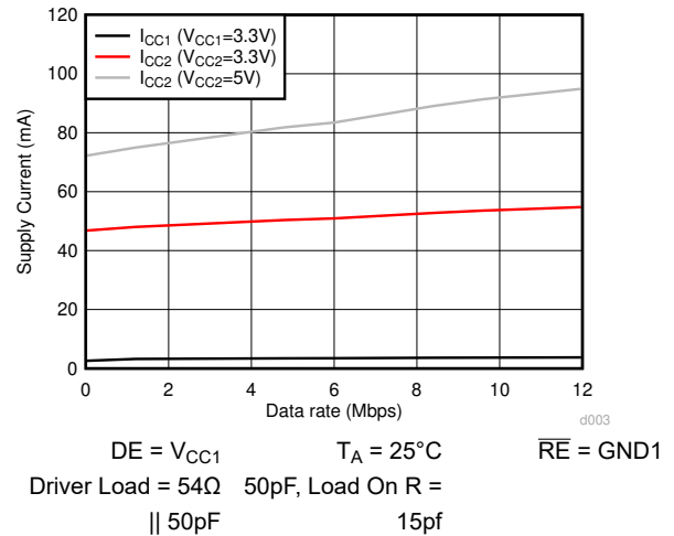
Figure 6-8. ISO143x Supply Current Vs Data Rate- 54Ω||50pF Load
