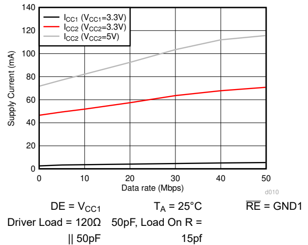
Figure 6-10. ISO145x Supply Current Vs Data Rate- 120Ω||50pF Load
