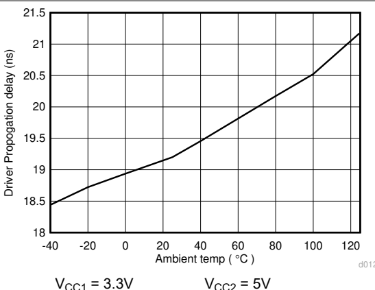
Figure 6-21. ISO145x Driver Propagation Delay (ns) Vs Temperature (C)
