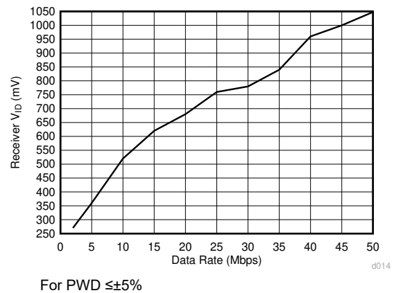
Figure 6-28. ISO145x Receiver V_{ID} vs Signaling Rate
