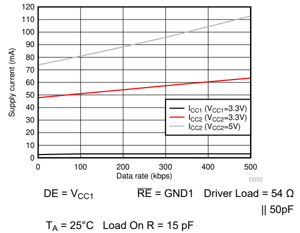
Figure 7-4. ISO141x Supply Current Vs Data Rate- With 54\Omega||50pF Load
