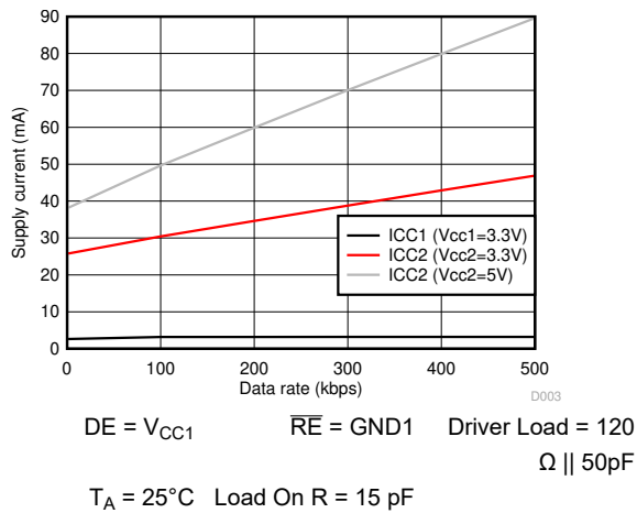
Figure 7-5. ISO141x Supply Current Vs Data Rate- With 120\Omega||50pF Load
