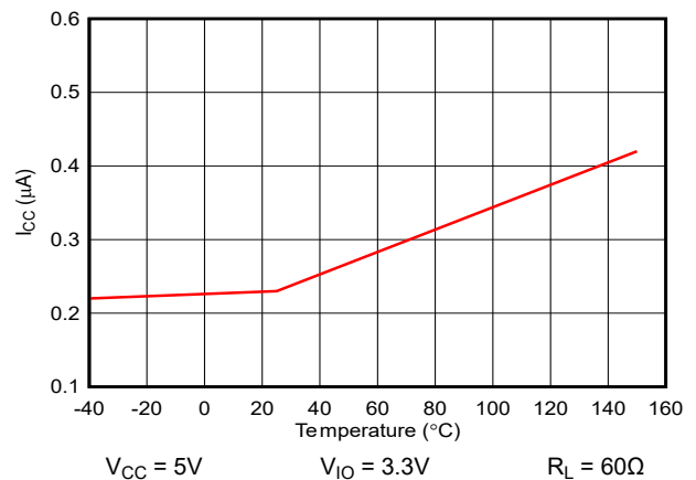
Figure 6-2. I_{CC} Standby (STB) vs Temperature
