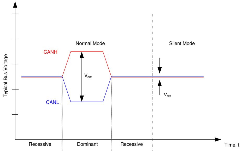
Figure 8-1. Bus States
