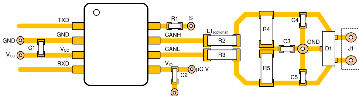
Figure 9-6. Layout Example
