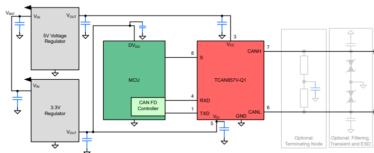
Simplified Schematic
