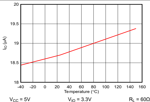
Figure 6-3. I_{IO} Standby (STB) vs Temperature
