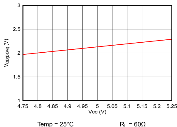
Figure 9-5. V OD(DOM) vs V CC
