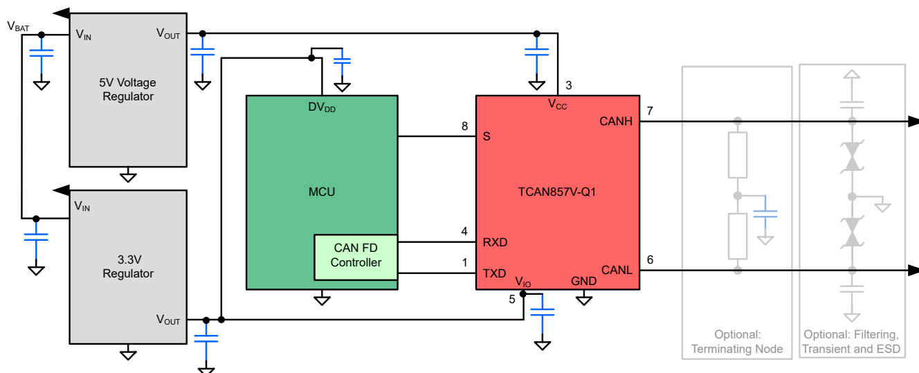
Figure 9-4. Typical Transceiver Application Using 3.3V IO Connections
