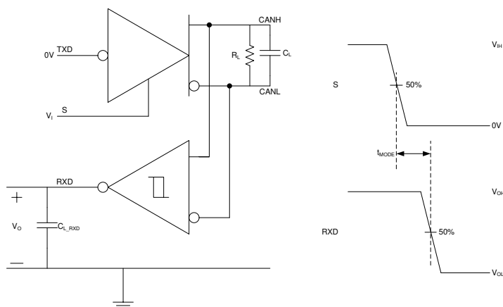
Figure 7-5. t_{MODE} Test Circuit and Measurement
