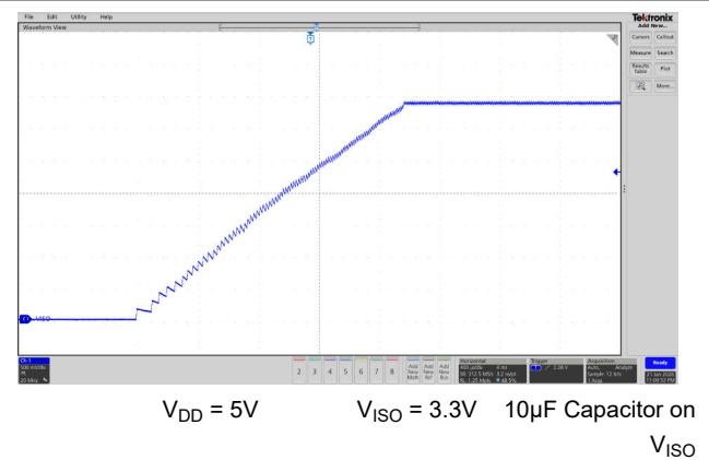
Figure 5-24. Soft Start at 110mA Load For V_{ISO} = 3.3V
