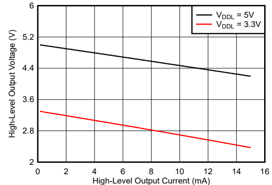
Figure 5-20. High-Level Output Voltage vs High-Level Output Current
