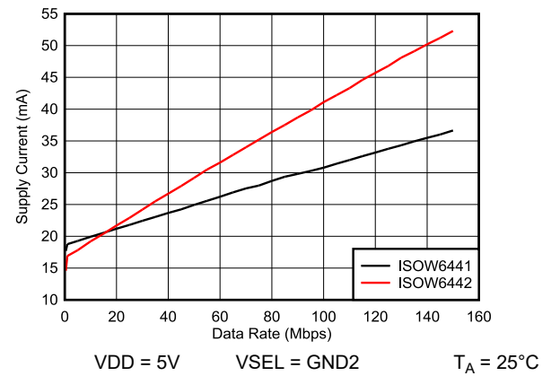
Figure 5-12. Supply Currents ( I_{DD} ) vs Data Rate For C_L = 15\text{pF}
