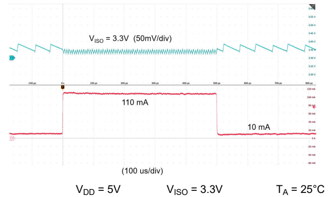
Figure 5-22. 10mA to 110mA Load Transient Response
