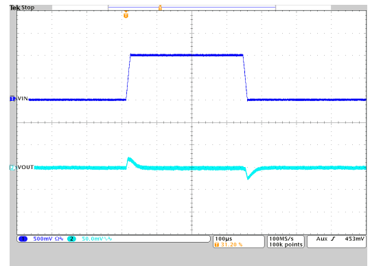
V_{OUT} = 1.8\text{ V} PWM T_A = 25^\circ\text{C} I_{OUT} = 2\text{ A} V_{IN} = 4.5\text{ V to } 5.5\text{ V to } 4.5\text{ V}
