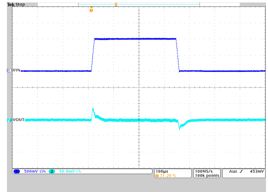
V_{OUT} = 3.3\text{ V} PWM T_A = 25^\circ\text{C} I_{OUT} = 2\text{ A} V_{IN} = 4.5\text{ V to } 5.5\text{ V to } 4.5\text{ V}
