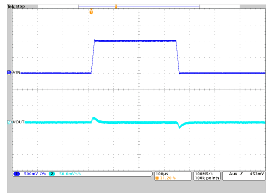
V_{OUT} = 1.2\text{ V} PWM T_A = 25^\circ\text{C} I_{OUT} = 2\text{ A} V_{IN} = 4.5\text{ V to } 5.5\text{ V to } 4.5\text{ V}
