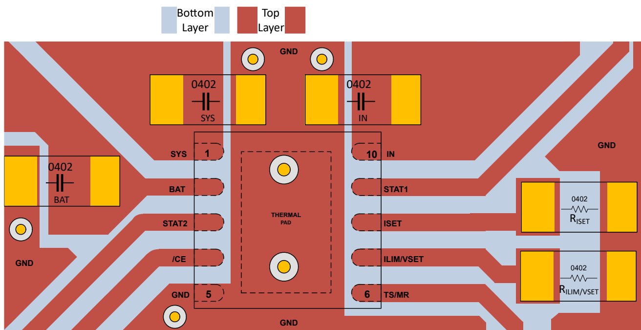
Figure 7-9. Board Layout Example
