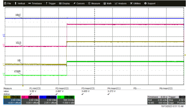
Figure 7-5. Wake Up from Factory Mode with Adapter Insertion
