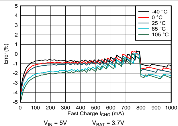
Figure 5-2. Charge Current Accuracy vs I_{CHG} Setting
