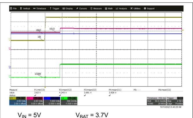
Figure 7-3. Power Up with IN Supply Insertion with Battery
