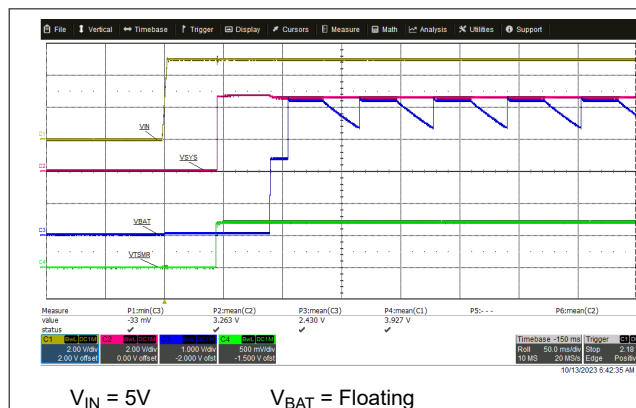
Figure 7-2. Power Up with IN Supply Insertion with No Battery
