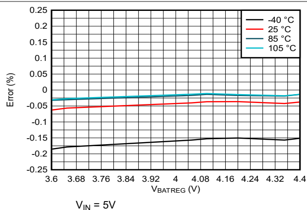
Figure 5-1. Battery Regulation Voltage Accuracy vs V_{BATREG} Setting
