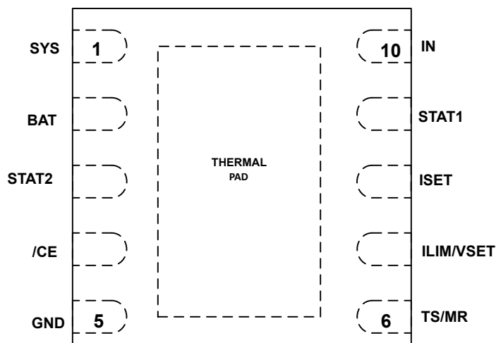
Figure 4-1. DLH Package 10-Pin WSON (Top View)
