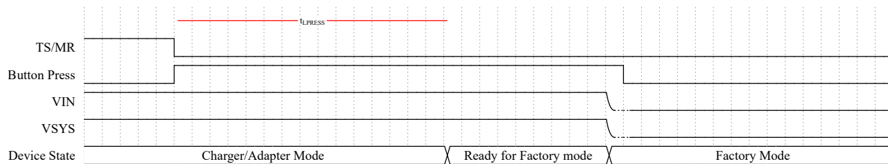
Figure 6-3. Enter Factory Mode
