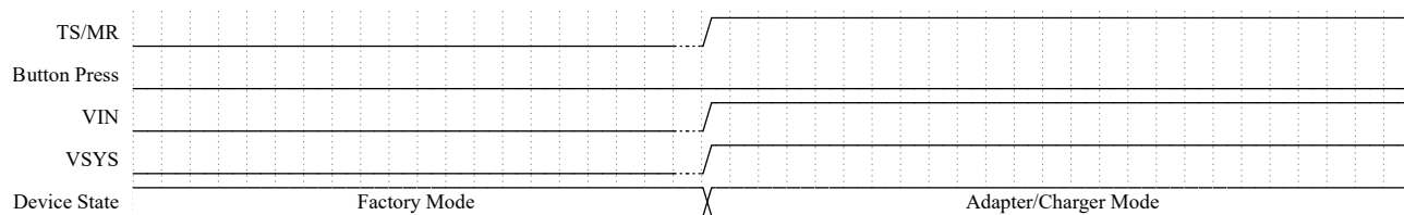
Figure 6-4. Exit Factory Mode
