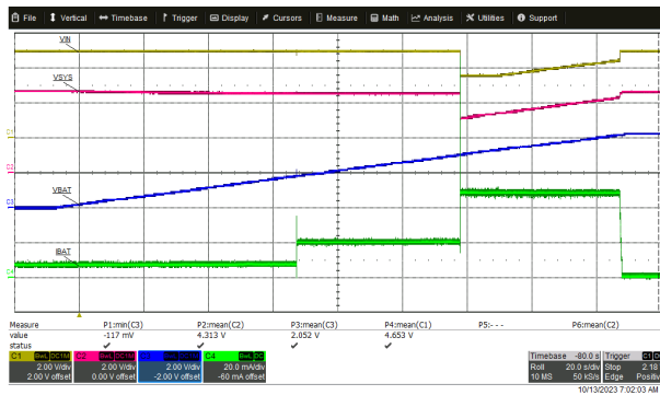
Figure 7-4. Enter Factory Mode
