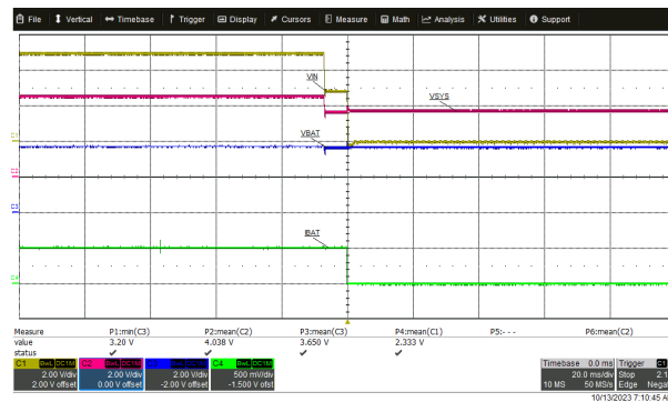
Figure 7-6. Battery Tracking VINDPM
