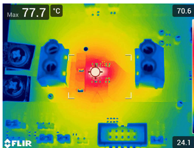
Figure 4-1. Thermal Performance (TPSM8287B30LAPEVM, V_{IN} = 5V , V_{OUT} = 0.6V , I_{OUT} = 30A )
