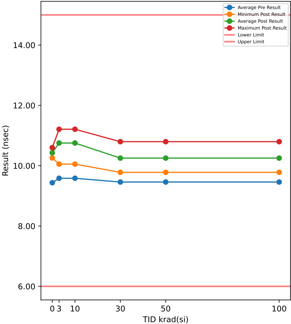
TID vs Result Stats
