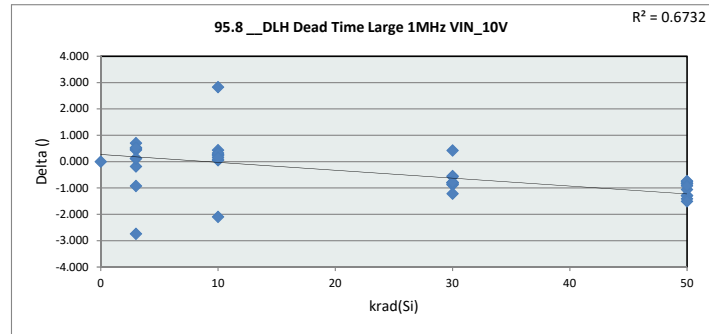
95.8 __DLH Dead Time Large 1MHz VIN_10V
