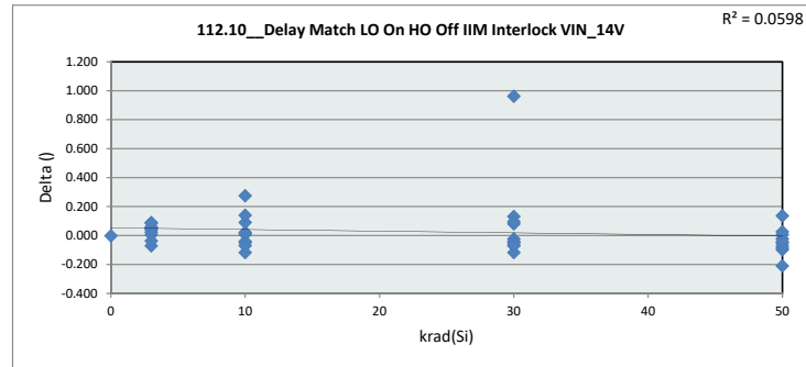
112.10 Delay Match
