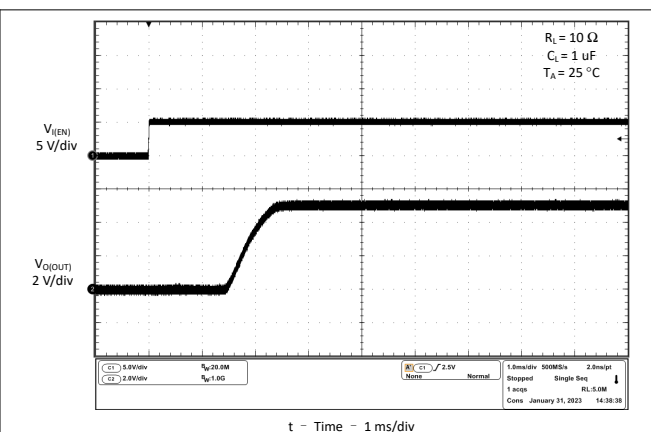
Figure 6-38. Turnon Delay and Rise Time With 1µF Load
