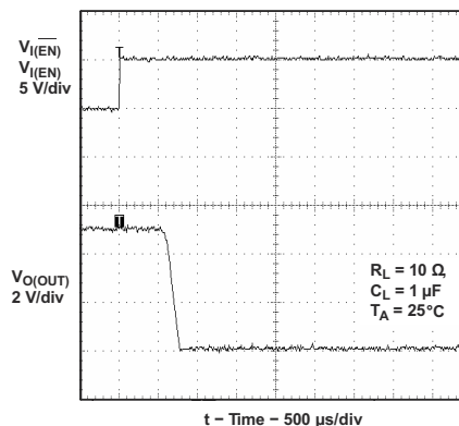
Figure 6-18. Turnoff Delay and Fall Time With 1 \mu\text{F} Load
