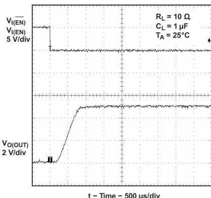
Figure 6-17. Turnon Delay and Rise Time With 1 \mu\text{F} Load
