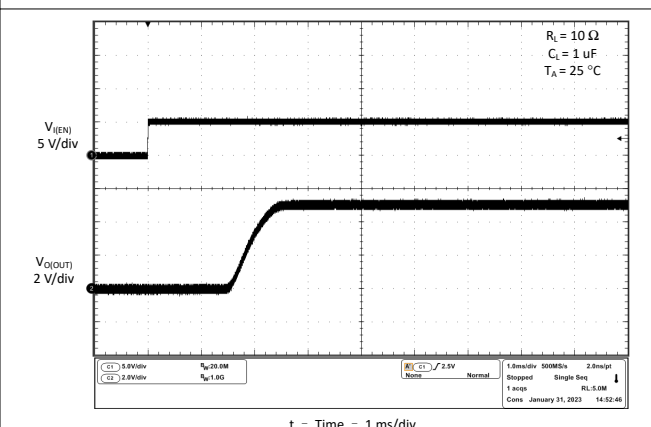
Figure 6-40. Turnon Delay and Rise Time With 100µF Load
