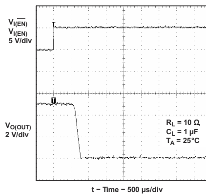
Figure 9-19. Turnoff Delay and Fall Time with 1 \mu F Load
