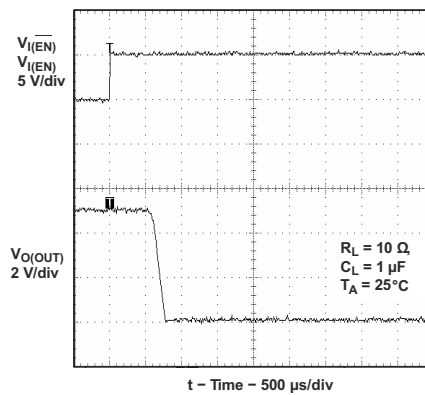
Figure 6-18. Turnoff Delay and Fall Time With 1 \mu\text{F} Load
