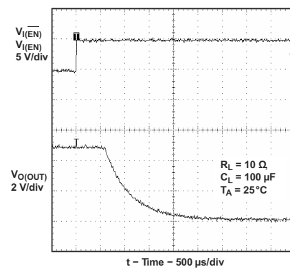
Figure 9-21. Turnoff Delay and Fall Time With 100 \mu F Load
