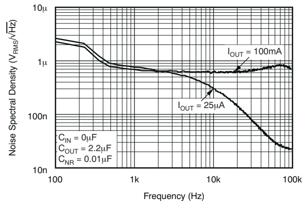
Figure 6-58. Noise Spectral Density vs Frequency (Legacy Device)
