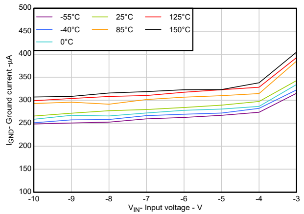
Figure 6-12. Ground Current vs Input Voltage (New Device)
