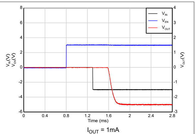
Figure 6-50. Start-up Response ( V_{IN} Ramping After EN) (New Device)
