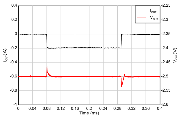
Figure 6-43. Load Transient Response(New Device)
