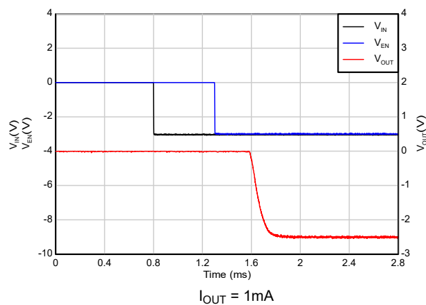
Figure 6-48. Start-up Response ( V_{IN} Ramping Before EN) (New Device)
