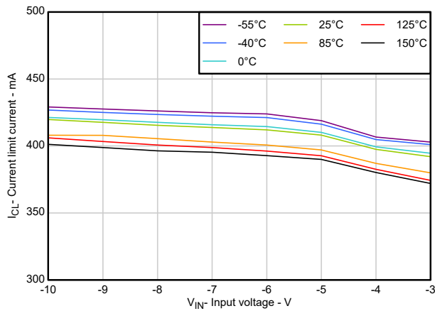
Figure 6-19. Current Limit vs V_{IN} (New Device)
