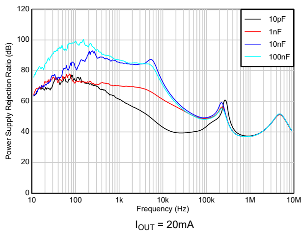
Figure 6-70. PSRR vs C_{NR} (New Device)
