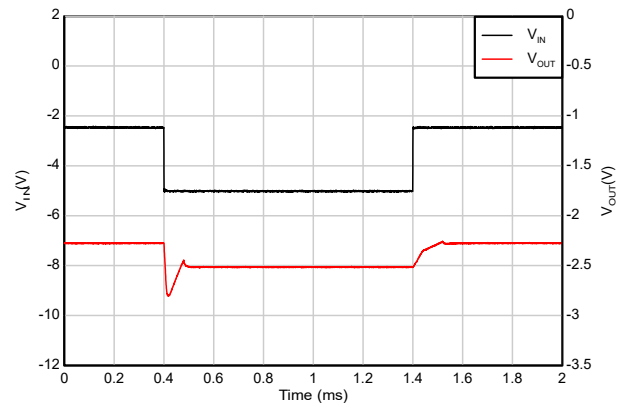
Figure 6-38. Dropout Exit Response (New Device)
