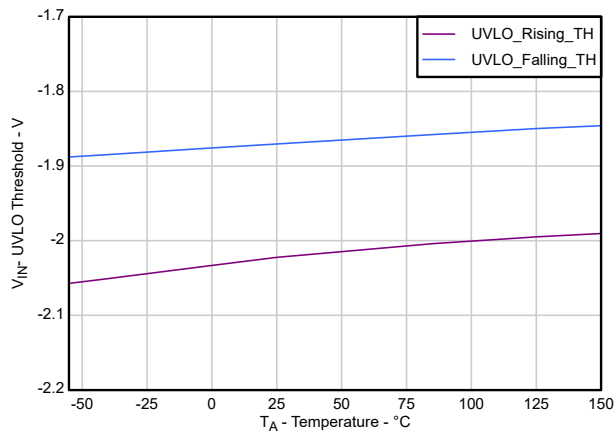
Figure 6-31. UVLO vs Junction Temperature (New Device)
