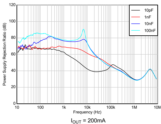
Figure 6-69. PSRR vs C_{NR} (New Device)
