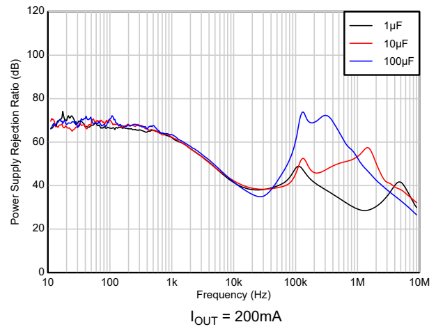
Figure 6-74. PSRR vs C_{OUT} (New Device)
