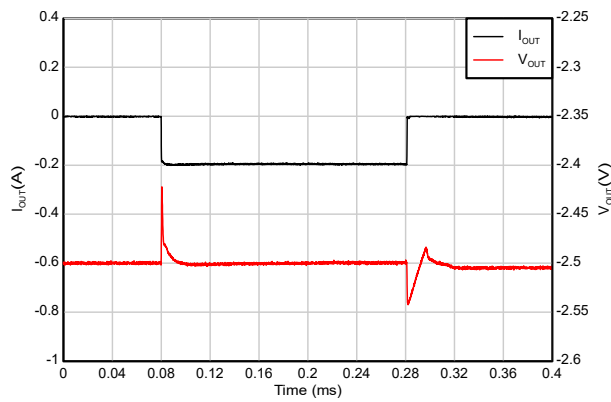
Figure 6-39. Load Transient Response (Legacy Device)
