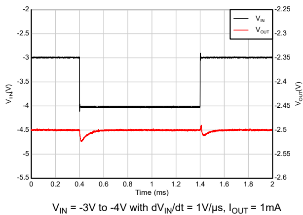
Figure 6-33. Line Transient Response (New Device)
