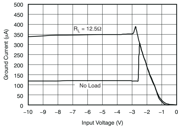
Figure 6-11. Ground Current vs Input Voltage (Legacy Device)
