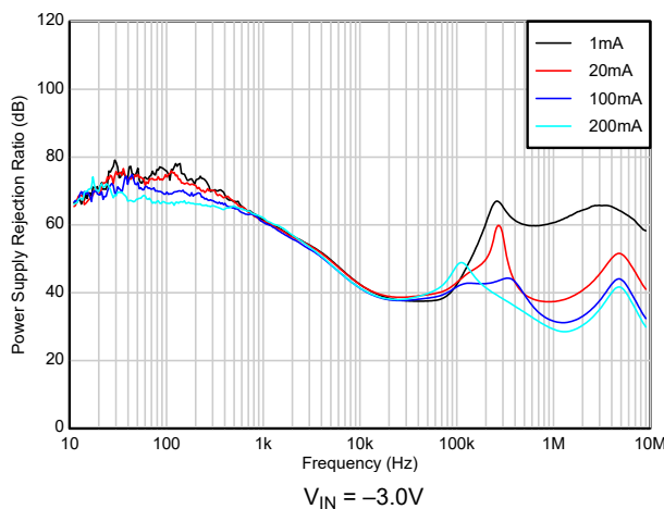
Figure 6-71. PSRR vs I_{OUT} (New Device)
