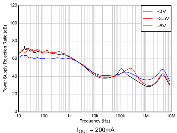
Figure 6-72. PSRR vs V_{IN} (New Device)
