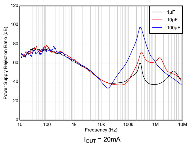
Figure 6-75. PSRR vs C_{OUT} (New Device)
