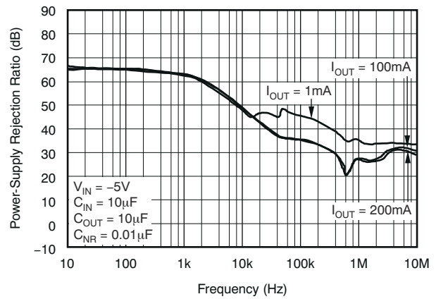
Figure 6-68. PSRR vs Frequency (Legacy Device)
