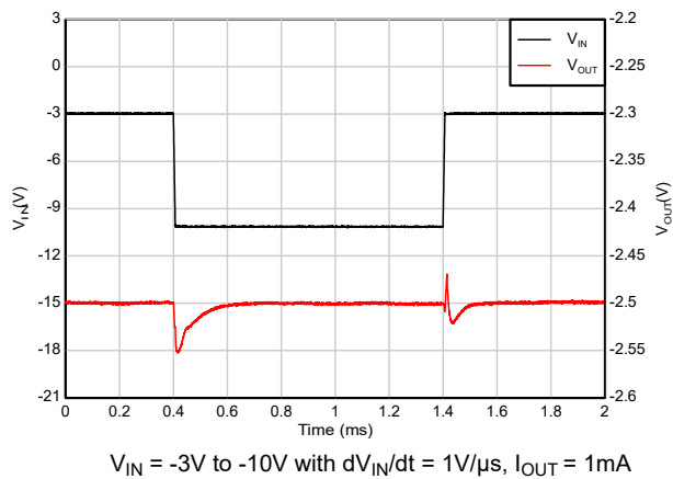
Figure 6-35. Line Transient Response (New Device)
