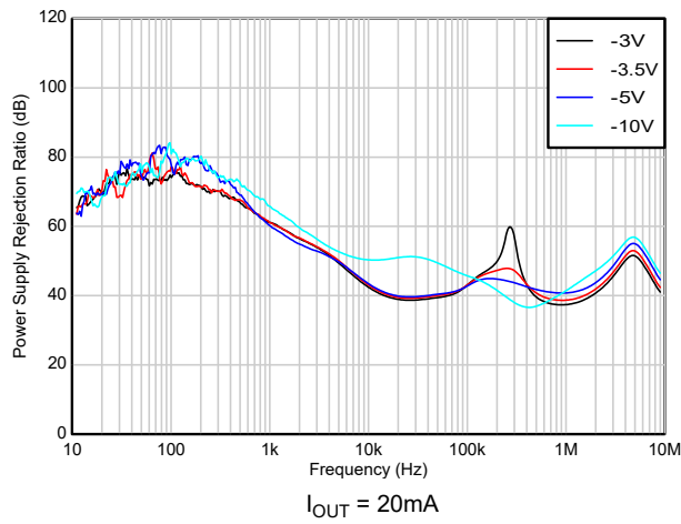
Figure 6-73. PSRR vs V_{IN} (New Device)
