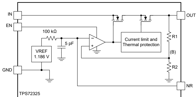
Figure 7-1. Functional Block Diagram (Adjustable, Legacy Chip)
