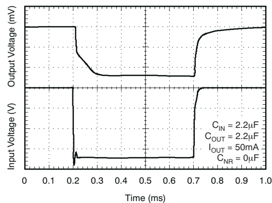
Figure 6-44. Start-Up Response (Legacy Device)
