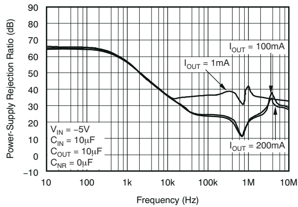
Figure 6-67. PSRR vs Frequency (Legacy Device)
