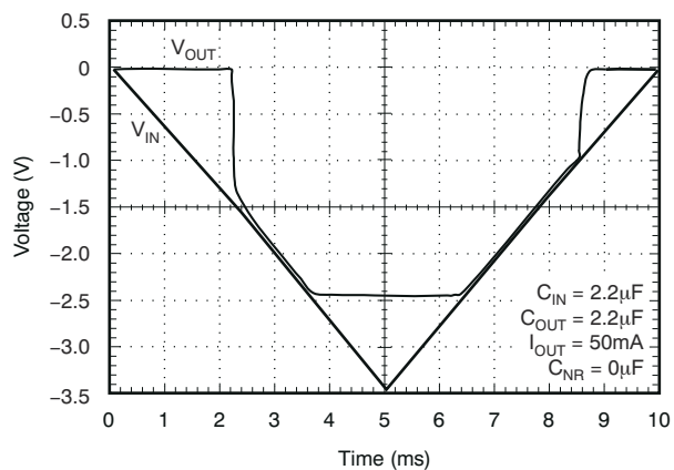
Figure 6-44. Start-Up Response (Legacy Device)
