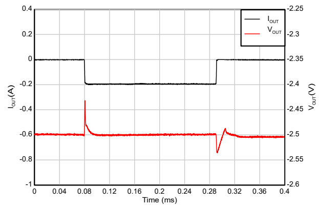
Figure 6-40. Load Transient Response (Legacy Device)
