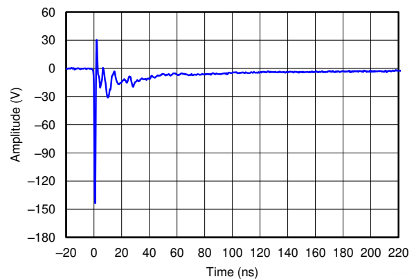
Figure 5-4. IEC 61000-4-2 Clamping Voltage, -8kV Contact
