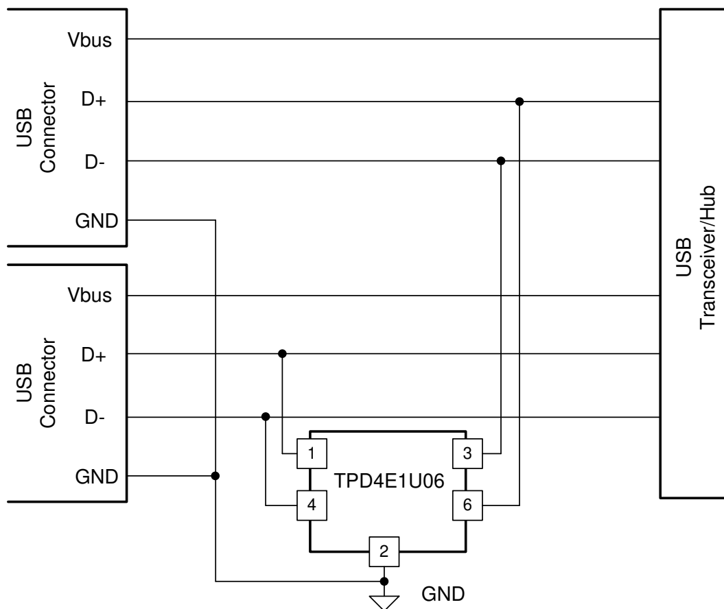
Figure 7-1. Dual USB 2.0 Application
