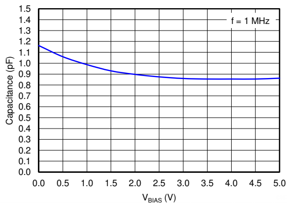
Figure 5-7. Capacitance Across V_{BIAS}
