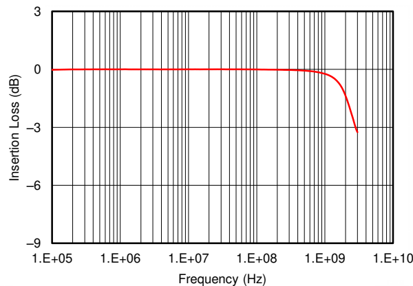
Figure 7-2. Insertion Loss Graph
