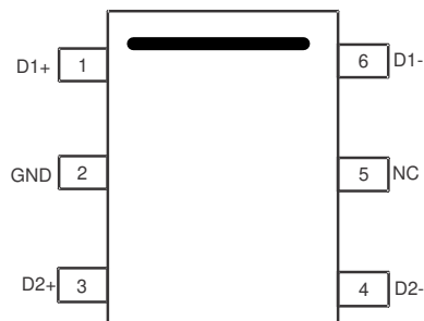
Figure 4-2. DBV Package6-Pin SOT-23Top View
