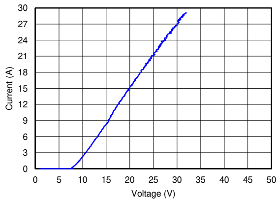
Figure 5-1. TLP, Data to GND
