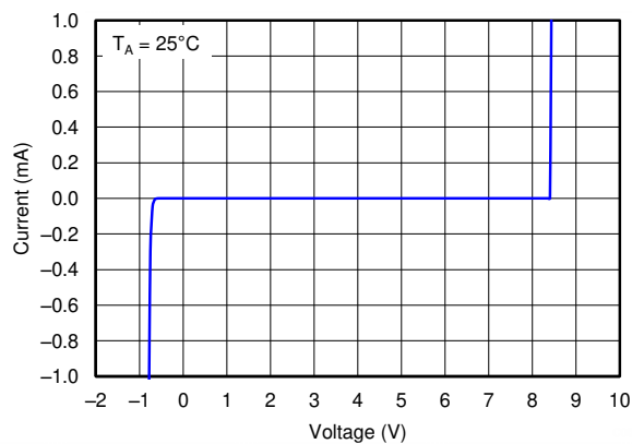
Figure 5-5. Diode Curve
