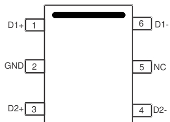
Figure 4-1. DCK Package6-Pin SC70Top View
