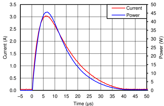
Figure 5-8. Surge Curve ( t_p = 8/20\mu s), Pin IO to GND
