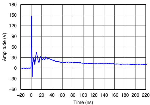
Figure 5-3. IEC 61000-4-2 Clamping Voltage, 8kV Contact
