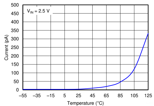
Figure 5-6. I_{LEAK} vs Temperature
