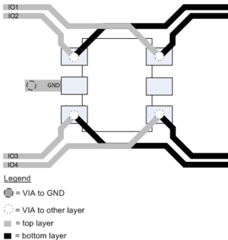
Figure 7-3. PCB Layout Recommendation
