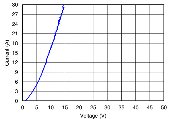
Figure 5-2. TLP, GND to Data
