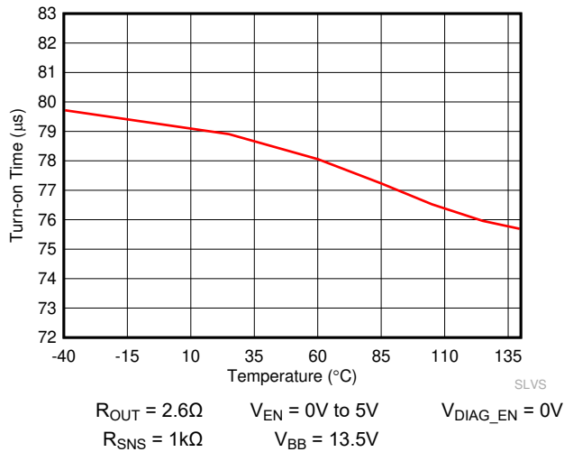
Figure 6-13. Turn-on Time ( t_{\text{ON}} ) vs Temperature
