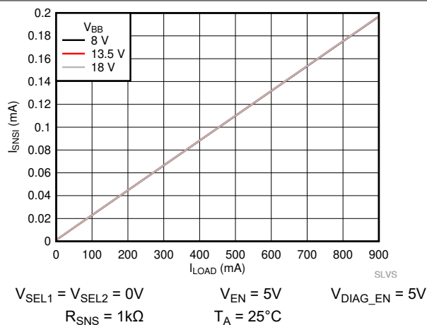
Figure 6-17. Current Sense Output Current ( I_{\text{SNSI}} ) vs Load Current ( I_{\text{OUT}} ) across V_{\text{BB}}
