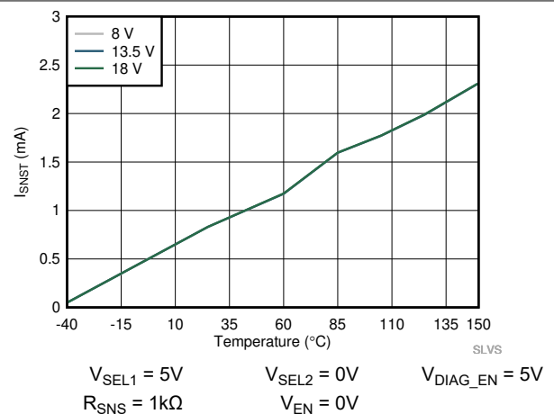
Figure 6-18. Temperature Sense Output Current ( I_{\text{SNSI}} ) vs Temperature
