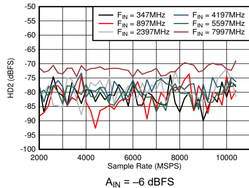
Figure 6-36. DES Mode: HD2 vs Sample Rate and Input Frequency
