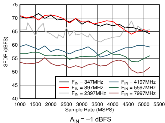
Figure 6-47. Dual Channel Mode: SFDR vs Sample Rate and Input Frequency
