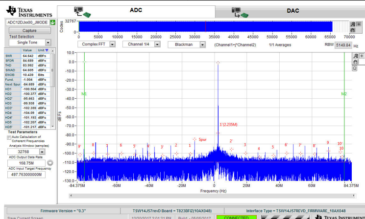
Figure 8-4. FFT for 497.77MHz Input Signal, 2.7GSPS, Decimation-by-16, f_{NCO} = 500MHz, JMODE16
