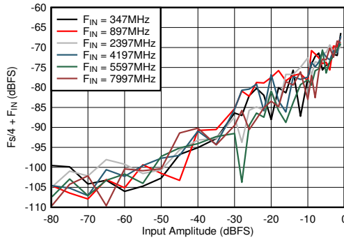
Figure 6-67. DES Mode: \text{Fs}/4 + F_{\text{IN}} vs Input Amplitude and Frequency
