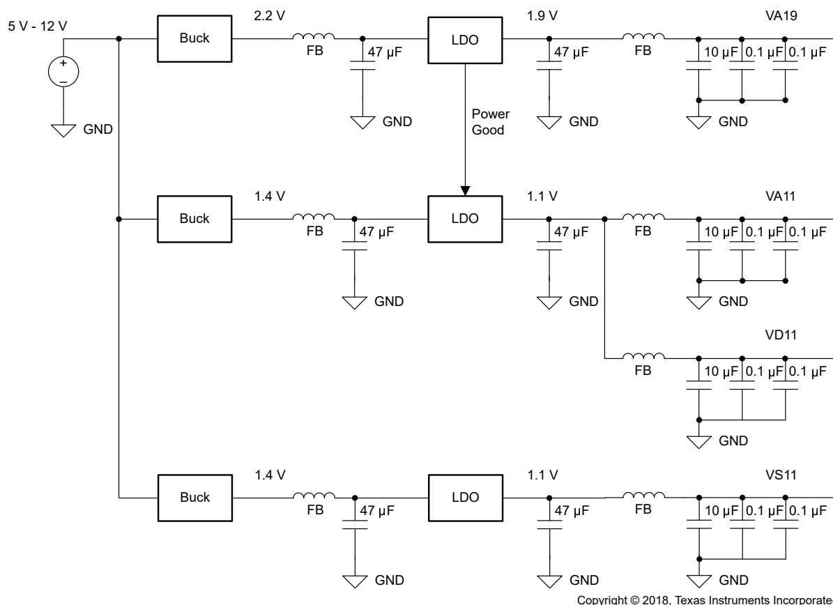
Figure 8-15. LDO Linear Regulator Approach Example (ADC12DJ5210RF)
