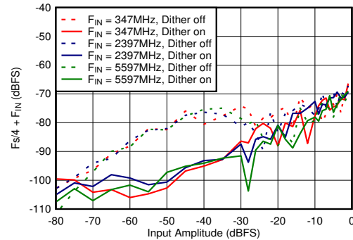
Figure 6-68. DES Mode: \text{Fs}/4 + F_{\text{IN}} vs Input Amplitude and Dither
