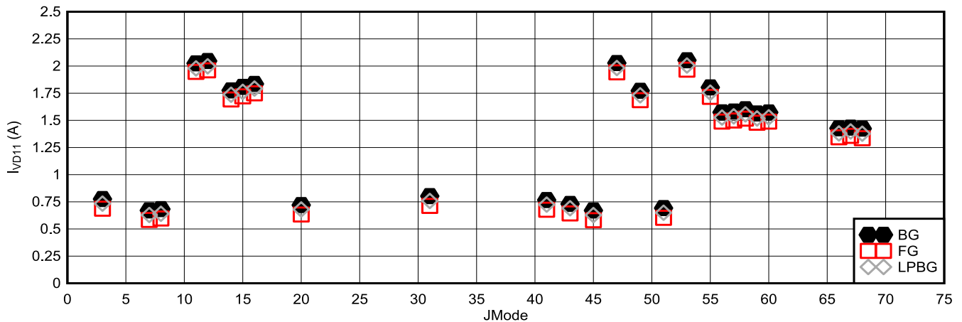
Figure 6-117. Dual Channel Mode: I_{VD11} vs JMODE at 5.2GSPS (ADC12DJ5200RF)
