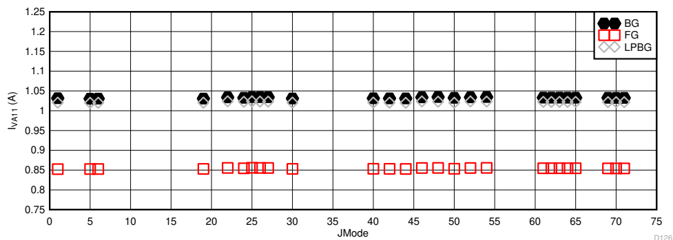
Figure 6-109. DES Mode: I_{VA19} vs JMODE at 10.4GSPS
