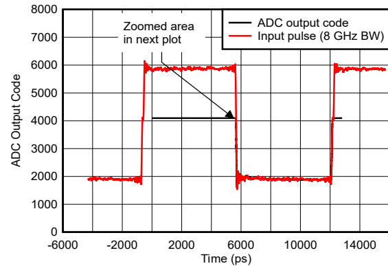
Figure 6-168. Pulse Overdrive Recovery
