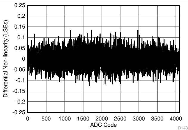
Figure 6-3. DNL vs ADC Code
