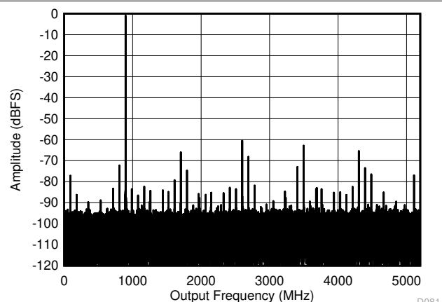
Figure 6-6. DES Mode: Single Tone FFT at 897 MHz
