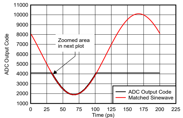
Figure 6-170. Sinewave Overdrive Recovery
