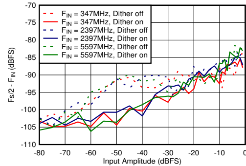
Figure 6-80. Dual Channel Mode: F_s/2 - F_{\text{IN}} vs Input Amplitude and Dither
