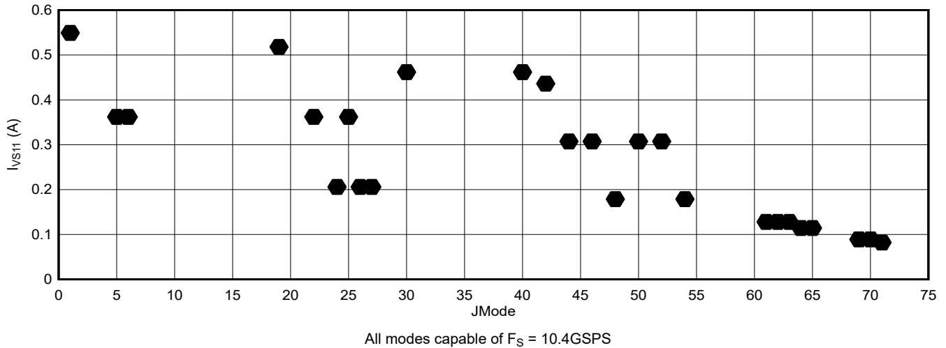
Figure 6-113. DES Mode: I_{VS11} vs JMODE at 10.4GSPS (ADC12DJ5210RF)
