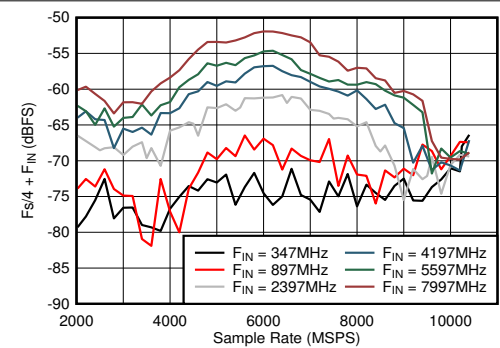
Figure 6-42. DES Mode: F_s/4 + F_{\text{IN}} vs Sample Rate and Input Frequency
