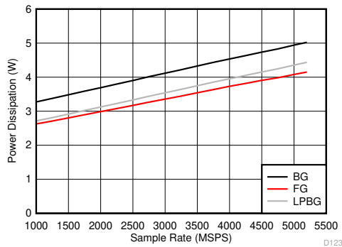
Figure 6-161. Dual Channel Mode: Power Dissipation vs Sample Rate
