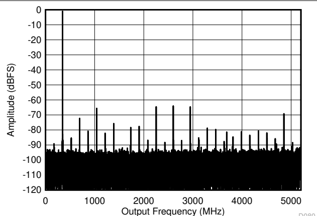
Figure 6-5. DES Mode: Single Tone FFT at 347 MHz
