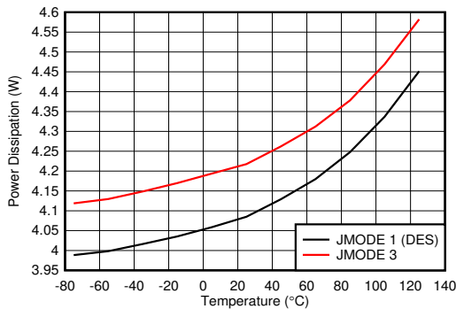
Figure 6-163. Power Dissipation vs Temperature
