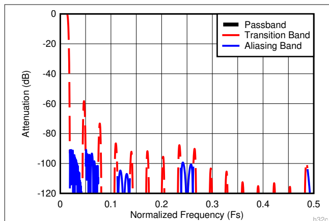
Figure 7-17. Decimate-by-32 Composite Response
