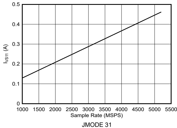
Figure 6-155. Dual Channel Mode: I_{VS11} vs Sample Rate (ADC12DJ5210RF)
