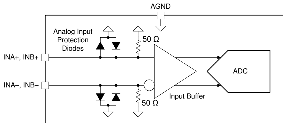
Figure 7-1. ADC12DJ52x0RF Analog Input Internal Termination and Protection Diagram
