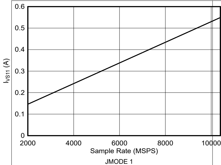
Figure 6-131. DES Mode: I_{VS11} vs Sample Rate (ADC12DJ5210RF)
