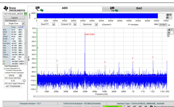
Figure 8-3. FFT for 497.77MHz Input Signal, 2.7GSPS, JMODE2
