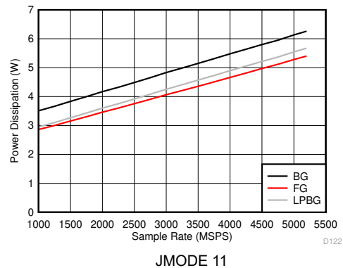
Figure 6-160. Dual Channel Mode: Power Dissipation vs Sample Rate
