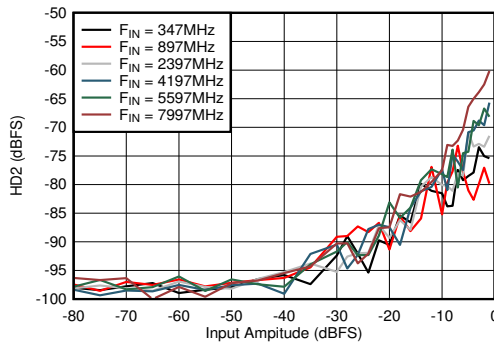
Figure 6-75. Dual Channel Mode: HD2 vs Input Amplitude and Frequency
