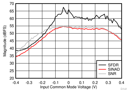
Figure 6-97. SNR, SFDR and SINAD vs Input Common Mode Voltage
