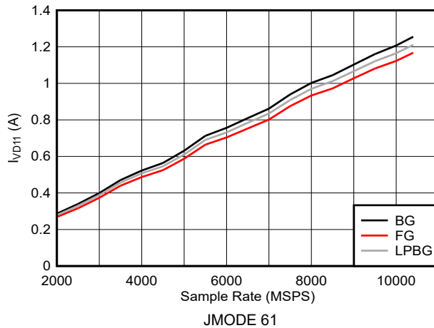
Figure 6-139. DES Mode: I_{VD11} vs Sample Rate (ADC12DJ5210RF)
