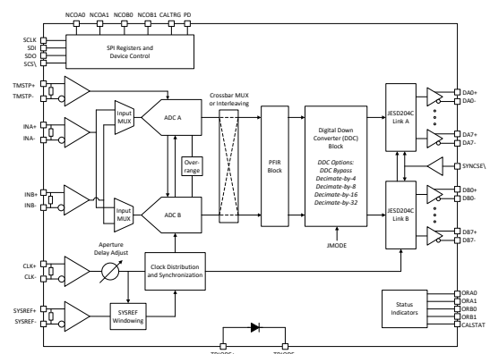
ADC12DJ52x0RF Block Diagram
