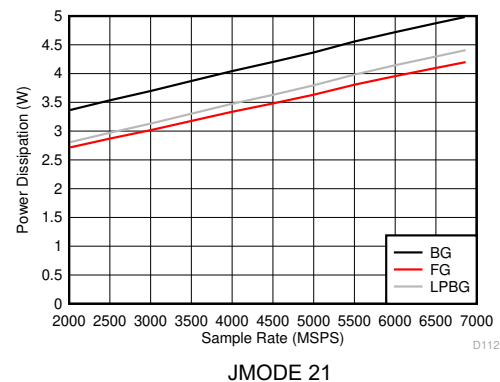
Figure 6-142. DES Mode: Power Dissipation vs Sample Rate
