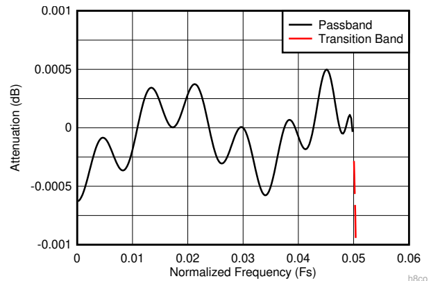
Figure 7-14. Decimate-by-8 Composite Zoomed Pass-Band Response
