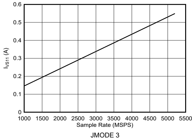
Figure 6-149. Dual Channel Mode: I_{VS11} vs Sample Rate (ADC12DJ5210RF)
