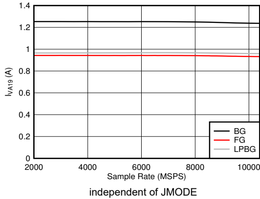
Figure 6-127. DES Mode: I_{VA19} vs Sample Rate
