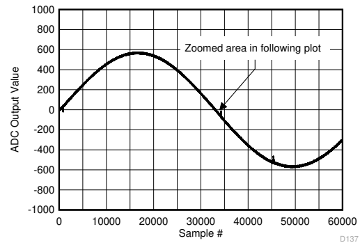
Figure 6-164. Background Calibration Core Transition (AC Signal)
