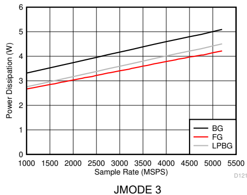
Figure 6-159. Dual Channel Mode: Power Dissipation vs Sample Rate
