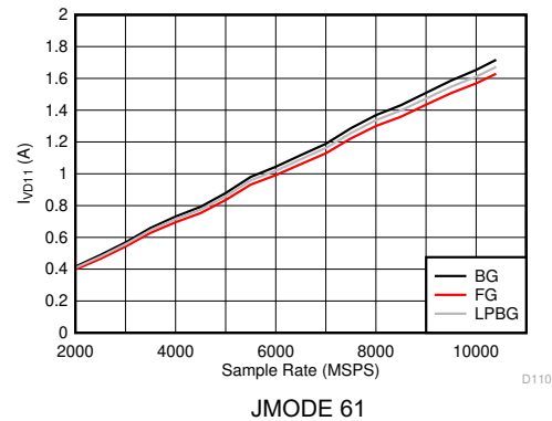
Figure 6-138. DES Mode: I_{VD11} vs Sample Rate (ADC12DJ5200RF)
