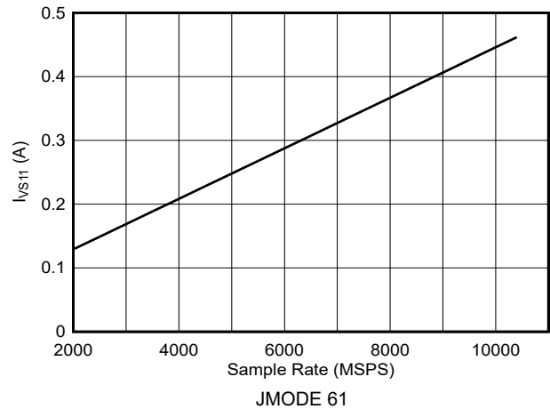
Figure 6-140. DES Mode: I_{VS11} vs Sample Rate (ADC12DJ5210RF)
