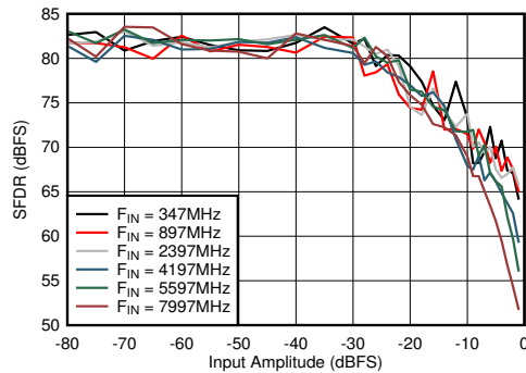
Figure 6-73. Dual Channel Mode: SFDR vs Input Amplitude and Frequency
