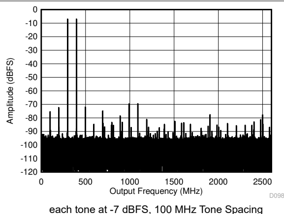
Figure 6-23. Dual Channel Mode: Two Tone FFT at 347 MHz
