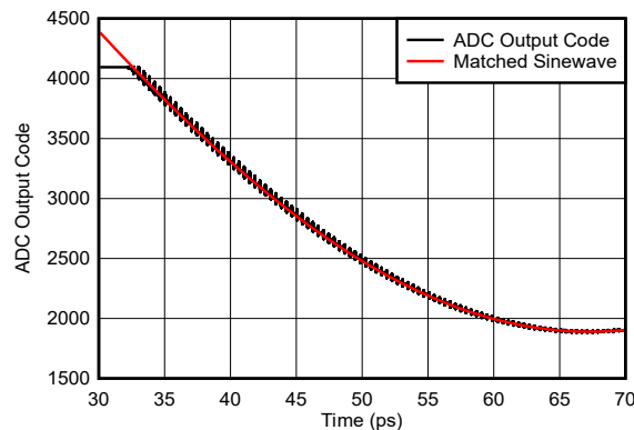
Figure 6-171. Sinewave Overdrive Recovery
