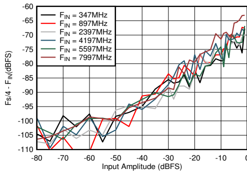
Figure 6-69. DES Mode: F_s/4 - F_{\text{IN}} vs Input Amplitude and Frequency
