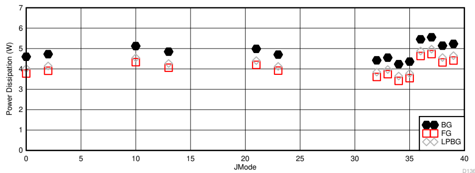
Figure 6-125. Other Modes with Lower Maximum F_S : I_{VS11} vs JMODE (ADC12DJ5210RF)
