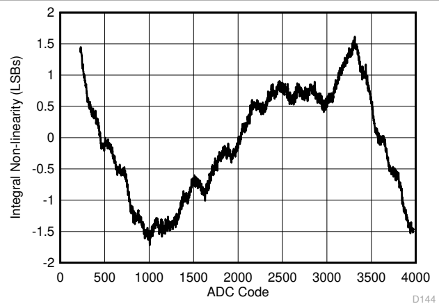
Figure 6-4. INL vs ADC Code
