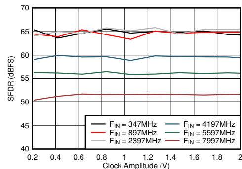
Figure 6-84. Dual Channel Mode: SFDR vs Clock Amplitude
