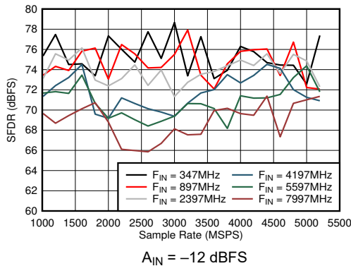
Figure 6-49. Dual Channel Mode: SFDR vs Sample Rate and Input Frequency
