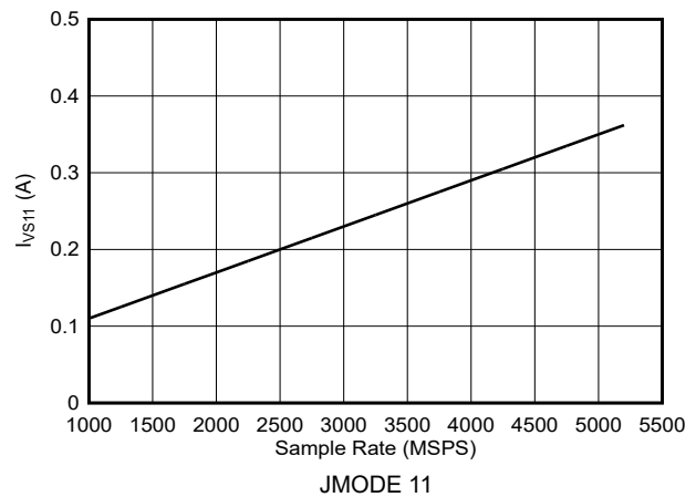
Figure 6-152. Dual Channel Mode: I_{VD11} vs Sample Rate (ADC12DJ5200RF)
