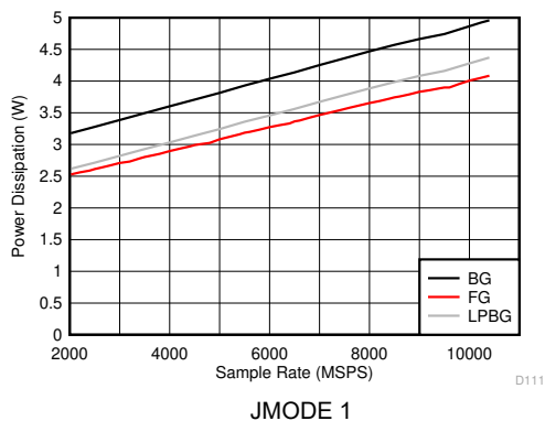
Figure 6-141. DES Mode: Power Dissipation vs Sample Rate
