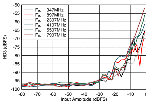
Figure 6-77. Dual Channel Mode: HD3 vs Input Amplitude and Frequency
