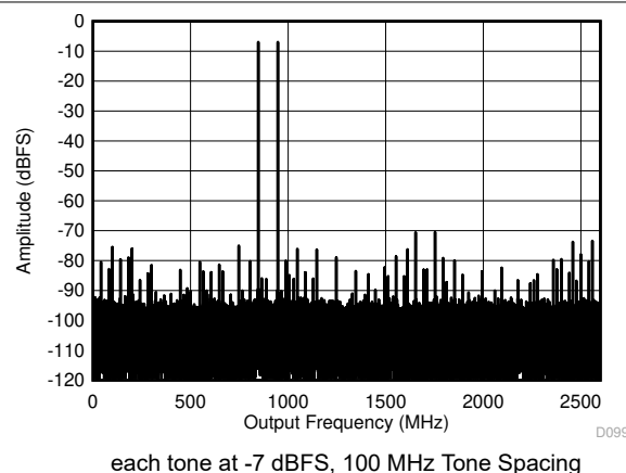
Figure 6-24. Dual Channel Mode: Two Tone FFT at 897 MHz
