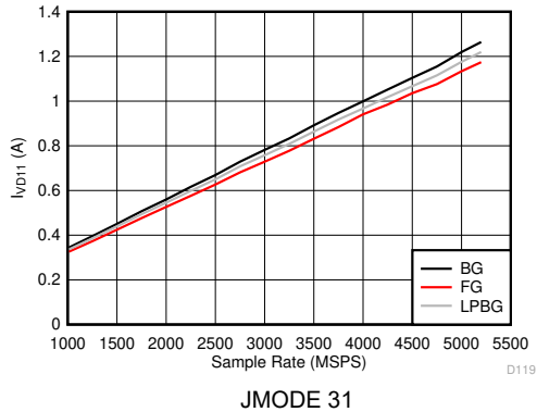
Figure 6-153. Dual Channel Mode: I_{VD11} vs Sample Rate (ADC12DJ5200RF)
