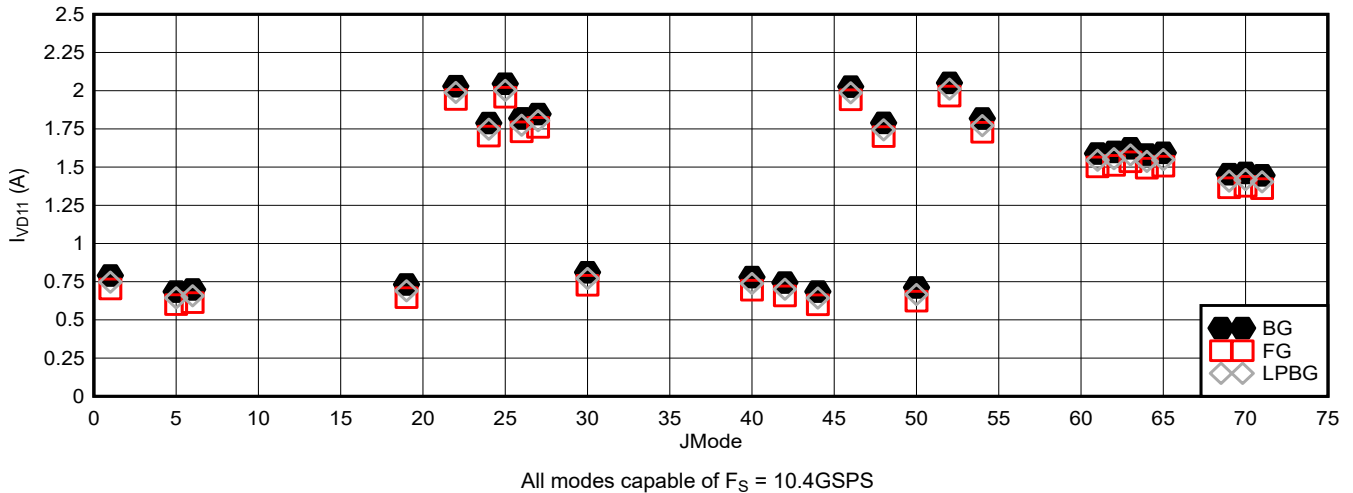
Figure 6-111. DES Mode: I_{VD11} vs JMODE at 10.4GSPS (ADC12DJ5200RF)
