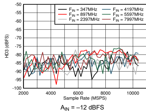
Figure 6-40. DES Mode: HD3 vs Sample Rate and Input Frequency
