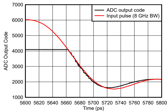
Figure 6-169. Pulse Overdrive Recovery Zoomed
