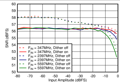
Figure 6-72. Dual Channel Mode: SNR vs Input Amplitude and Dither
