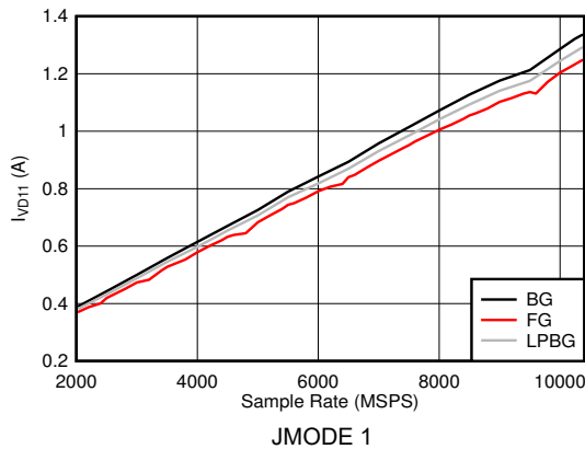
Figure 6-129. DES Mode: I_{VD11} vs Sample Rate (ADC12DJ5200RF)
