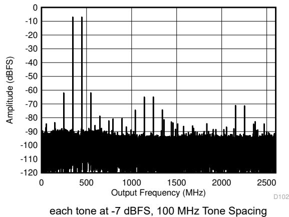
Figure 6-27. Dual Channel Mode: Two Tone FFT at 5597 MHz
