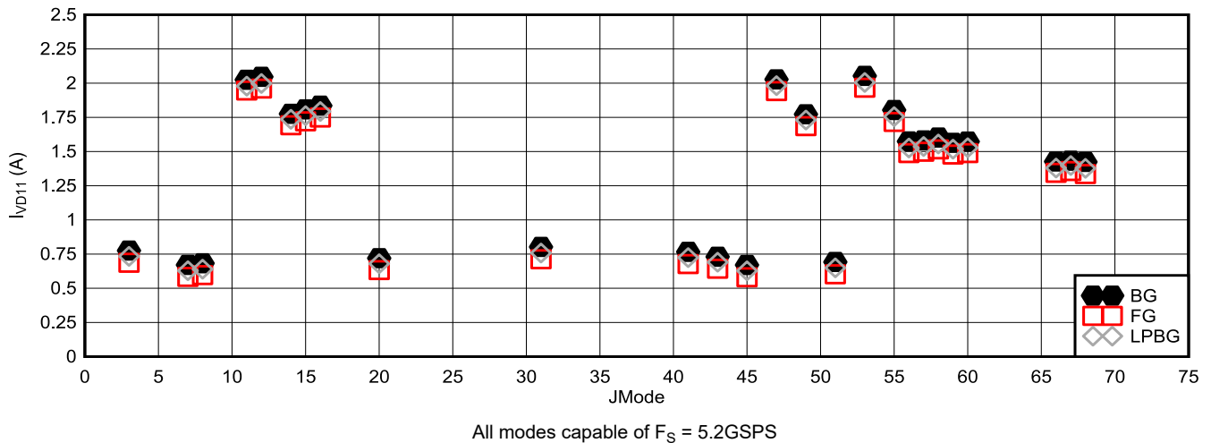
Figure 6-117. Dual Channel Mode: I_{VD11} vs JMODE at 5.2GSPS (ADC12DJ5200RF)
