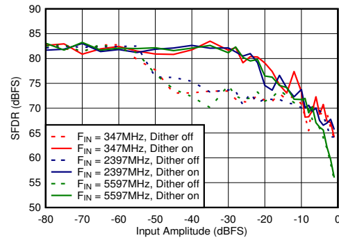
Figure 6-74. Dual Channel Mode: SFDR vs Input Amplitude and Dither
