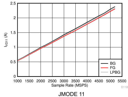
Figure 6-150. Dual Channel Mode: I_{VD11} vs Sample Rate (ADC12DJ5200RF)
