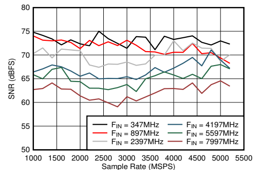
Figure 6-46. Dual Channel Mode: SNR vs Sample Rate and Input Frequency
