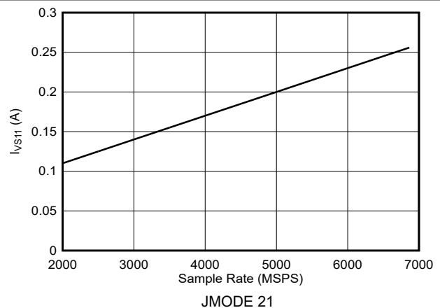
Figure 6-134. DES Mode: I_{VS11} vs Sample Rate (ADC12DJ5210RF)
