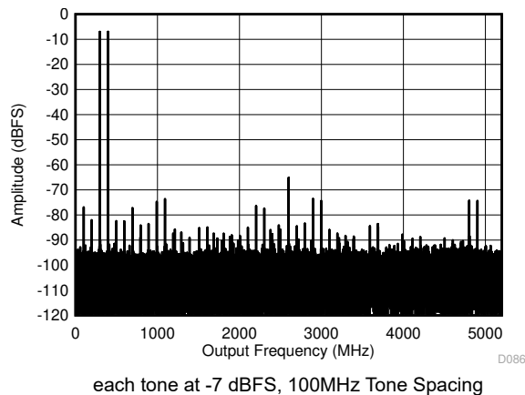
Figure 6-11. DES Mode: Two Tone FFT at 347 MHz
