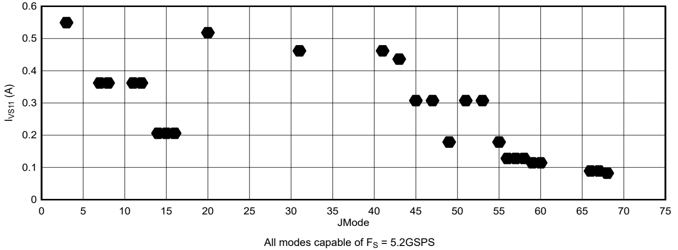
Figure 6-119. Dual Channel Mode: I_{VS11} vs JMODE at 5.2GSPS (ADC12DJ5210RF)
