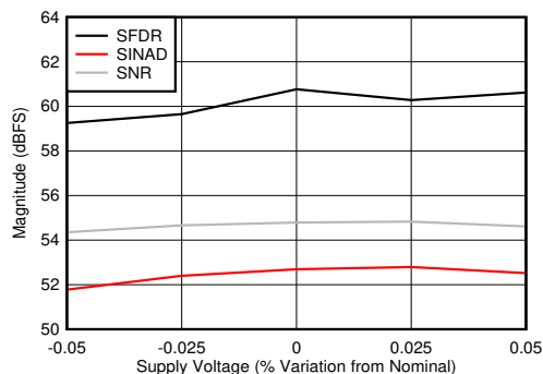
Figure 6-93. DES Mode: SNR, SINAD and SFDR vs Supply Voltage
