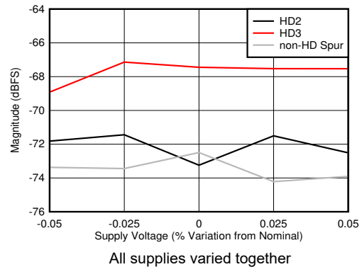
Figure 6-96. Dual Channel Mode: HD2, HD3 and Worst non-HD Spur vs Supply Voltage
