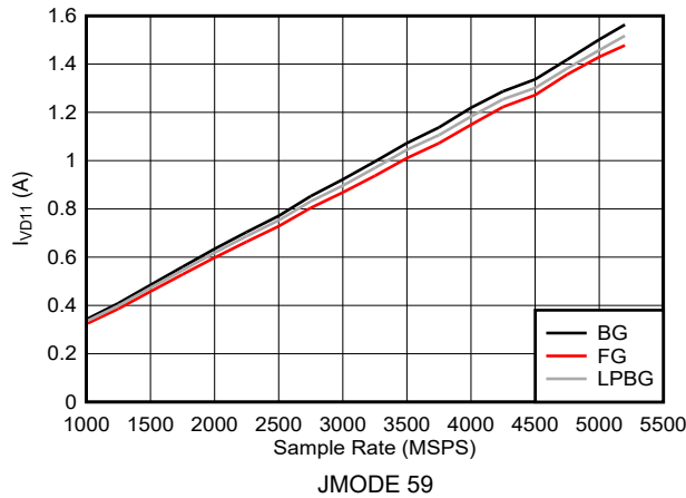
Figure 6-157. Dual Channel Mode: I_{VD11} vs Sample Rate (ADC12DJ5210RF)
