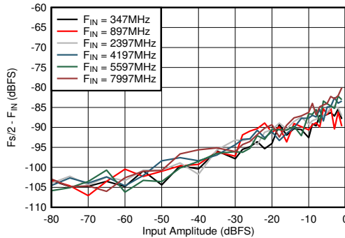
Figure 6-79. Dual Channel Mode: F_s/2 - F_{\text{IN}} vs Input Amplitude and Frequency
