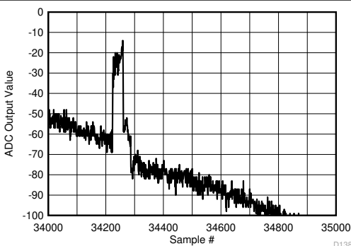
Figure 6-165. Background Calibration Core Transition (AC Signal - zoomed)
