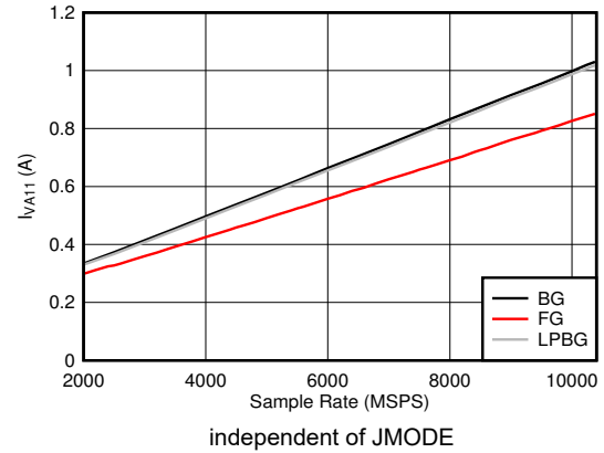
Figure 6-128. DES Mode: I_{VA11} vs Sample Rate
