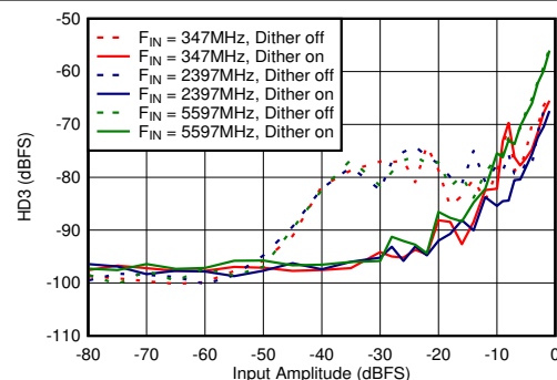
Figure 6-78. Dual Channel Mode: HD3 vs Input Amplitude and Dither
