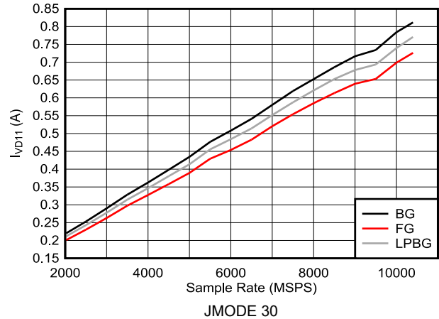
Figure 6-136. DES Mode: I_{VD11} vs Sample Rate (ADC12DJ5210RF)
