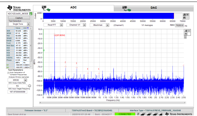
Figure 8-9. 200MHz, Sine-Wave Frequency Domain (FFT) for 5GSPS, Single-Channel Oscilloscope
