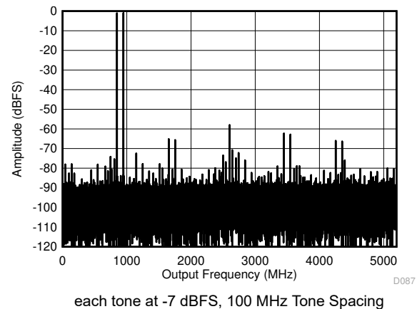
Figure 6-12. DES Mode: Two Tone FFT at 897 MHz
