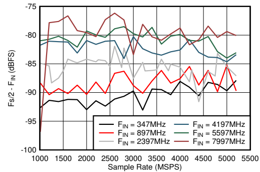
Figure 6-56. Dual Channel Mode: F_s/2 - F_{\text{IN}} vs Sample Rate and Input Frequency
