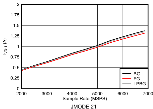
Figure 6-133. DES Mode: I_{VD11} vs Sample Rate (ADC12DJ5210RF)
