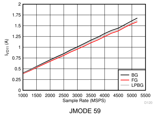
Figure 6-156. Dual Channel Mode: I_{VD11} vs Sample Rate (ADC12DJ5200RF)
