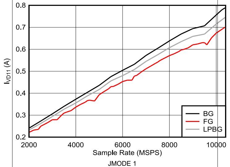
Figure 6-130. DES Mode: I_{VD11} vs Sample Rate (ADC12DJ5210RF)
