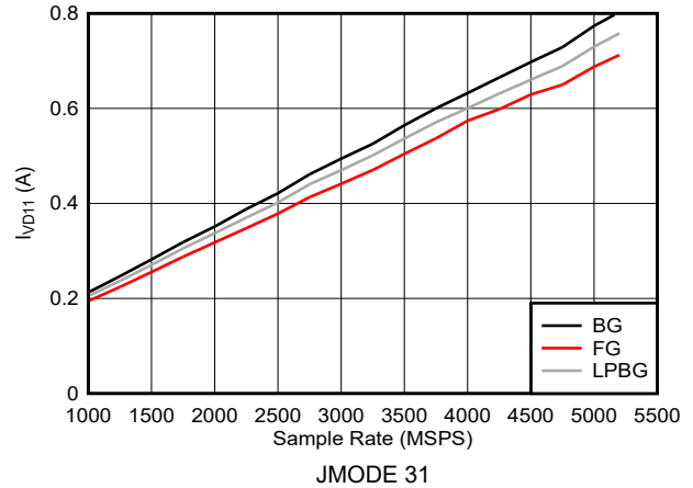
Figure 6-154. Dual Channel Mode: I_{VD11} vs Sample Rate (ADC12DJ5210RF)
