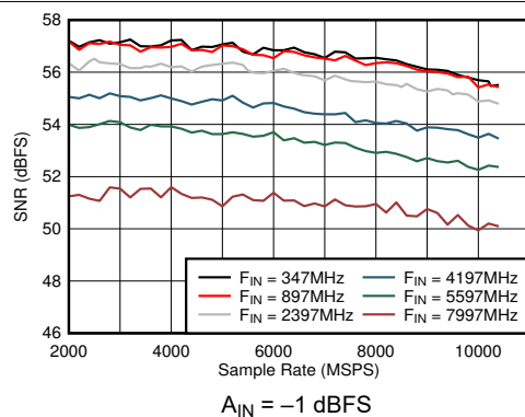
Figure 6-29. DES Mode: SNR vs Sample Rate and Input Frequency
