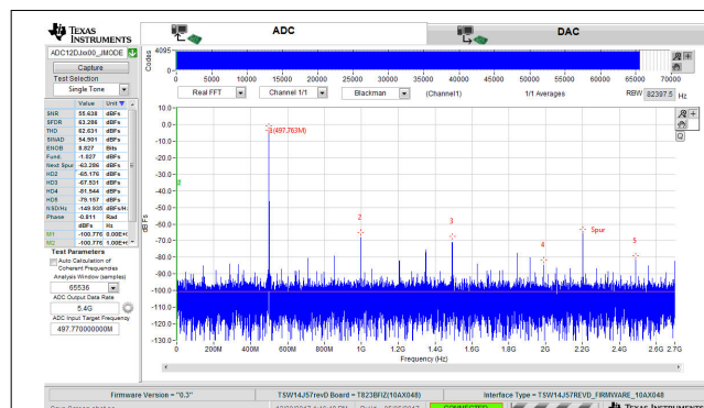
Figure 8-2. FFT for 497.77MHz Input Signal, 5.4GSPS, JMODE0
