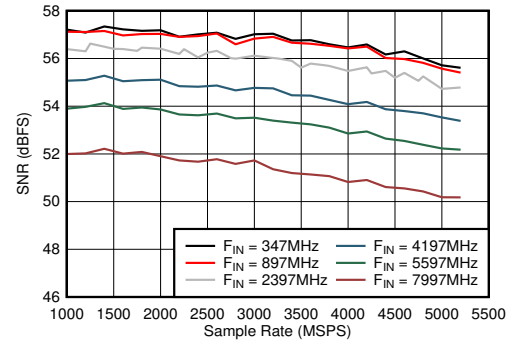
Figure 6-44. Dual Channel Mode: SNR vs Sample Rate and Input Frequency
