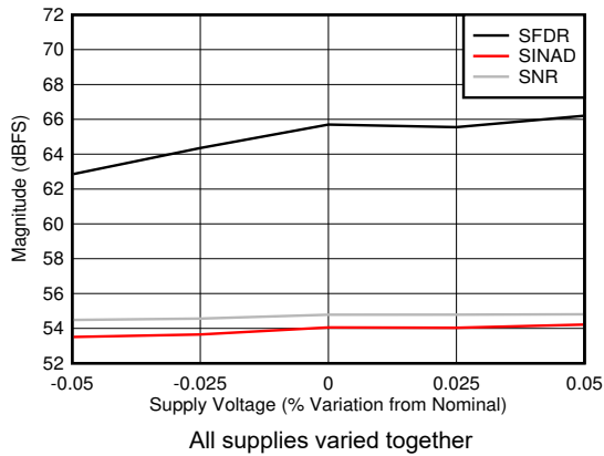
Figure 6-95. Dual Channel Mode: SNR, SINAD and SFDR vs Supply Voltage
