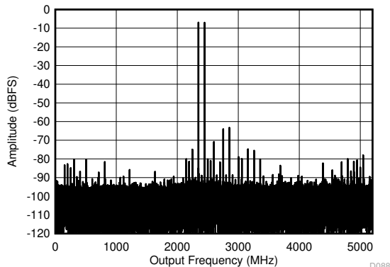
Figure 6-13. DES Mode: Two Tone FFT at 2397 MHz
