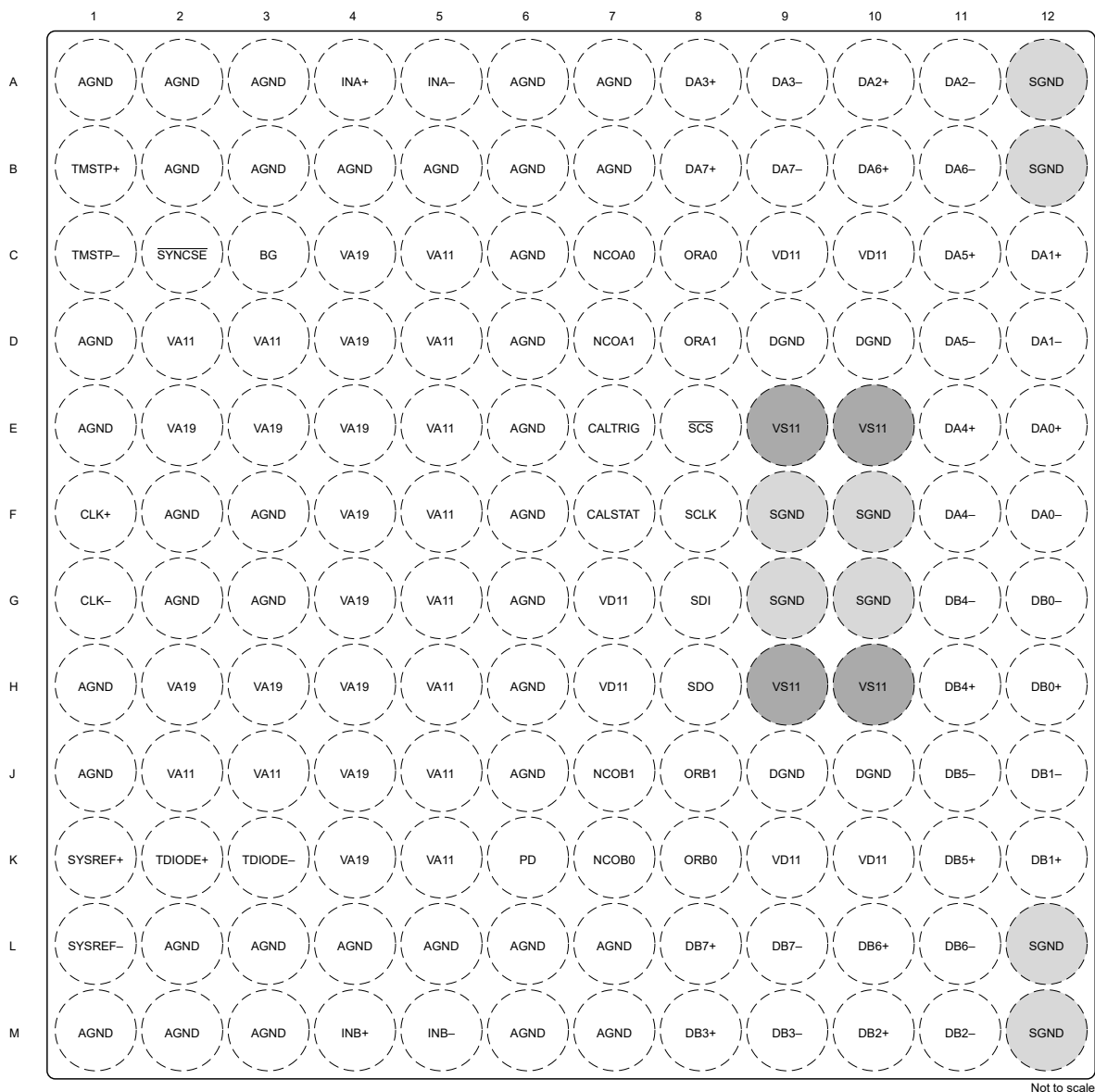
Figure 5-2. ADC12DJ5210RF AAV Package, 144-Ball Flip Chip BGA Top View
