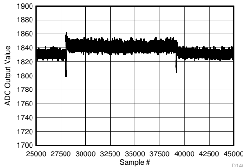
Figure 6-167. Background Calibration Core Transition (DC Signal - zoomed)
