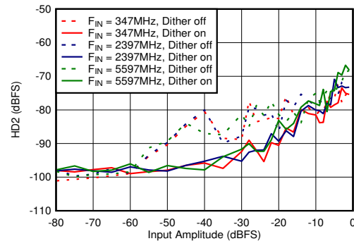
Figure 6-76. Dual Channel Mode: HD2 vs Input Amplitude and Dither
