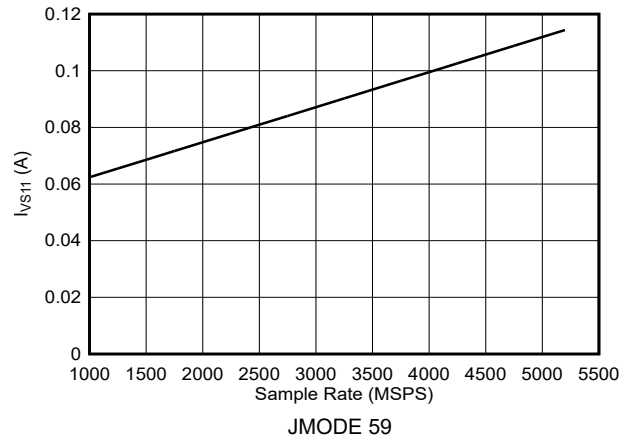
Figure 6-158. Dual Channel Mode: I_{VS11} vs Sample Rate (ADC12DJ5210RF)
