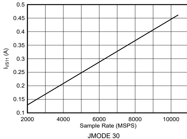
Figure 6-137. DES Mode: I_{VS11} vs Sample Rate (ADC12DJ5210RF)
