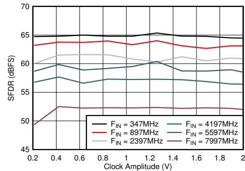
Figure 6-82. DES Mode: SFDR vs Clock Amplitude
