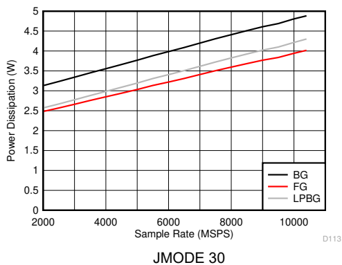
Figure 6-143. DES Mode: Power Dissipation vs Sample Rate
