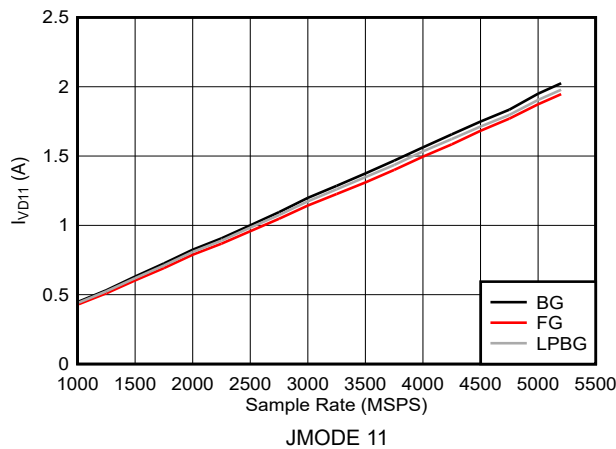
Figure 6-151. Dual Channel Mode: I_{VD11} vs Sample Rate (ADC12DJ5210RF)
