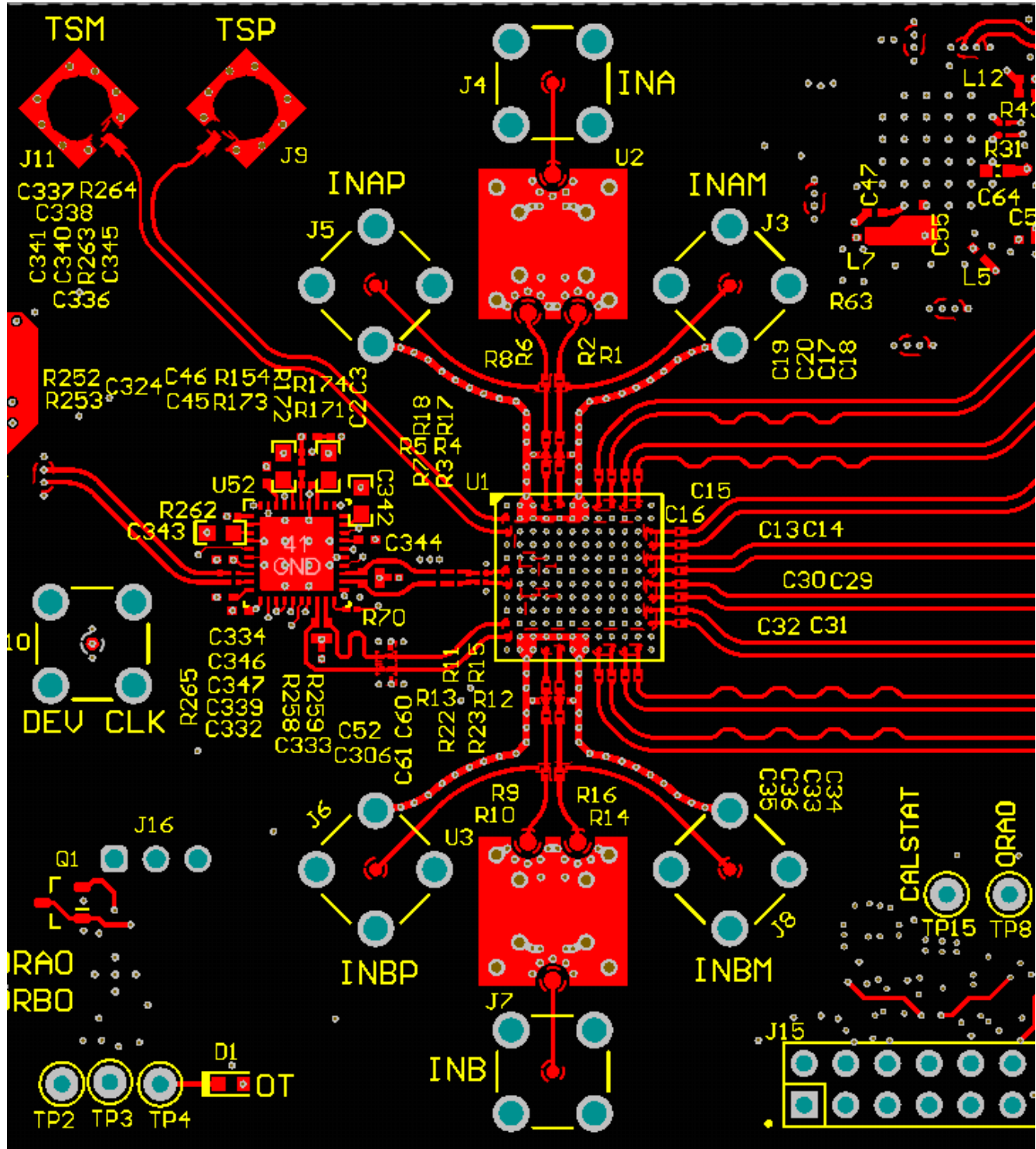
Figure 8-17. Top Layer Routing: Analog Inputs, CLK and SYSREF, DA0-3, DB0-3
