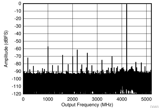
Figure 6-8. DES Mode: Single Tone FFT at 4197 MHz
