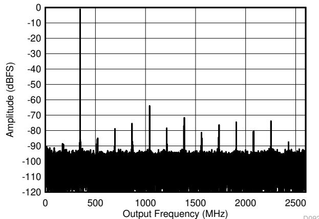
Figure 6-17. Dual Channel Mode: Single Tone FFT at 347 MHz
