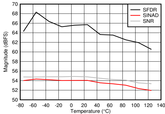
Figure 6-89. Dual Channel Mode: SNR, SINAD and SFDR vs Temperature
