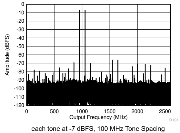
Figure 6-26. Dual Channel Mode: Two Tone FFT at 4197 MHz
