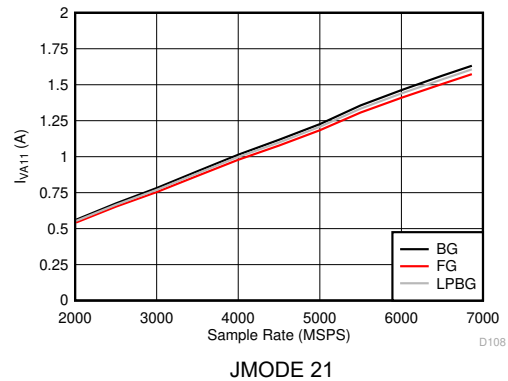
Figure 6-132. DES Mode: I_{VD11} vs Sample Rate (ADC12DJ5200RF)
