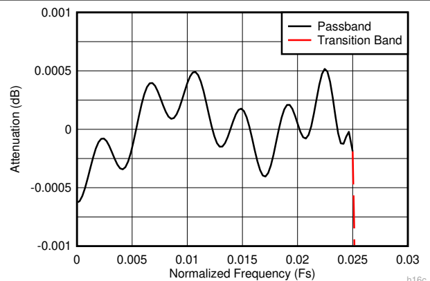
Figure 7-16. Decimate-by-16 Composite Zoomed Pass-Band Response
