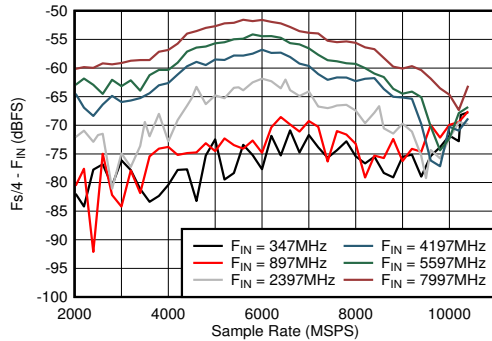
Figure 6-43. DES Mode: F_s/4 - F_{\text{IN}} vs Sample Rate and Input Frequency
