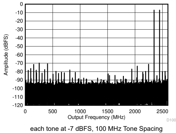
Figure 6-25. Dual Channel Mode: Two Tone FFT at 2397 MHz
