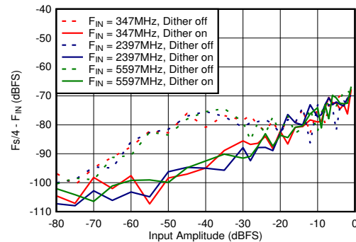
Figure 6-70. DES Mode: F_s/4 - F_{\text{IN}} vs Input Amplitude and Dither
