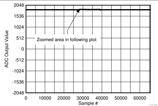
Figure 6-166. Background Calibration Core Transition (DC Signal)
