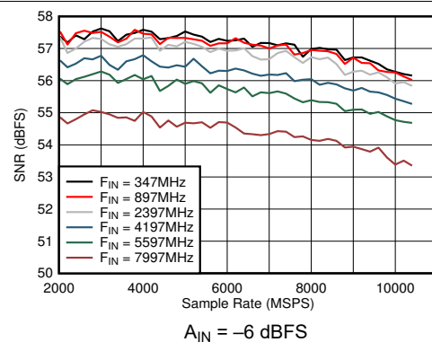
Figure 6-30. DES Mode: SNR vs Sample Rate and Input Frequency
