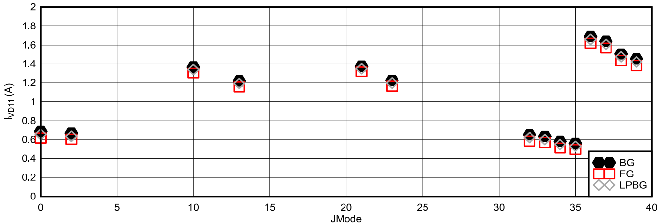
Figure 6-123. Other Modes with Lower Maximum F_S : I_{VD11} vs JMODE (ADC12DJ5200RF)
