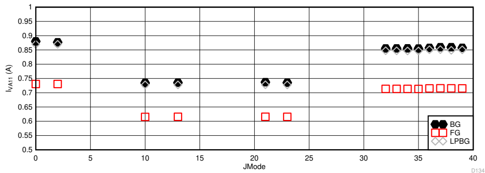
Figure 6-121. Other Modes with Lower Maximum F_S : I_{VA19} vs JMODE
