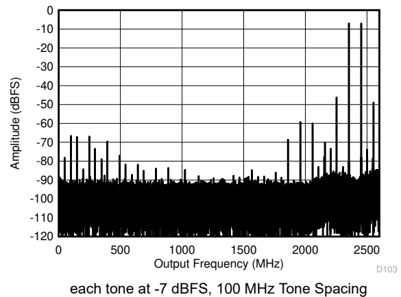
Figure 6-28. Dual Channel Mode: Two Tone FFT at 7997 MHz
