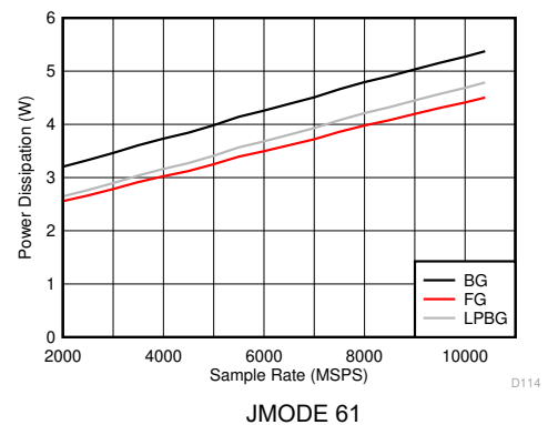
Figure 6-144. DES Mode: Power Dissipation vs Sample Rate
