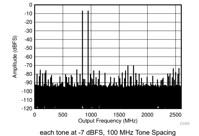
Figure 6-24. Dual Channel Mode: Two Tone FFT at 897 MHz
