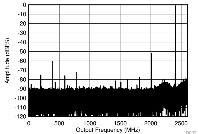
Figure 6-22. Dual Channel Mode: Single Tone FFT at 7997 MHz
