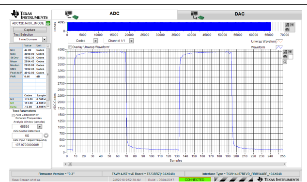
Figure 8-7. 40MHz, Square-Wave Time Domain for 5GSPS, Single-Channel Oscilloscope
