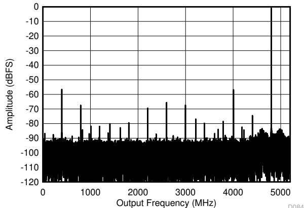
Figure 6-9. DES Mode: Single Tone FFT at 5597 MHz
