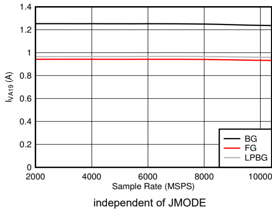
Figure 6-127. DES Mode: I_{VA19} vs Sample Rate
