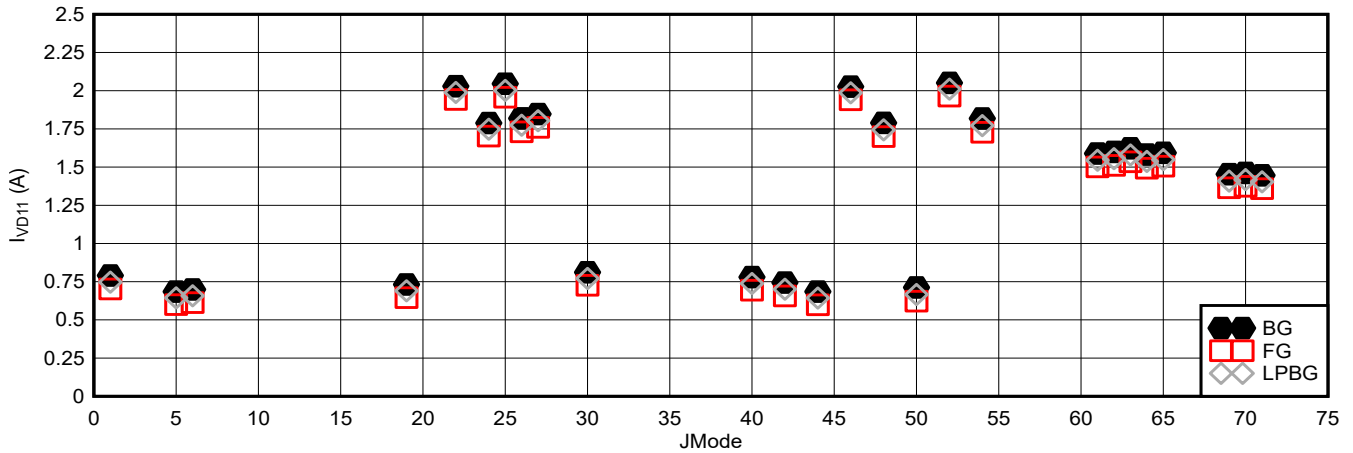
Figure 6-111. DES Mode: I_{VD11} vs JMODE at 10.4GSPS (ADC12DJ5200RF)
