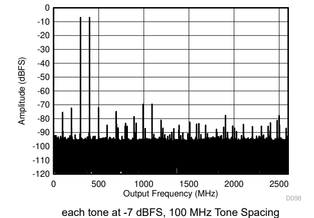
Figure 6-23. Dual Channel Mode: Two Tone FFT at 347 MHz
