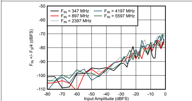
Figure 6-65. DES Mode: F_{IN} \pm F_{IN}/4 vs Input Amplitude and Frequency
