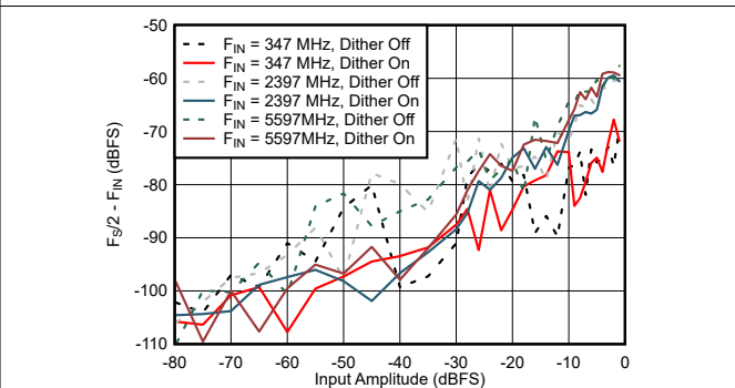
Figure 6-64. DES Mode: F_s/2 - F_{IN} vs Input Amplitude and Dither
