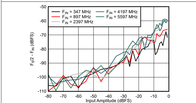
Figure 6-63. DES Mode: F_s/2 - F_{IN} vs Input Amplitude and Frequency
