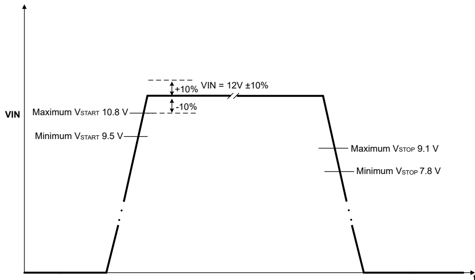
Figure 8-6. Start-Up and UVLO Values for Two-Resistor Configuration With VIN = 12 V
