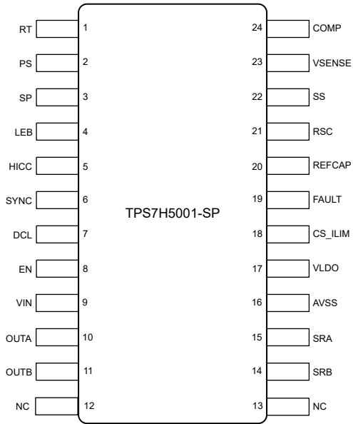
Figure 6-5. TPS7H5001-SP PW Package 24-Pin TSSOP (Top View)
