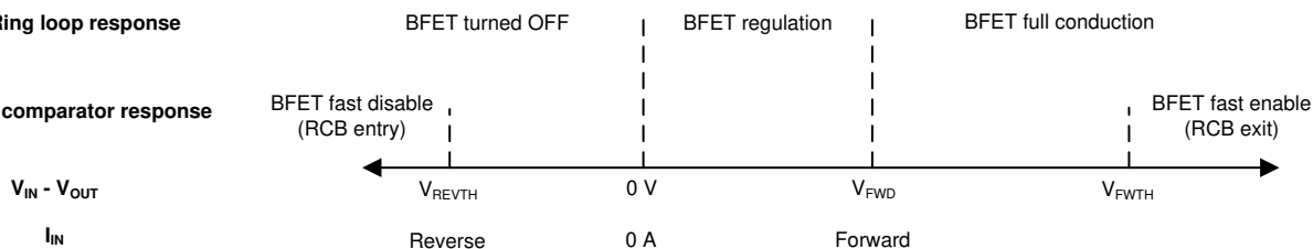
Figure 7-13. Reverse Current Blocking Response
