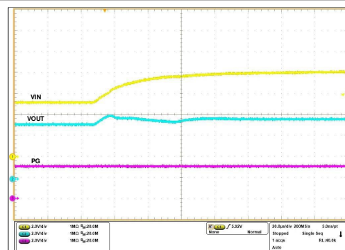
Figure 6-45. Overvoltage Lockout Response - TPS259470x/4x
