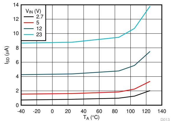
Figure 6-7. IN Shutdown Current vs Temperature
