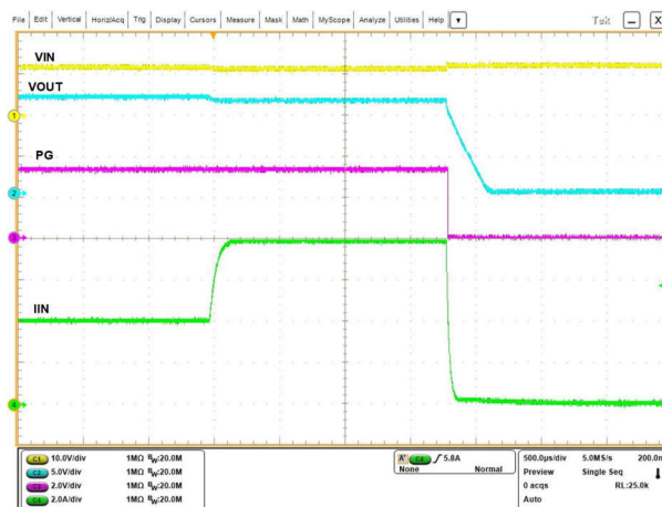
Figure 8-6. Circuit Breaker Response
