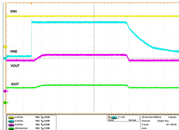
Figure 8-8. Active ORing Response
