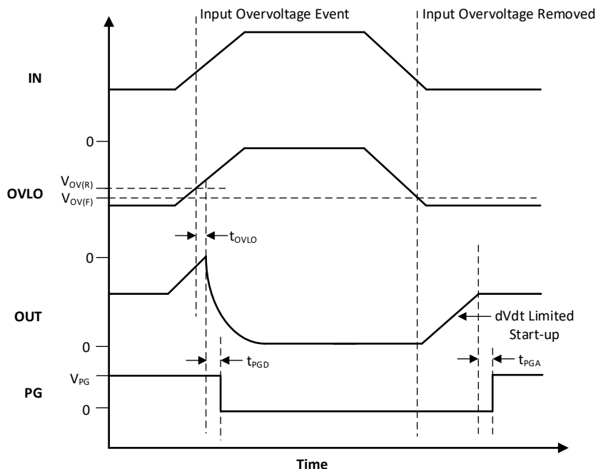
Figure 7-7. TPS25947x Overvoltage Lockout and Recovery
