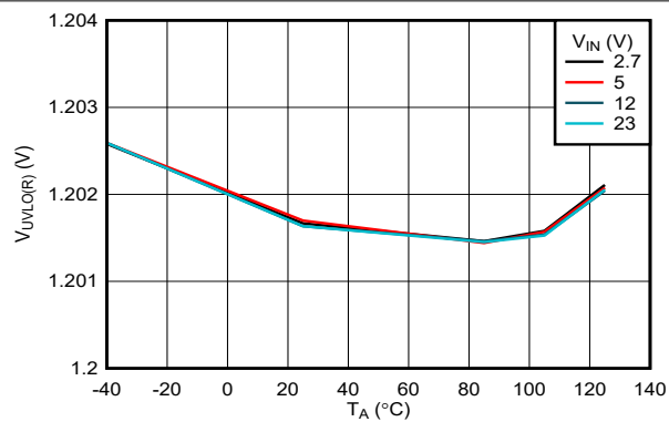
Figure 6-9. EN/UVLO Rising Threshold vs Temperature
