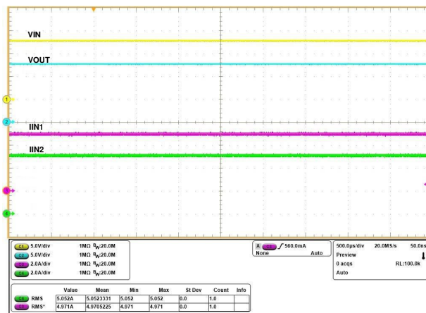
Figure 8-20. Parallel Devices Load Current During Steady State
