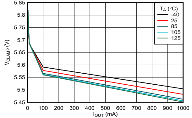
Figure 6-27. OVC Clamping Voltage (OVCSEL = Open) vs Load Current
