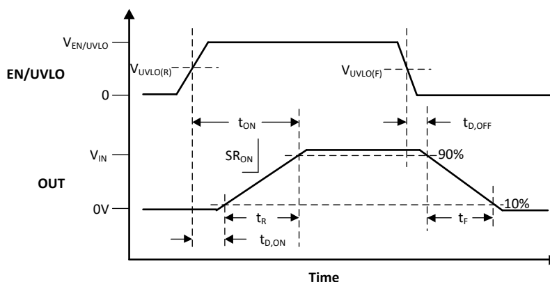
Figure 6-1. TPS25947xx Switching Times
