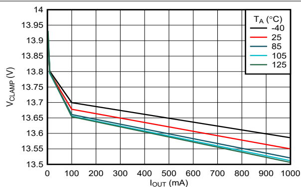
Figure 6-25. OVC Clamping Voltage (OVCSEL = 392kΩ to GND) vs Load Current
