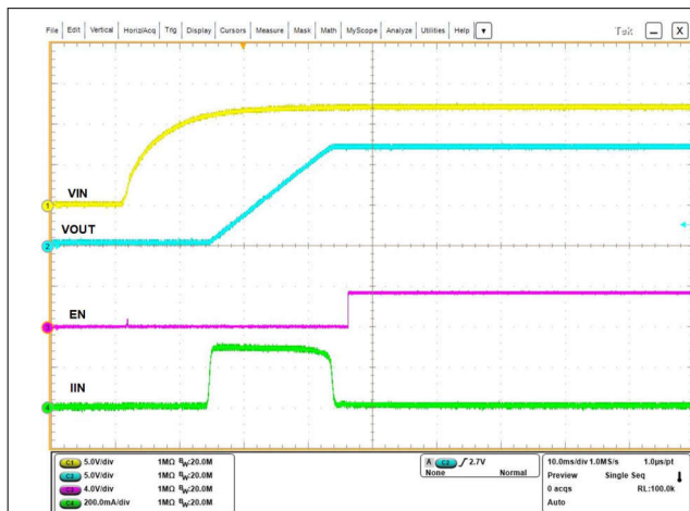
Figure 8-4. Power Up
