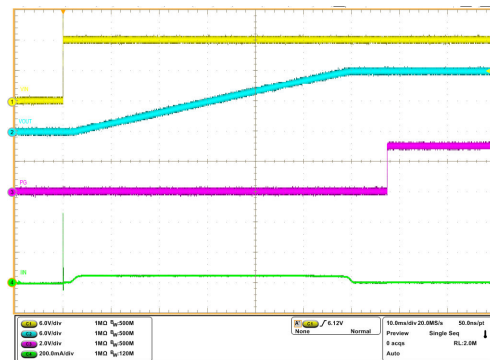
Figure 6-38. Start-Up with Enable
