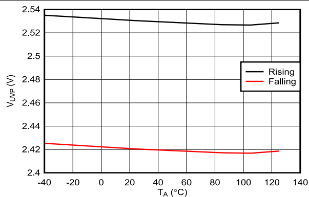
Figure 6-8. IN Undervoltage Threshold vs Temperature
