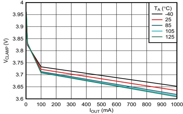
Figure 6-26. OVC Clamping Voltage (OVCSEL = GND) vs Load Current
