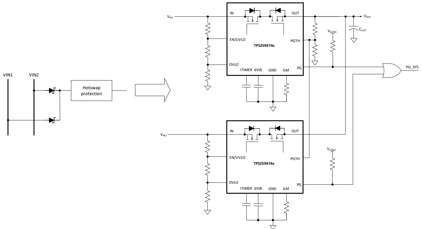
Figure 8-7. Two Devices, Active ORing Configuration
