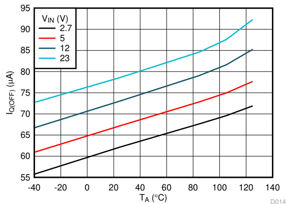
Figure 6-6. IN OFF State (UVLO) Current vs Temperature
