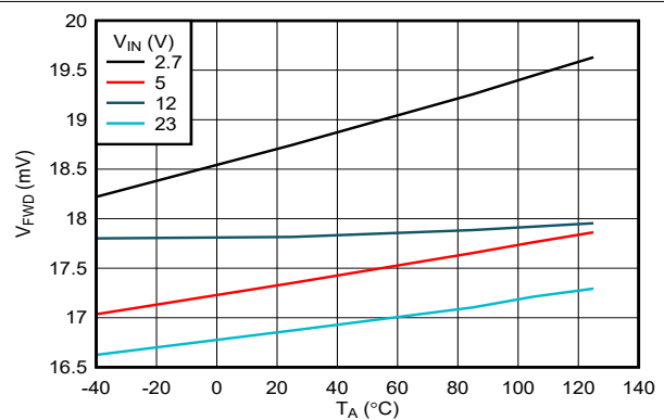
Figure 6-19. RCB - Forward Regulation Voltage vs Temperature
