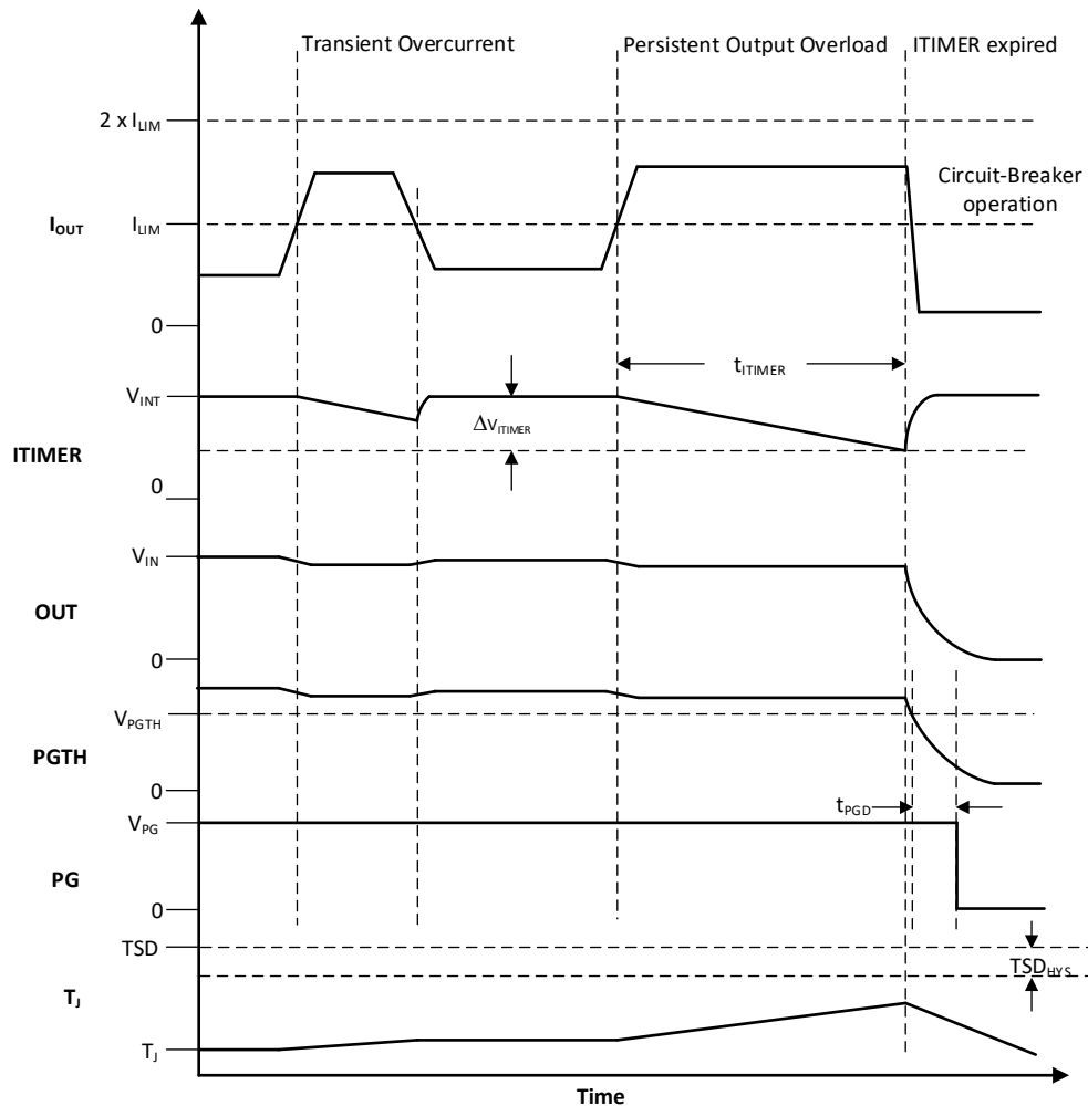
Figure 7-9. TPS25947x Overcurrent Response
