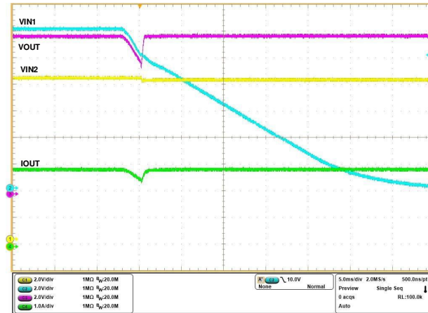
Figure 8-11. TPS259470x Power MUX - Switchover from Primary to Auxiliary Supply
