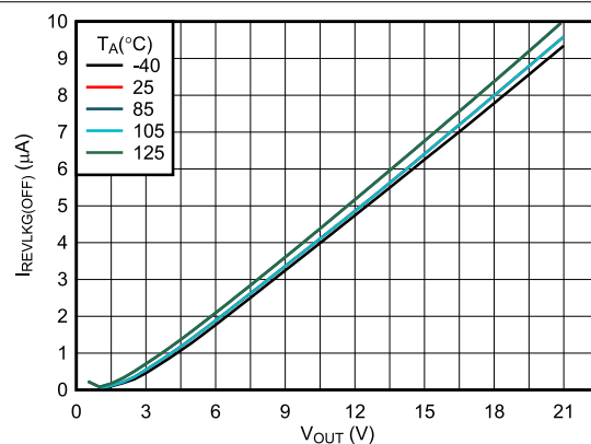
Figure 6-23. Reverse Leakage Current During OFF-State
