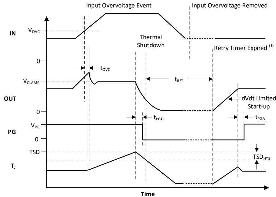
Figure 7-8. TPS25947x Overvoltage Response (Auto-Retry)
