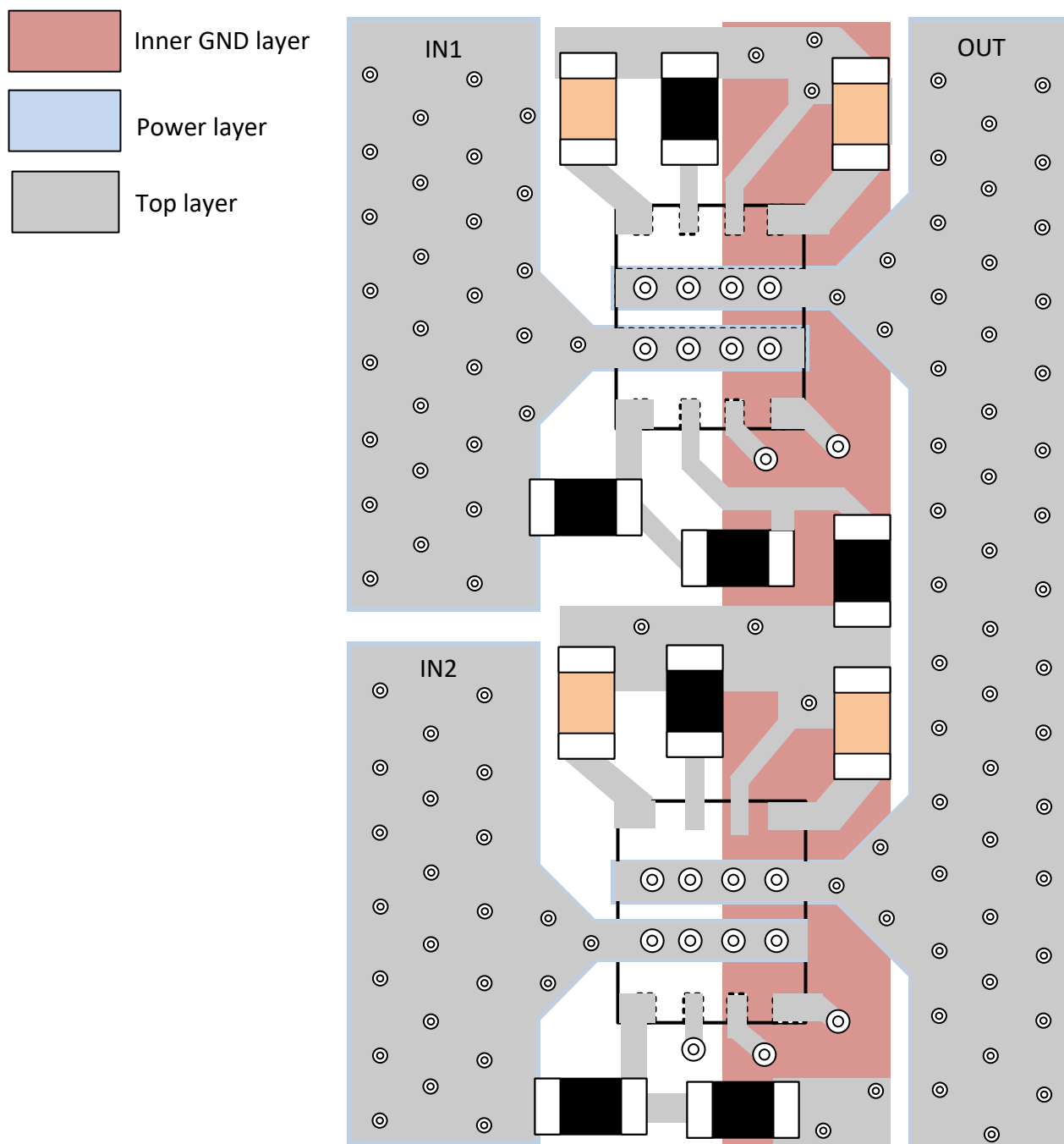
Figure 8-23. Layout Example - 2 × TPS259470x in PowerMUX Configuration
