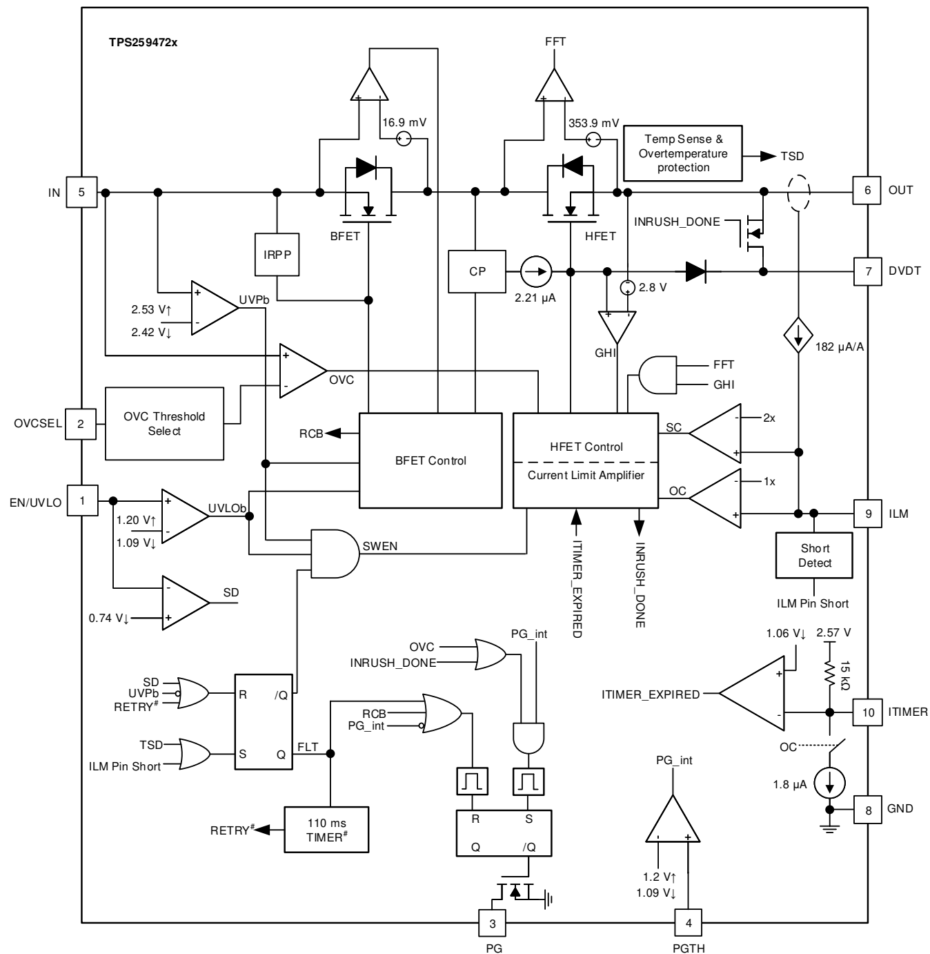
Figure 7-2. TPS259472x Block Diagram
