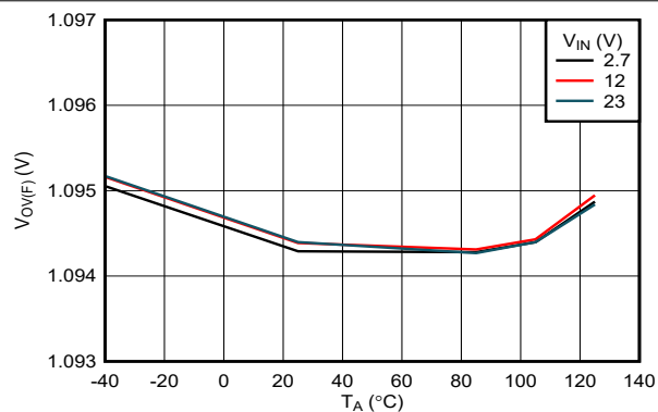
Figure 6-13. OVLO Falling Threshold vs Temperature
