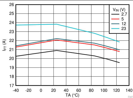
Figure 6-18. Steady State Fixed Fast-Trip Current Threshold vs Temperature
