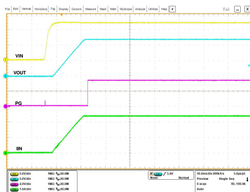
Figure 6-40. Input Hot-Plug
