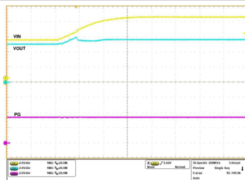
Figure 6-44. Input Reverse Polarity Protection - Slow Ramp
