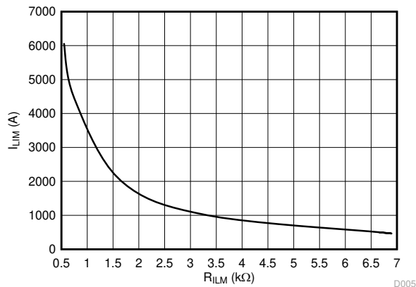
Figure 6-14. Overcurrent Threshold vs ILM Resistor
