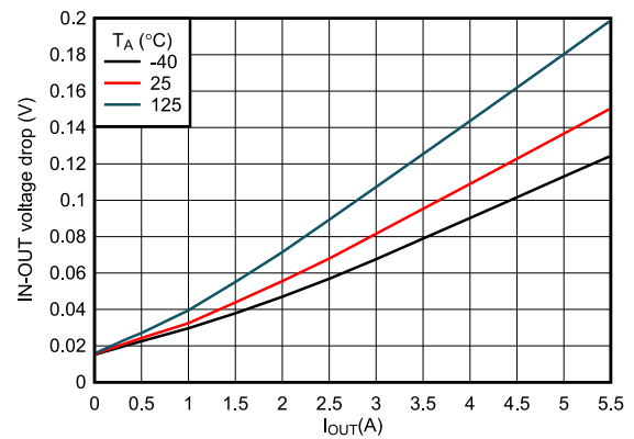
Figure 6-3. Forward Voltage Drop vs Load Current
