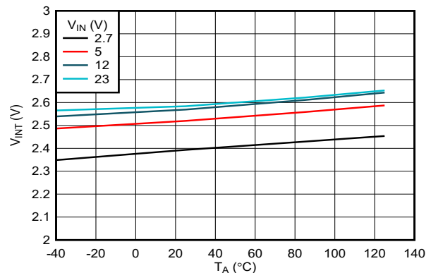
Figure 6-31. ITIMER Internal Pullup Voltage vs Temperature
