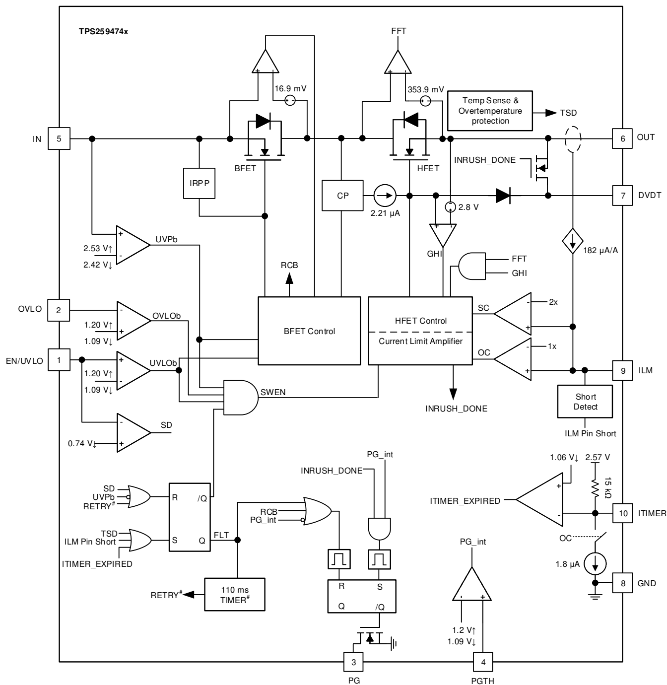
Figure 7-3. TPS25947x Block Diagram
