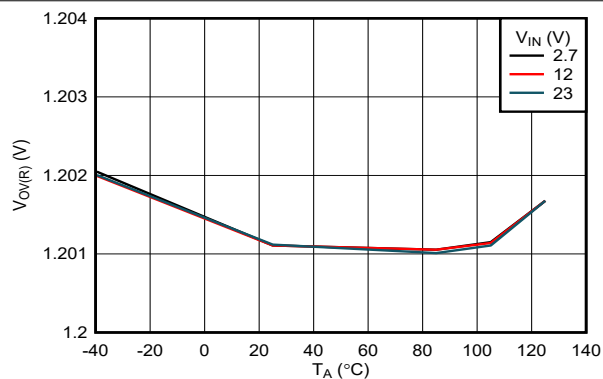
Figure 6-12. OVLO Rising Threshold vs Temperature
