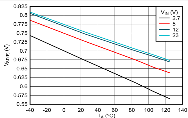
Figure 6-11. EN/UVLO Shutdown Falling Threshold vs Temperature
