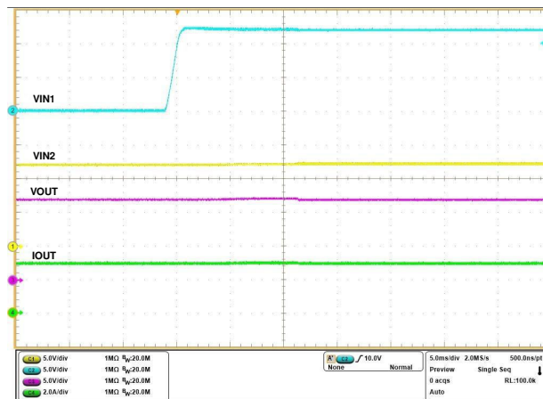
Figure 8-12. TPS259470x Power MUX - Switchover from Auxiliary to Primary Supply
