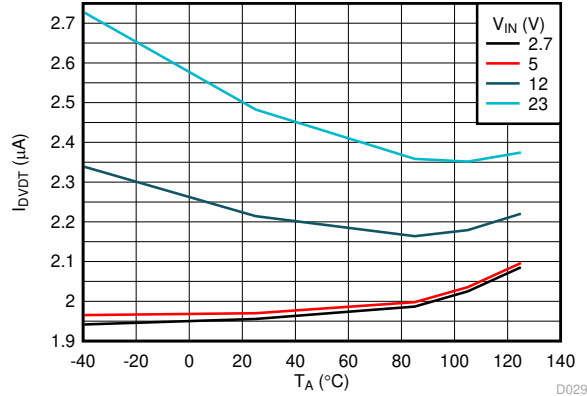
Figure 6-32. DVDT Charging Current vs Temperature
