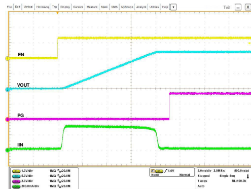
Figure 6-39. Start-Up with Supply
