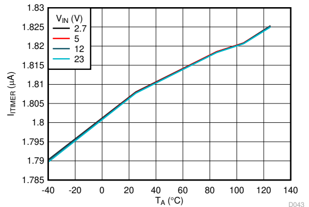
Figure 6-29. ITIMER Discharge Current vs Temperature
