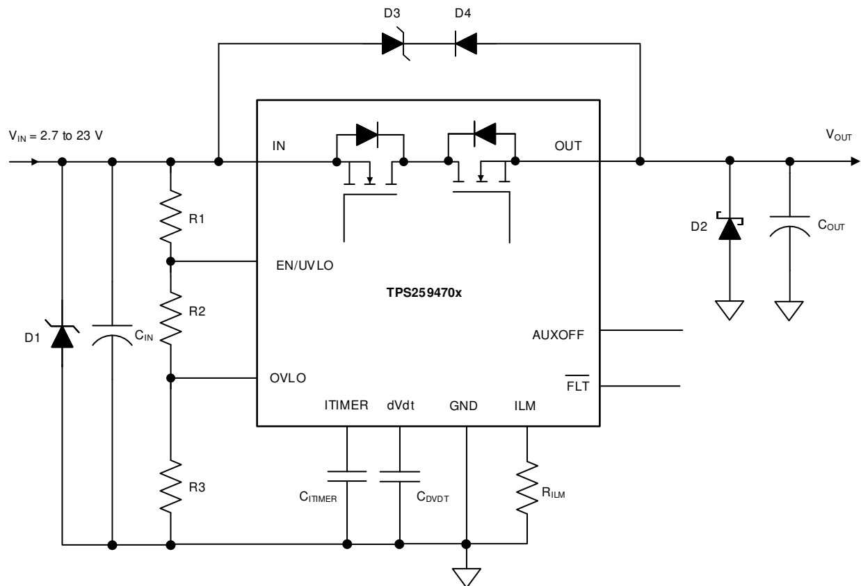
Figure 8-21. Circuit Implementation with Optional Protection Components
