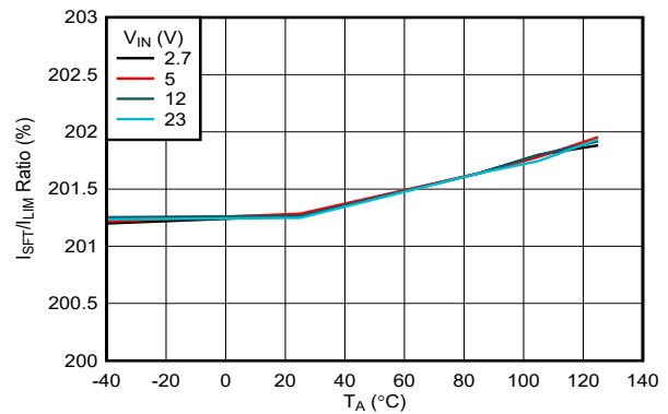
Figure 6-17. Scalable Fast-Trip Threshold: Current Limit Threshold ( I_{LIM} ) Ratio vs Temperature
