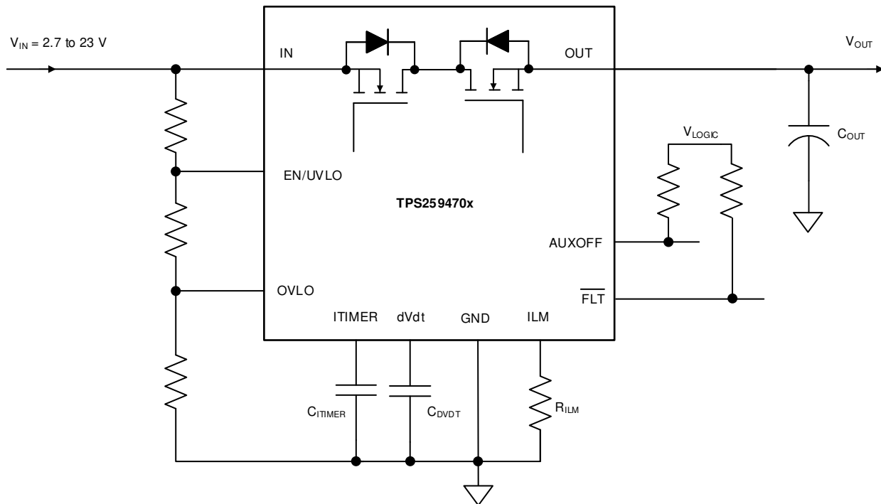
Simplified Schematic
