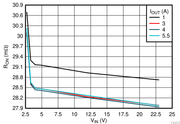
Figure 6-2. ON-Resistance vs Supply Voltage
