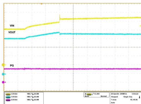
Figure 6-46. Overvoltage Clamp Response - TPS259472x
