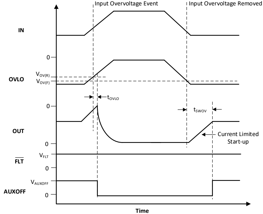
Figure 7-6. TPS259470x Overvoltage Lockout and Recovery
