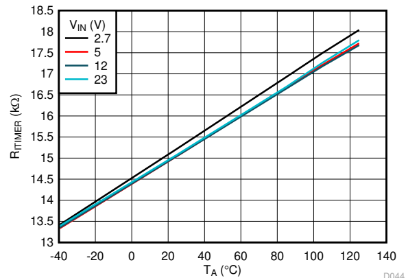
Figure 6-30. ITIMER Internal Pullup Resistance vs Temperature
