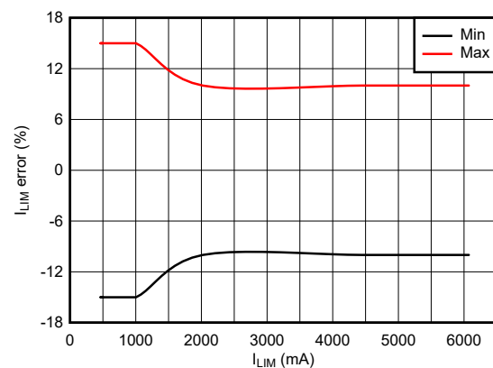
Figure 6-15. Overcurrent Threshold Accuracy (Across Process, Voltage and Temperature)
