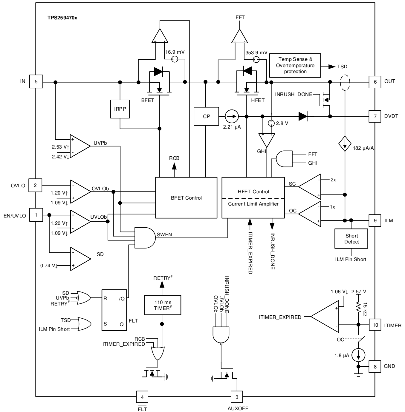
Figure 7-1. TPS259470x Block Diagram
