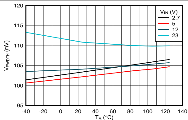
Figure 6-21. RCB - Forward Comparator Threshold vs Temperature
