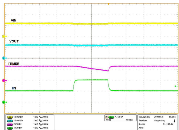
Figure 8-5. Transient Overload
