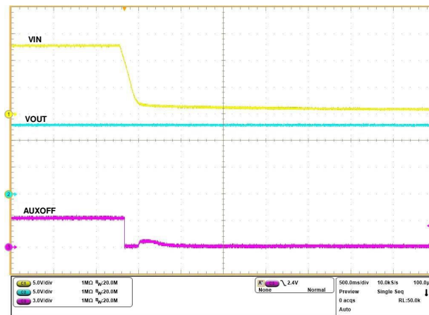
Figure 7-16. Reverse Current Blocking Performance During Input Supply Failure
