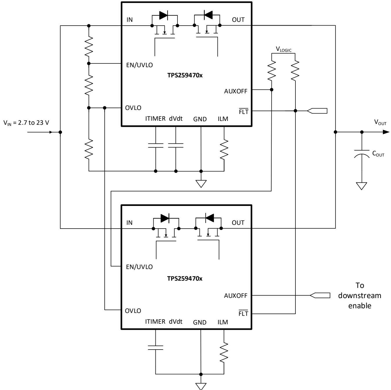
Figure 8-18. Two Devices Connected in Parallel for Higher Steady State Current Capability
