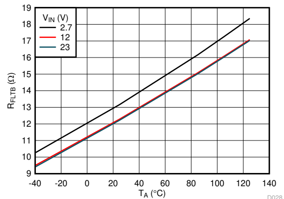
Figure 6-35. FLTB Pin Pulldown Resistance vs Temperature
