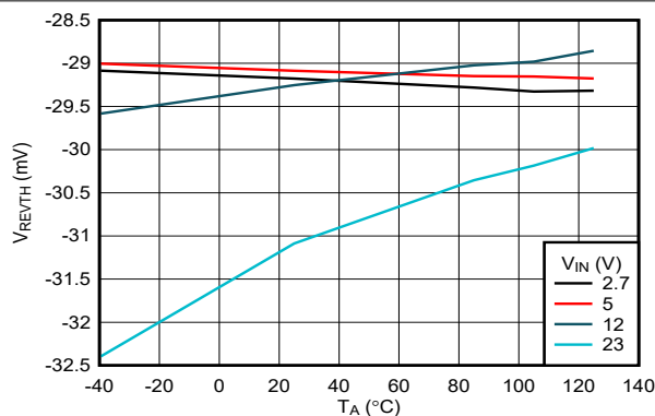
Figure 6-20. RCB - Reverse Comparator Threshold vs Temperature
