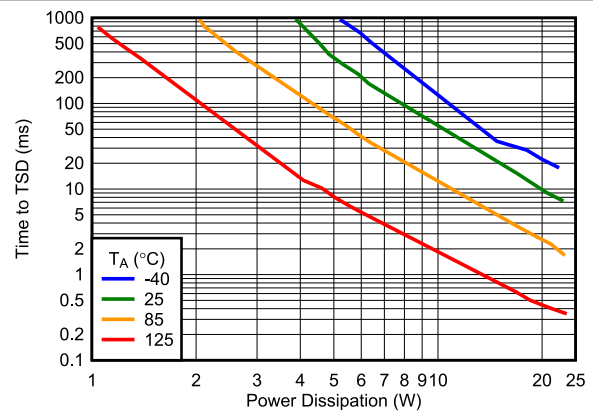
Figure 6-37. Time to Thermal Shut-Down During Steady State
