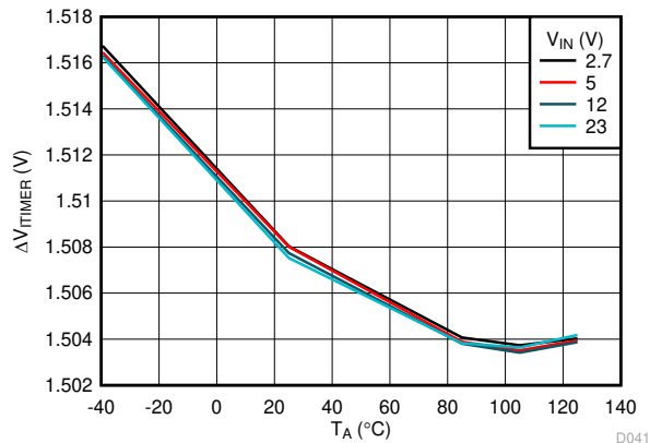
Figure 6-28. ITIMER Discharge Differential Voltage Threshold vs Temperature
