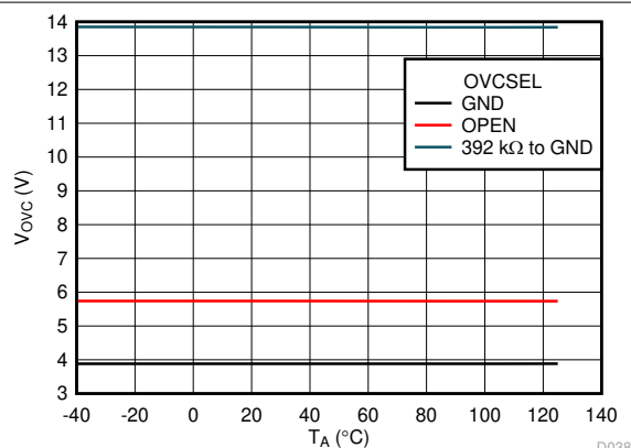
Figure 6-24. OVC Threshold vs Temperature
