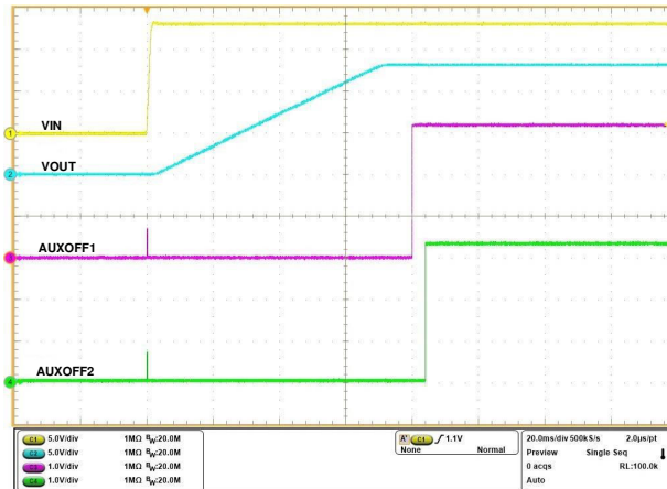
Figure 8-19. Parallel Devices Sequencing During Start-Up
