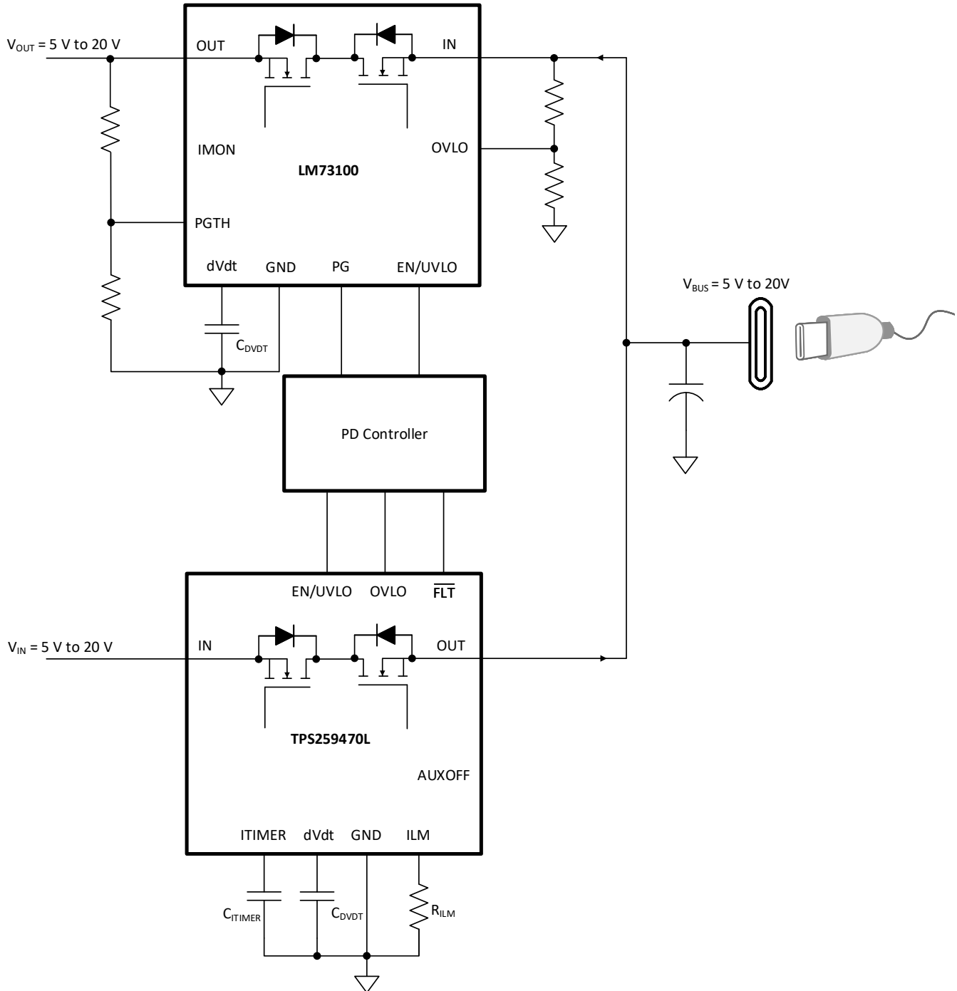
Figure 8-16. USB PD Port Protection
