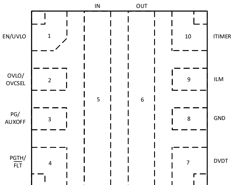
Figure 5-1. TPS25947xx RPW Package 10-Pin QFN Top View
