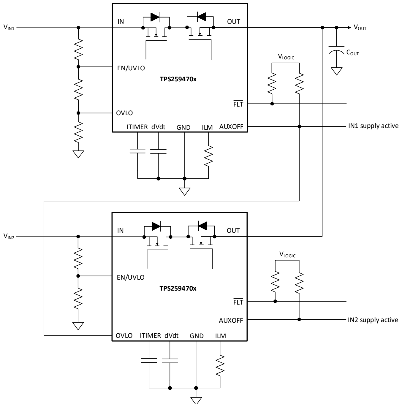
Figure 8-10. Priority Power MUXing with 2 × TPS259470x - Option 1
