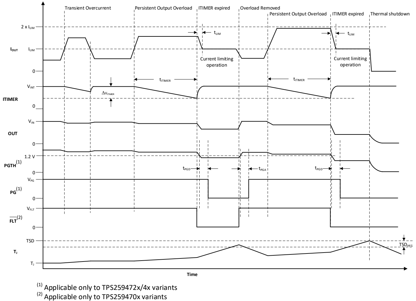
Figure 7-10. TPS259470x/2x Active Current Limit Response
