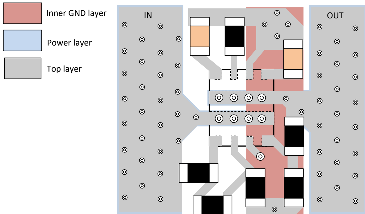
Figure 8-22. Layout Example - Single TPS25947x with PGTH Referred to OUT
