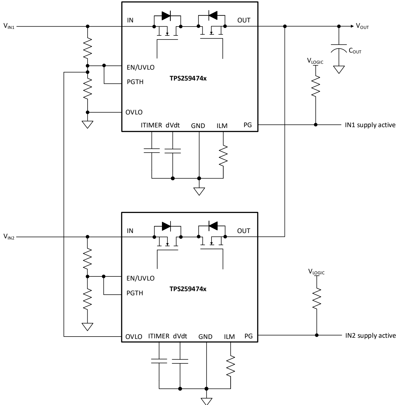
Figure 8-15. Priority power MUXing with 2 × TPS25947x
