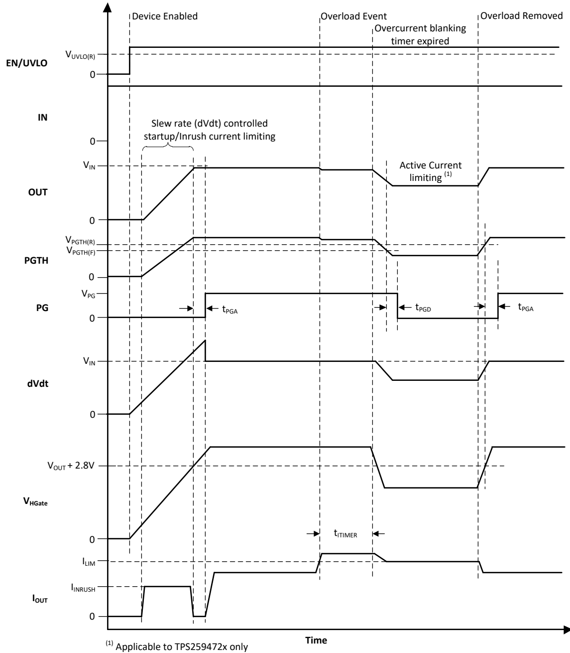
Figure 7-17. TPS259472x, TPS259474x PG Timing Diagram
