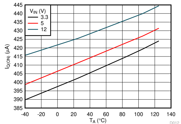
Figure 6-5. IN Quiescent Current vs Temperature (TPS259472x Variant)
