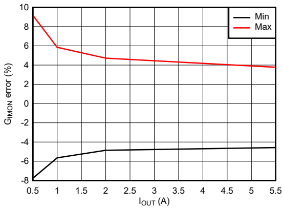
Figure 6-16. Analog Current Monitor Gain Accuracy
