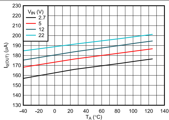
Figure 6-22. OUT Leakage Current During ON-State Reverse Current Blocking
