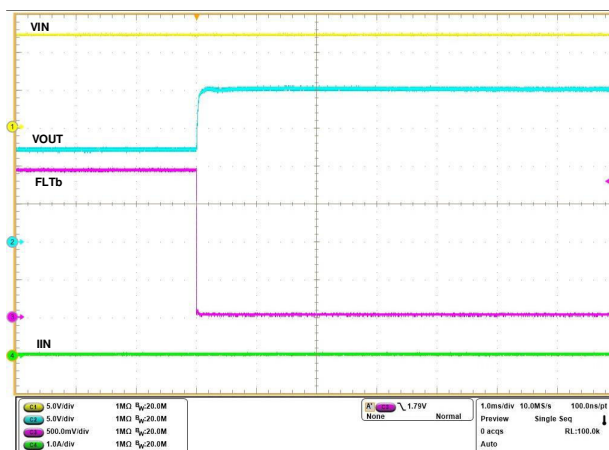
Figure 7-14. Reverse Current Blocking Performance During Fast Voltage Step at Output
