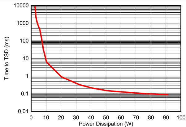
Figure 6-36. Time to Thermal Shut-Down During Inrush State
