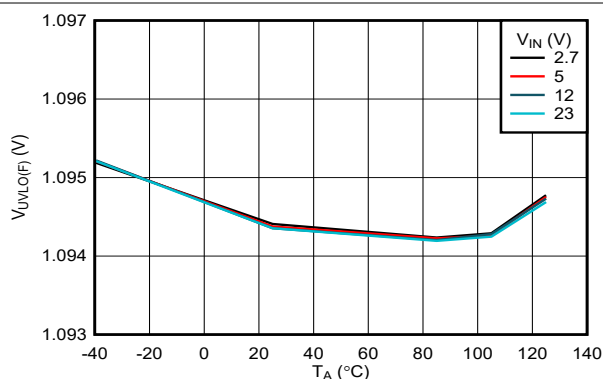
Figure 6-10. EN/UVLO Falling Threshold vs Temperature
