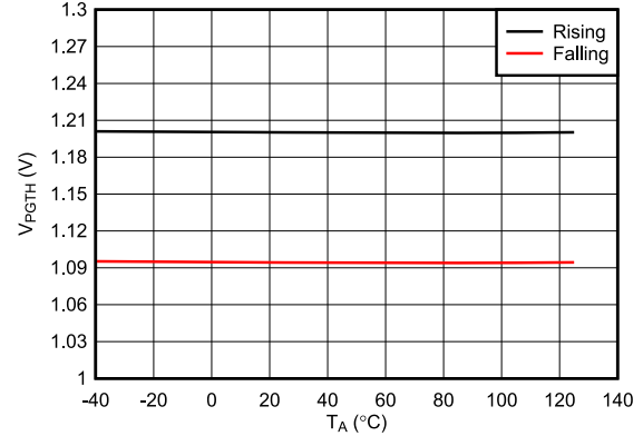
Figure 6-33. PGTH Threshold vs Temperature
