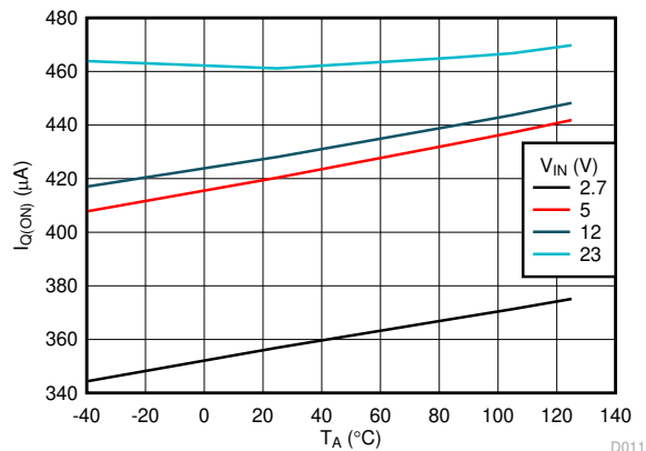
Figure 6-4. IN Quiescent Current vs Temperature (TPS259470x, TPS2594704x Variants)
