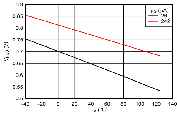
Figure 6-34. PG Low Voltage Without Input Supply vs Temperature
