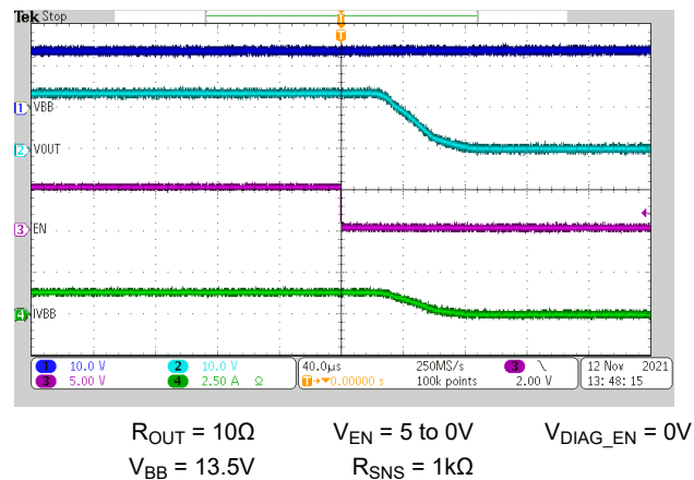
Figure 5-21. Turn-off Time ( t_{OFF} )
