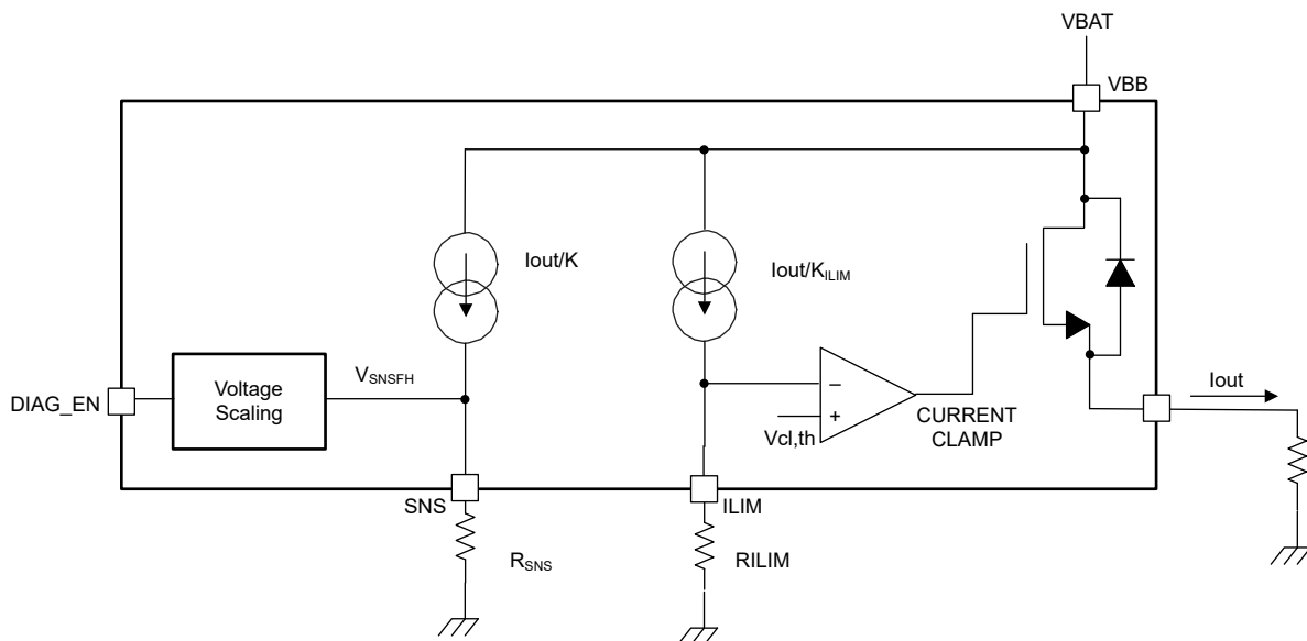
Figure 7-3. Current-Sense and Current-Limit Block Diagram
