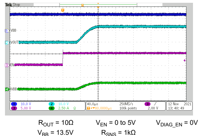
Figure 5-20. Turn-on Time ( t_{ON} )
