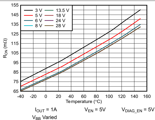
Figure 5-6. R_{DS(on)} vs Temperature
