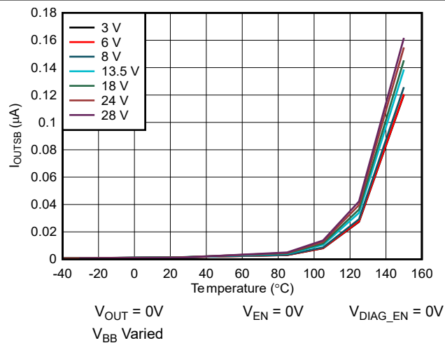
Figure 5-3. Output Leakage Current I_{OUT,STBY} vs Temperature
