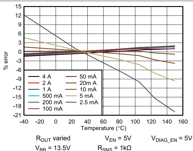
Figure 5-10. K_{SNS} Error vs Temperature
