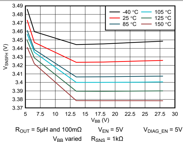
Figure 5-12. V_{SNSFH} (3.3V) vs V_{BB}
