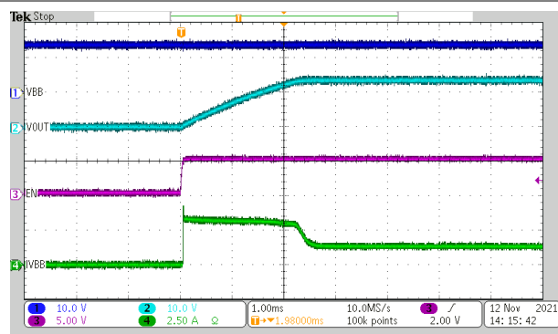
Figure 5-23. Short Circuit With ILIM Shorted to Ground
