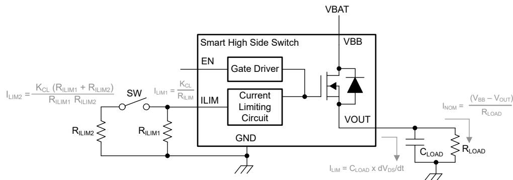
Figure 8-2. Dynamic Changing Current Limit Setup
