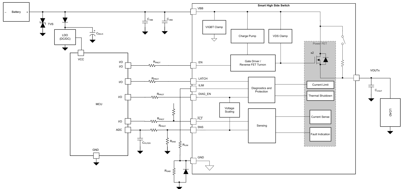
Figure 8-1. Typical Application Circuitry
