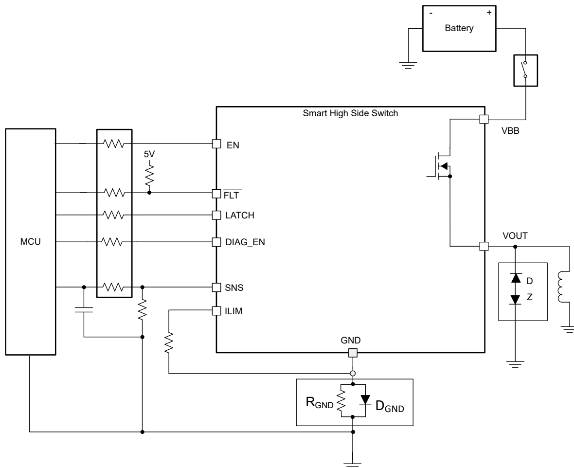
Figure 7-19. Loss of Battery
