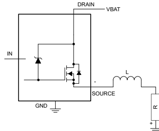
Figure 7-7. Driving Inductive Load
