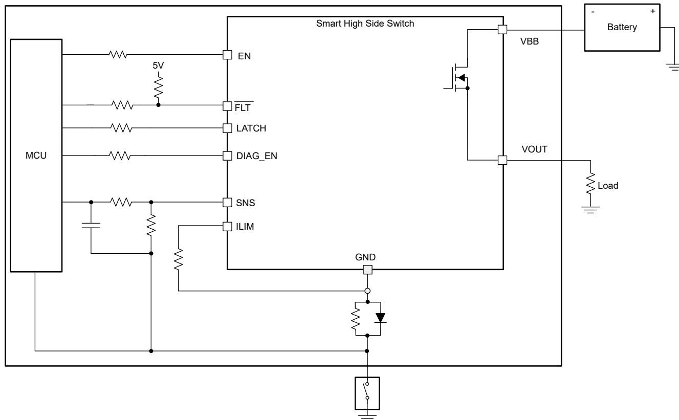
Figure 7-18. Loss of Module GND
