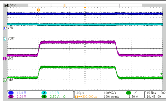
Figure 8-7. Load Step
