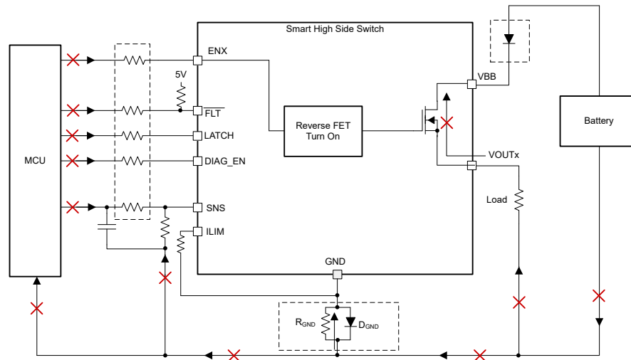
Figure 7-20. Reverse Protection With Block Diode
