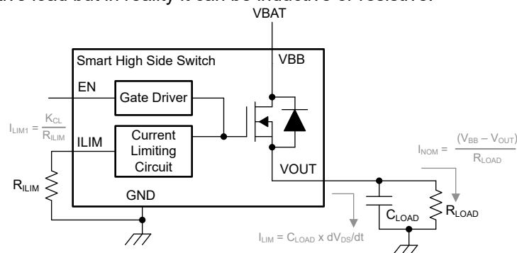
Figure 7-5. Capacitive Charging Circuit
