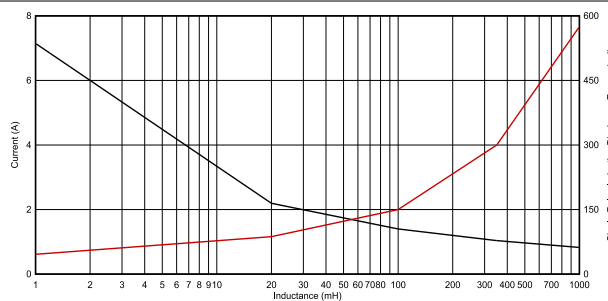
Figure 5-26. Inductive Load Discharge Energy Capability ( T_A = 125^\circ C )
