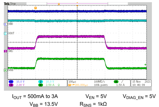
Figure 5-22. I_{SNS} Settling Time ( t_{SNSION} ) on Load Step
