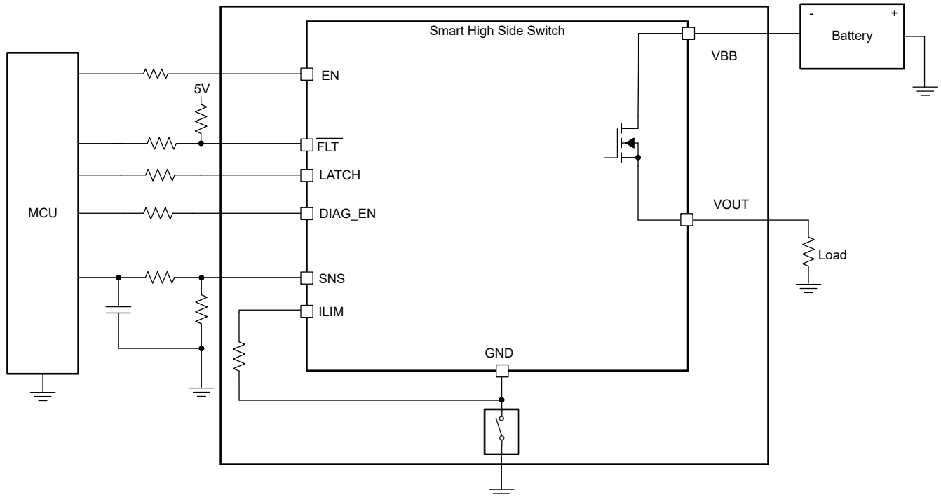
Figure 7-17. Loss of Device GND
