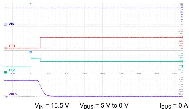
Figure 9-13. Type-C Detach
