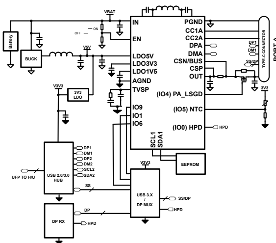
Figure 9-2. Simplified Single USB PD Charger with DisplayPort Alt Mode - MUX control with GPIO
