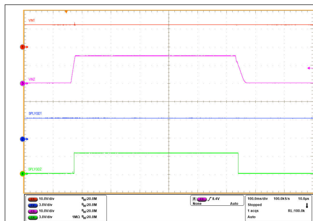
Figure 8-14. Active ORing Response
