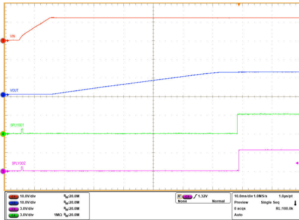
Figure 8-22. Parallel Devices Sequencing During Start-Up
