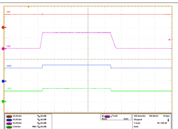
Figure 8-15. Active ORing Response
