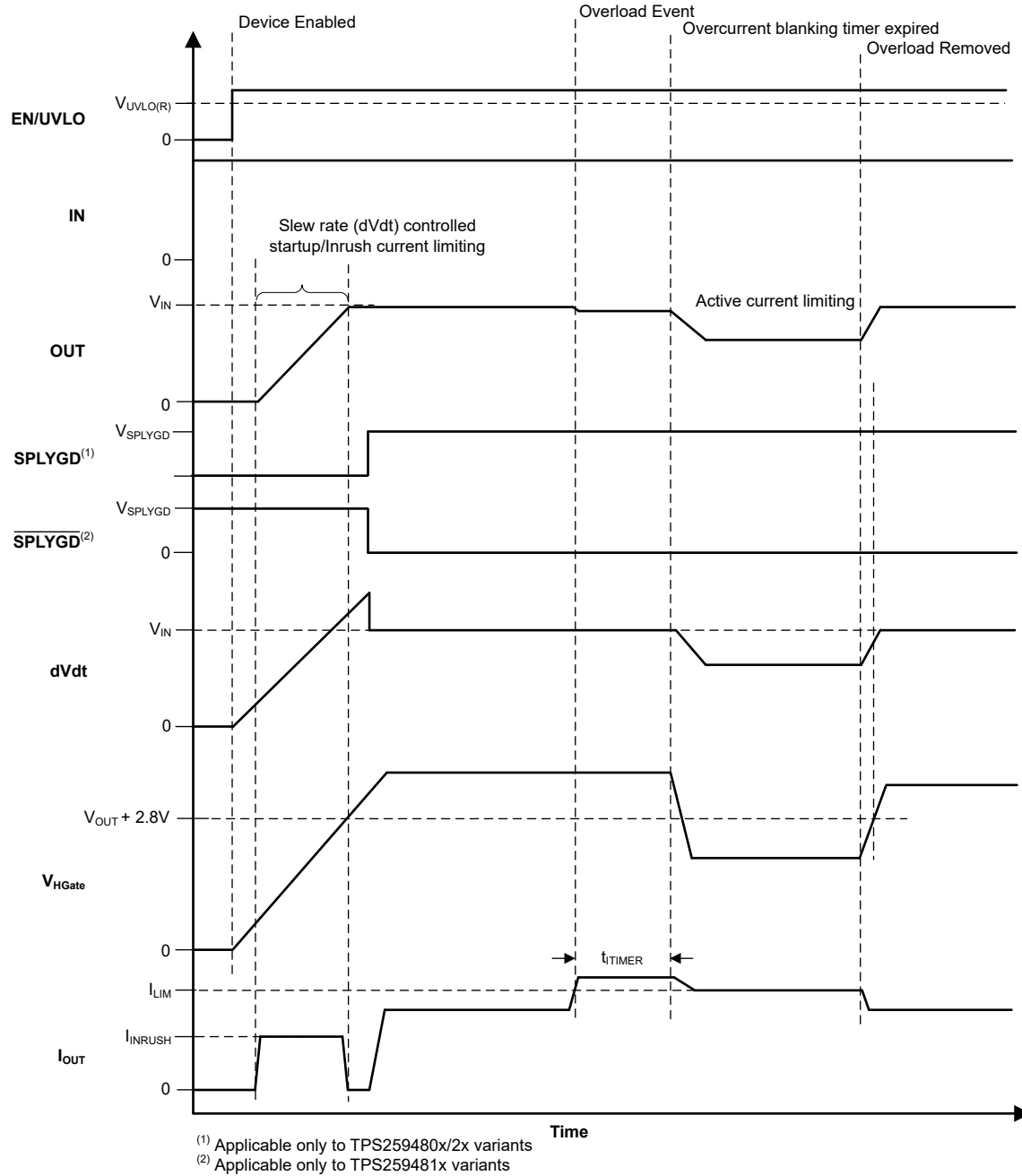
Figure 7-16. TPS25948xx SPLYGD Behavior
