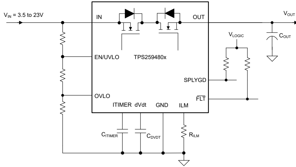
Simplified Schematic
