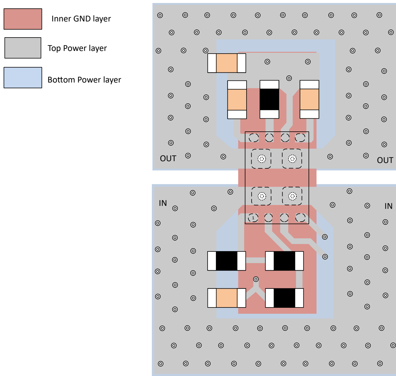
Figure 8-26. Layout Example
