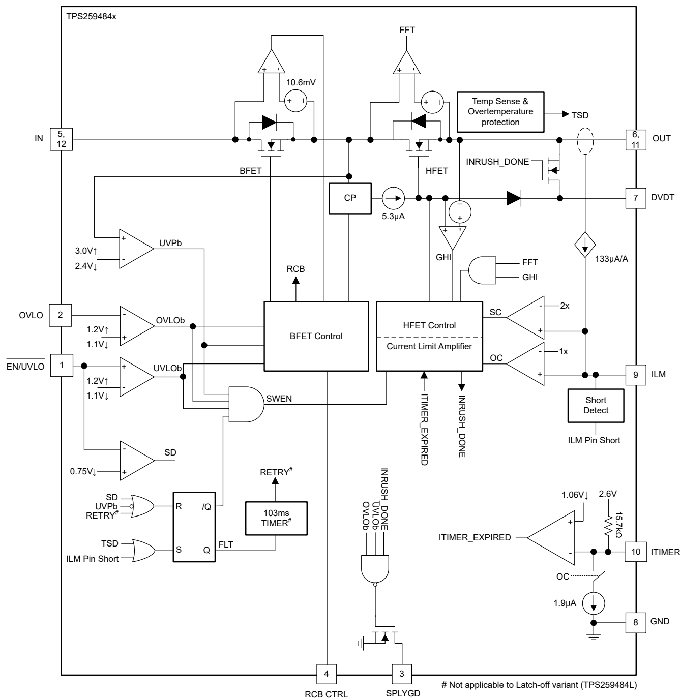
Figure 7-4. TPS25948 Block Diagram
