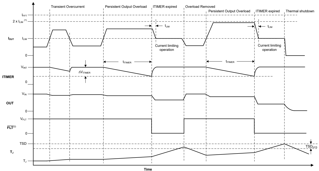
Figure 7-8. TPS25948xx Active Current Limit Response
