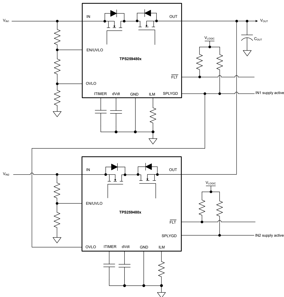
Figure 8-16. Priority Power MUXing With 2 × TPS259480x - Option 1
