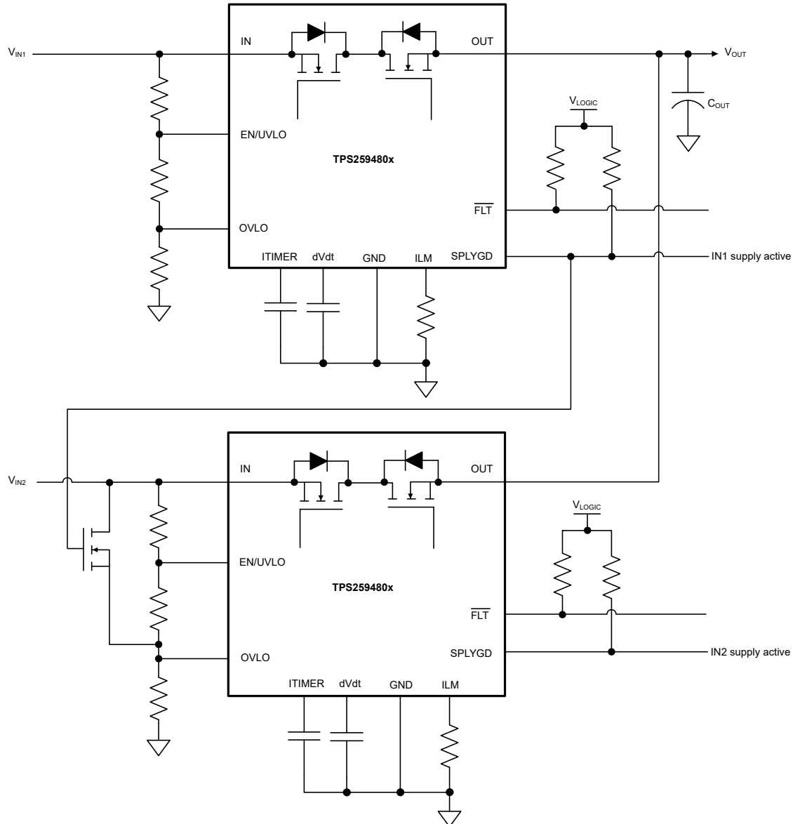
Figure 8-19. Priority Power MUXing With 2 × TPS259480x - Option 2
