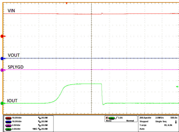
Figure 8-11. Wake up into Short Protection
