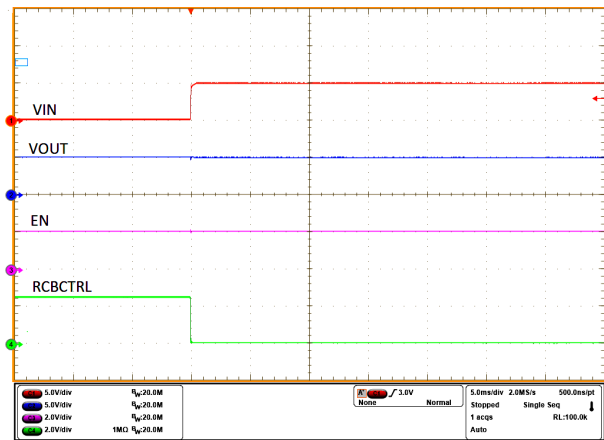
Figure 8-12. Power Up in OTG Mode
